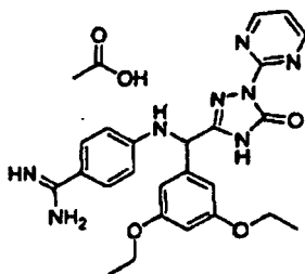
[Chemical Formula 250]
