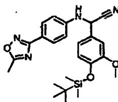
[Chemical Formula 102]
