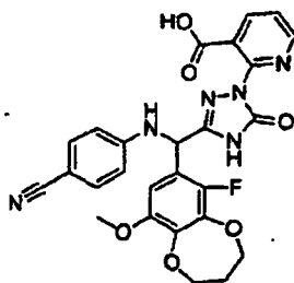
[Chemical Formula 450]
