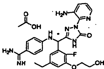
[Chemical Formula 790]
