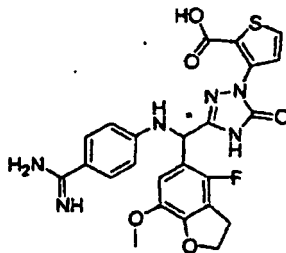
[Chemical Formula 546]
