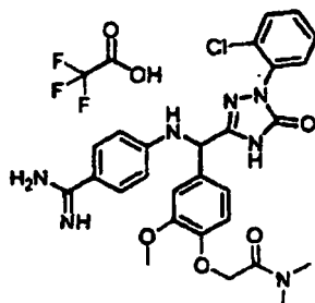
[Chemical Formula 750]
