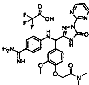
[Chemical Formula 632]
