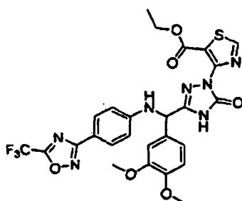
[Chemical Formula 506]
