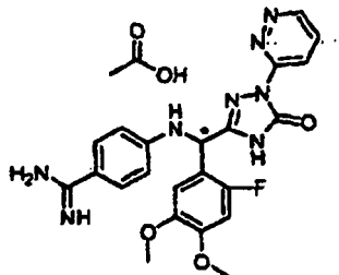
[Chemical Formula 318]
