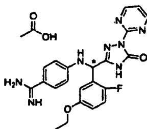
[Chemical Formula 280]
