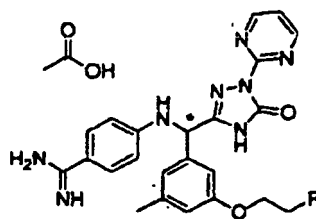
[1474] [Chemical Formula 625]
