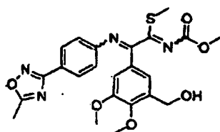
[Chemical Formula 128]
