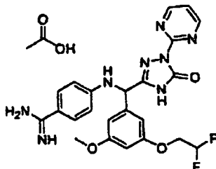
[Chemical Formula 736]
