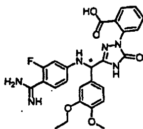
[Chemical Formula 792]
