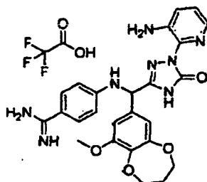
[Chemical Formula 163]
