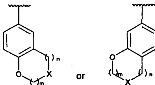
[Chemical Formula 11]
