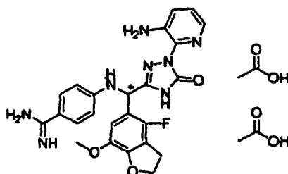
[Chemical Formula 211]
