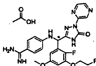
[Chemical Formula 289]
