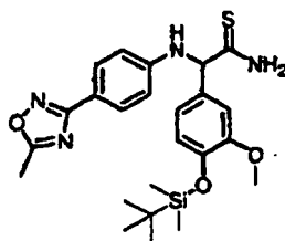
[Chemical Formula 103]
