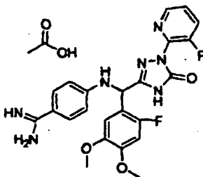
[Chemical Formula 327]
