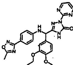
[Chemical Formula 99]
