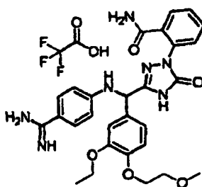
[Chemical Formula 738]
