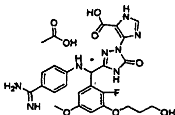
[Chemical Formula 782]
