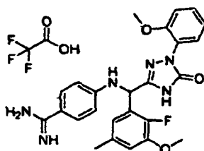
{Chemical Formula 89}
