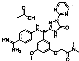
[Chemical Formula 222]
