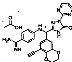
[Chemical Formula 820]
