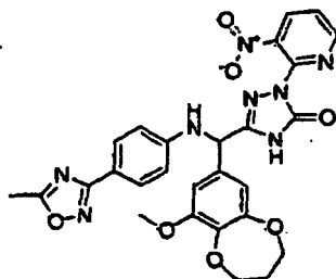
[Chemical Formula 162]
