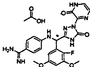
[Chemical Formula 394]
