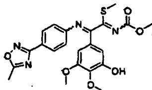
[Chemical Formula 268]
