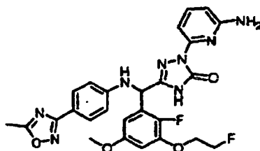
[Chemical Formula 209]
