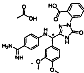
[Chemical Formula 172]
