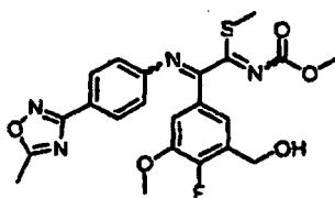
[Chemical Formula 342]
