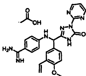
[Chemical Formula 737]
