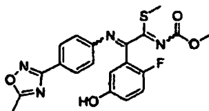
[Chemical Formula 279]
