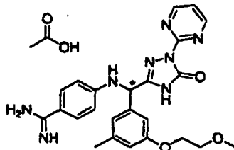
[Chemical Formula 277]
