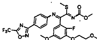
[Chemical Formula 529]
