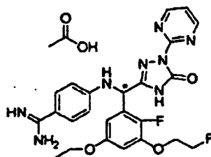
[Chemical Formula 232]
