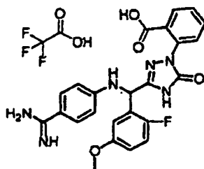
[Chemical Formula 637]
