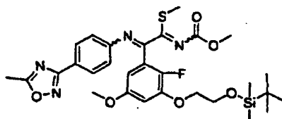
[Chemical Formula 524]
