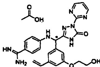
[Chemical Formula 199]
