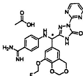
[Chemical Formula 631]
