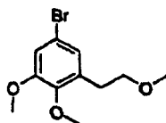
[Chemical Formula 334]
