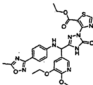
[Chemical Formula 480]
