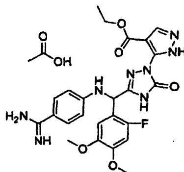
[Chemical Formula 400]
