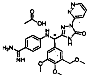
[Chemical Formula 656]
