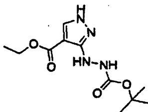
[Chemical Formula 397]
