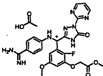
[Chemical Formula 793]
