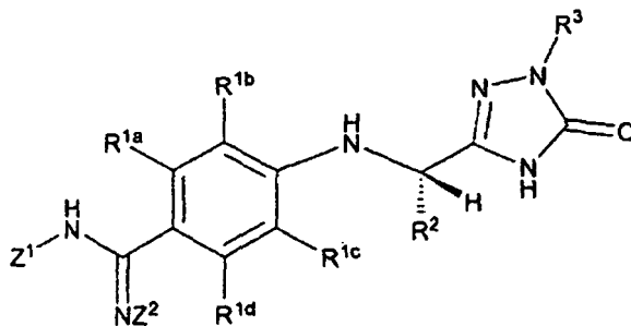
[Chemical Formula 3]
