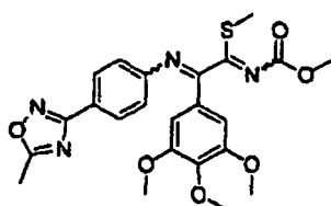
[Chemical Formula 570]
