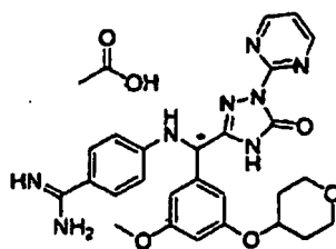
[Chemical Formula 223]
