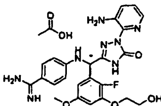
[Chemical Formula 527]
