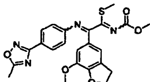
[Chemical Formula 151]
