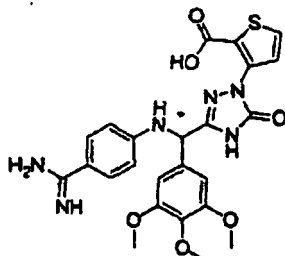
[Chemical Formula 571]
