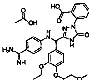
[Chemical Formula 721]
