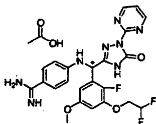
[Chemical Formula 288]
