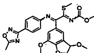
[Chemical Formula 256]
