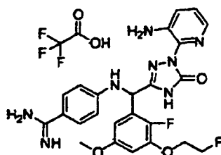
[Chemical Formula 359]
