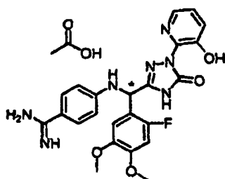
[Chemical Formula 657]
