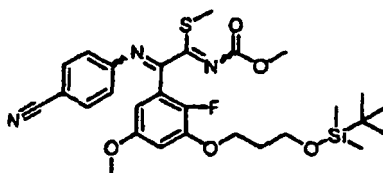
[Chemical Formula 416]
