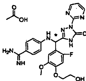
[Chemical Formula 584]
