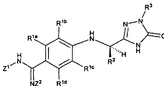
[Chemical Formula 2]
