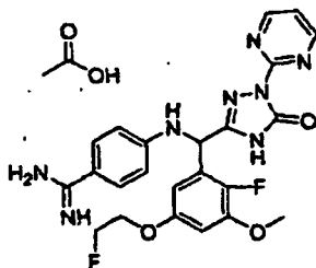
[Chemical Formula 734]
