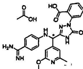
[Chemical Formula 176]
