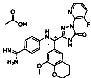
[Chemical Formula 146]
