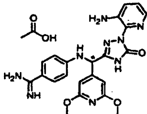
[Chemical Formula 215]
