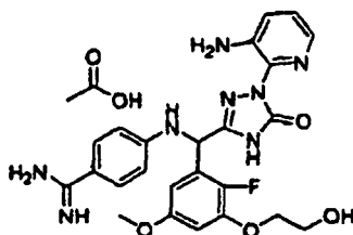
[Chemical Formula 526]
