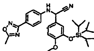
[Chemical Formula 94]
