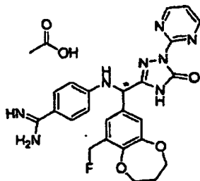
[Chemical Formula 690]
