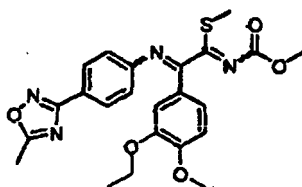
[Chemical Formula 98]
