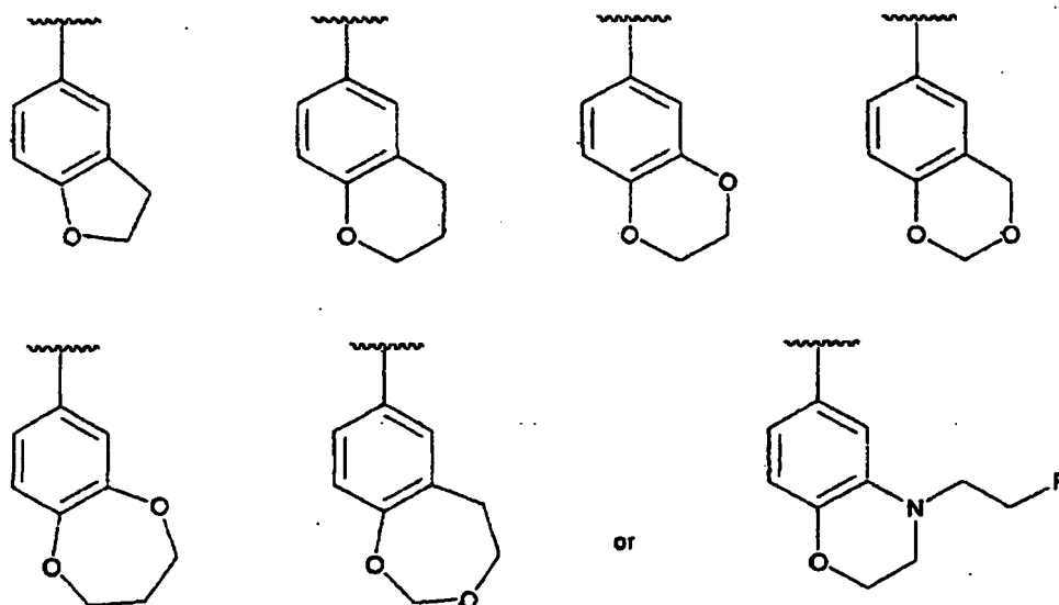
[Chemical Formula 12]
