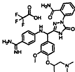
[Chemical Formula 751]
