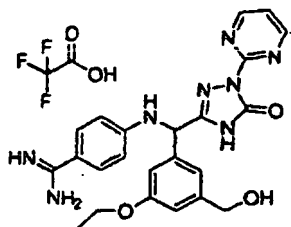
[Chemical Formula 590]
