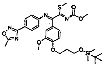
[Chemical Formula 536]
