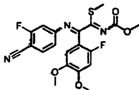
[Chemical Formula 377]
