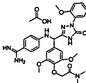
[Chemical Formula 586]
