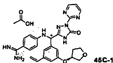
[Chemical Formula 197]
