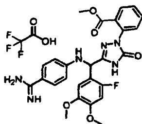
[Chemical Formula 299]
