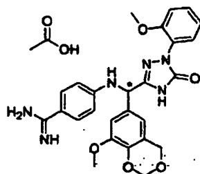
[Chemical Formula 278]
