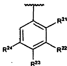
[Chemical Formula 4]
