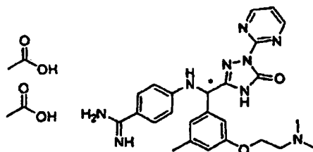
[Chemical Formula 827]
