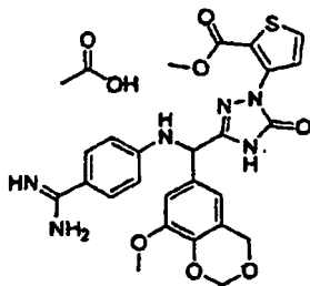
[Chemical Formula 388]
