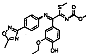
[Chemical Formula 307]
