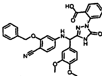
[Chemical Formula 474]
