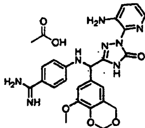
[Chemical Formula 217]
