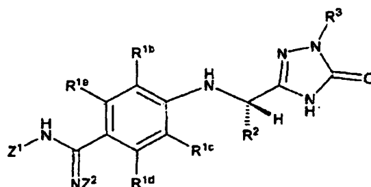
[Chemical Formula 3]
