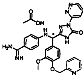
[Chemical Formula 754]
