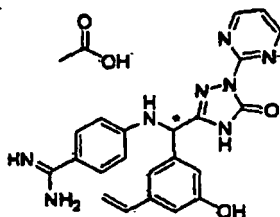
[Chemical Formula 200]
