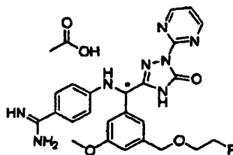
[Chemical Formula 238]
