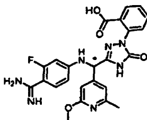
[Chemical Formula 440]
