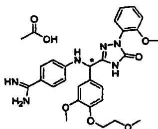
[Chemical Formula 662]
