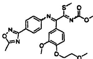
[Chemical Formula 510]
