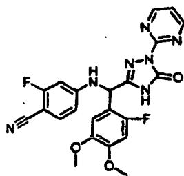
[Chemical Formula 378]
