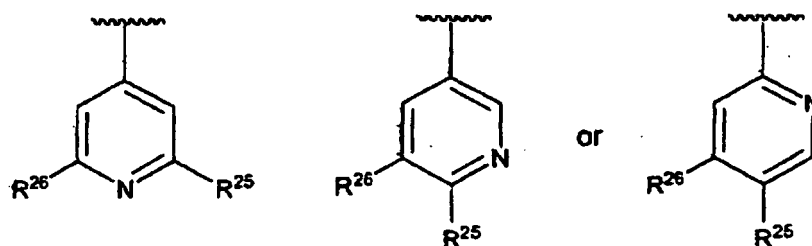
[Chemical Formula 5]
