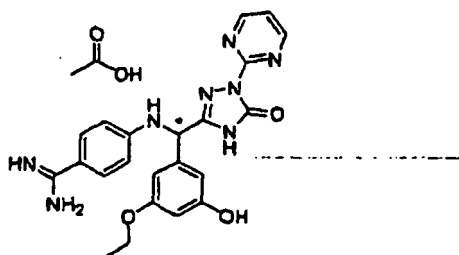
[Chemical Formula 561]
