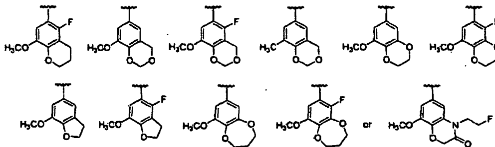
[Chemical Formula 21]
