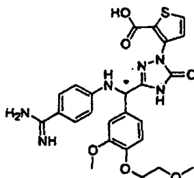
[Chemical Formula 511]
