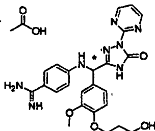
[Chemical Formula 825]
