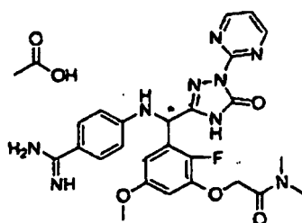
{Chemical Formula 90}
