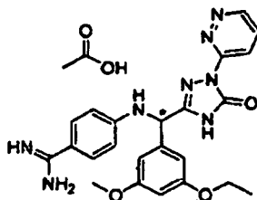
[Chemical Formula 225]
