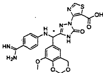
[Chemical Formula 426]
