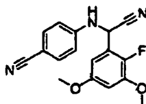
[Chemical Formula 40]
