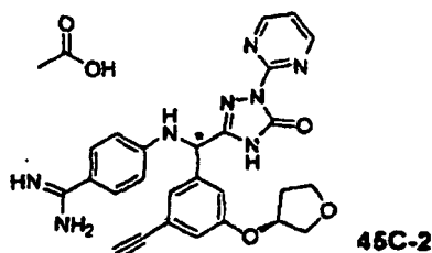
[Chemical Formula 198]
