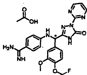
[Chemical Formula 212]
