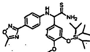
[Chemical Formula 95]
