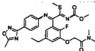
[Chemical Formula 353]
