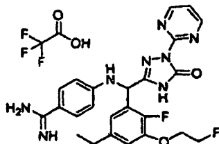
[Chemical Formula 700]
