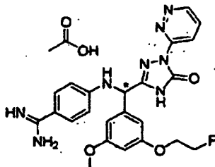
[Chemical Formula 224]
