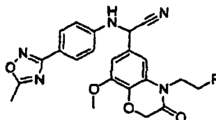
[Chemical Formula 564]
