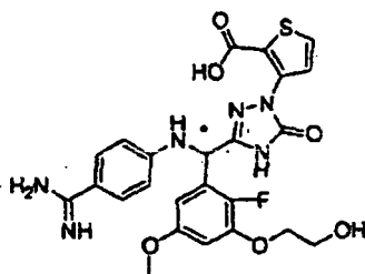
[Chemical Formula 572]
