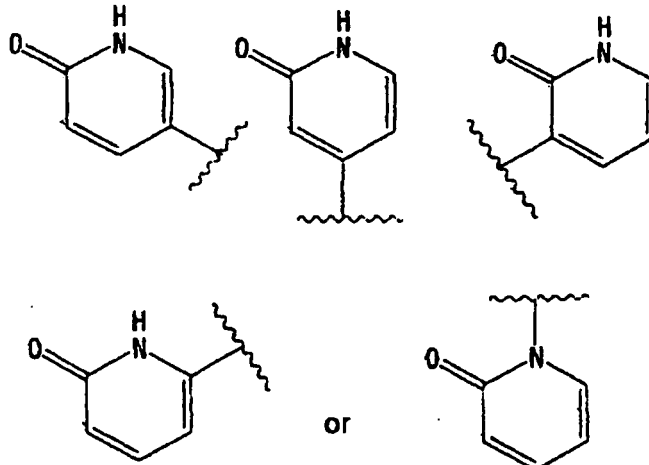
[Chemical Formula 13]
