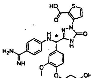
[Chemical Formula 537]
