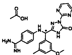
[Chemical Formula 276]
