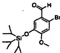
[Chemical Formula 319]
