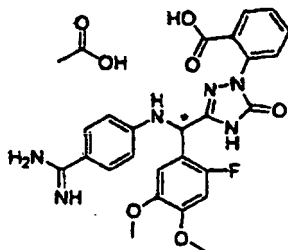
[Chemical Formula 39]
