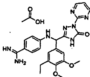
[Chemical Formula 600]
