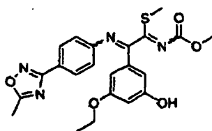
[Chemical Formula 247]
