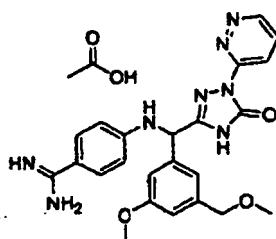
[Chemical Formula 239]
