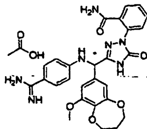
[Chemical Formula 545]
