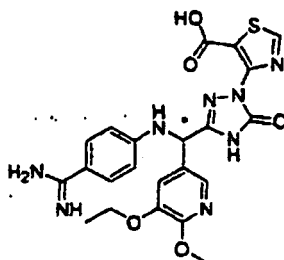
[Chemical Formula 481]
