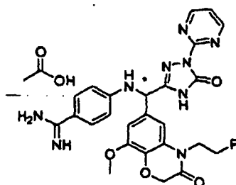
[Chemical Formula 565]
