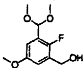
[Chemical Formula 547]
