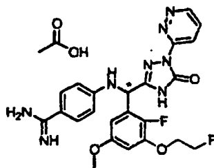
[Chemical Formula 387]
