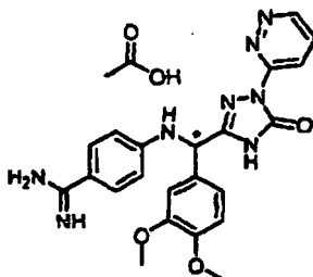
[Chemical Formula 385]
