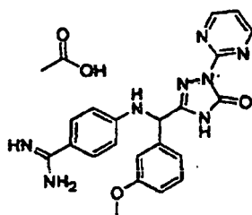
[Chemical Formula 707]
