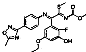
[Chemical Formula 231]
