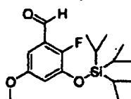
[Chemical Formula 51]
