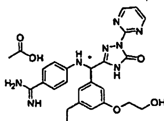
[Chemical Formula 821]
