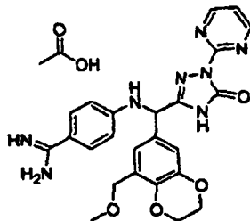
[Chemical Formula 680]
