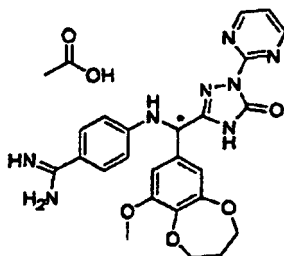
[Chemical Formula 396]
