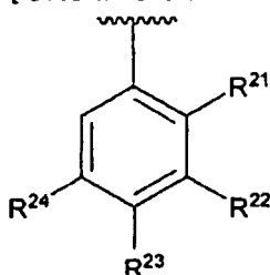
[Chemical Formula 4]
