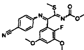
[Chemical Formula 44]
