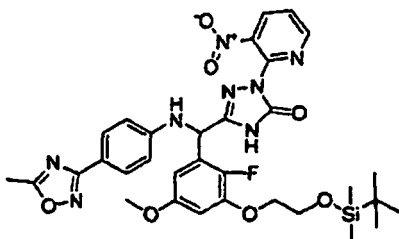
[Chemical Formula 525]
