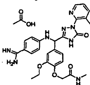
[Chemical Formula 331]
