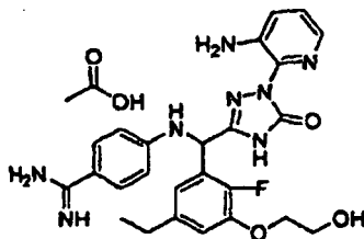
[Chemical Formula 789]
