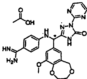
[Chemical Formula 666]
