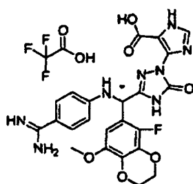
[Chemical Formula 502]
