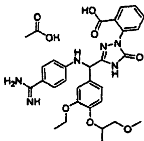
[Chemical Formula 722]
