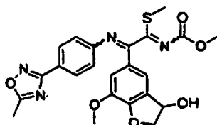
[Chemical Formula 255]
