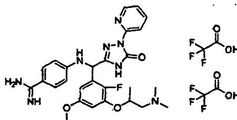
[Chemical Formula 85]
