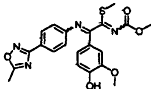
[Chemical Formula 105]
