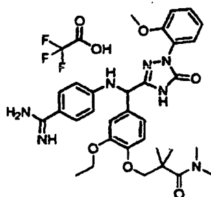
[Chemical Formula 753]
