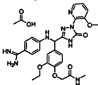
[Chemical Formula 330]
