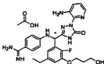
[Chemical Formula 535]
