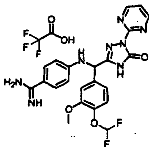
[Chemical Formula 652]
