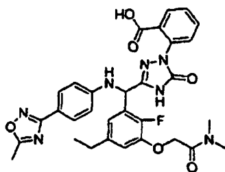
[Chemical Formula 354]
