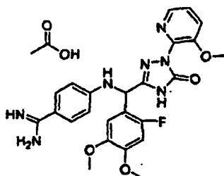
[Chemical Formula 326]
