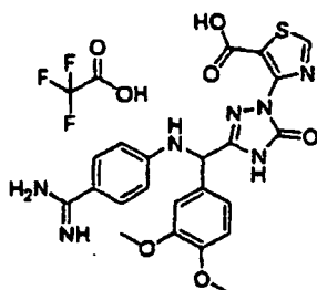
[Chemical Formula 507]
