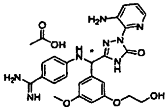
[Chemical Formula 791]
