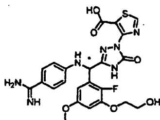
[Chemical Formula 427]
