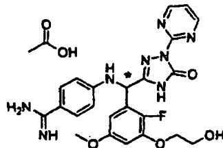
[Chemical Formula 439]
