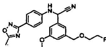
[Chemical Formula 237]
