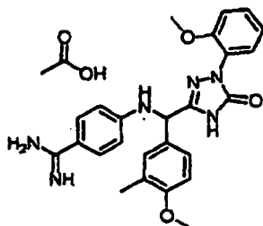
[Chemical Formula 651]
