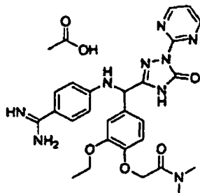
[Chemical Formula 585]
