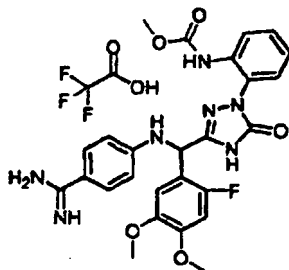
[Chemical Formula 641]
