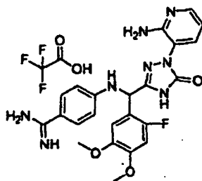
[Chemical Formula 785]
