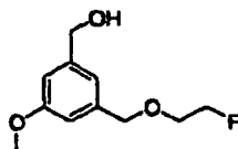
[Chemical Formula 236]
