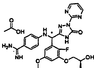
[Chemical Formula 812]
