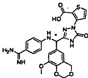
[Chemical Formula 569]
