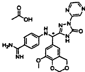
[Chemical Formula 291]
