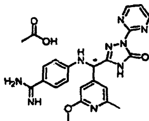
[Chemical Formula 177]
