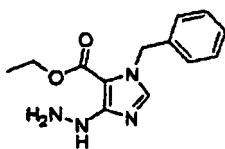
[Chemical Formula 485]
