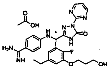
[Chemical Formula 783]
