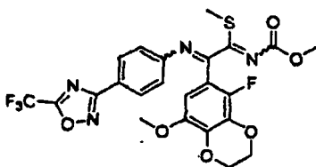
[Chemical Formula 490]
