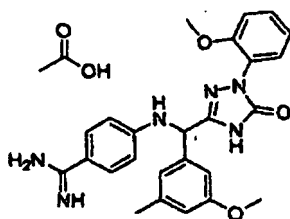
[Chemical Formula 733]
