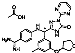
[Chemical Formula 218]
