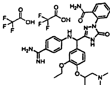
[Chemical Formula 636]
