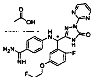
[Chemical Formula 626]
