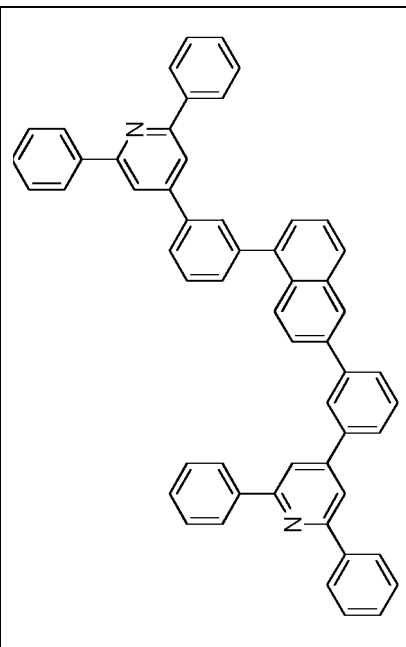
Compound 2-c-10
