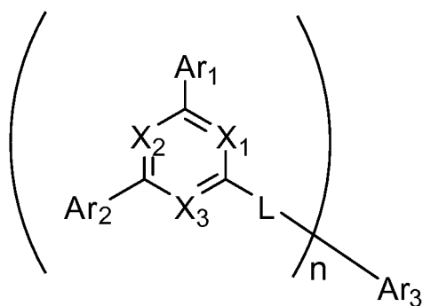
Formula 1
