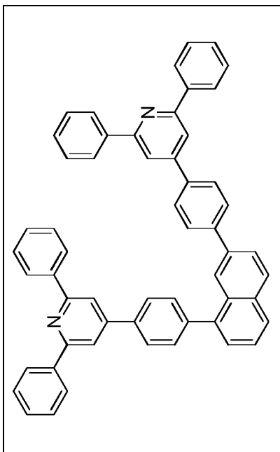
Compound 2-d-8
