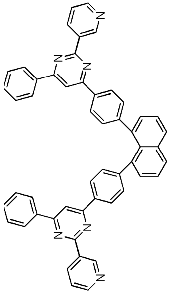
Compound 2-b-3
