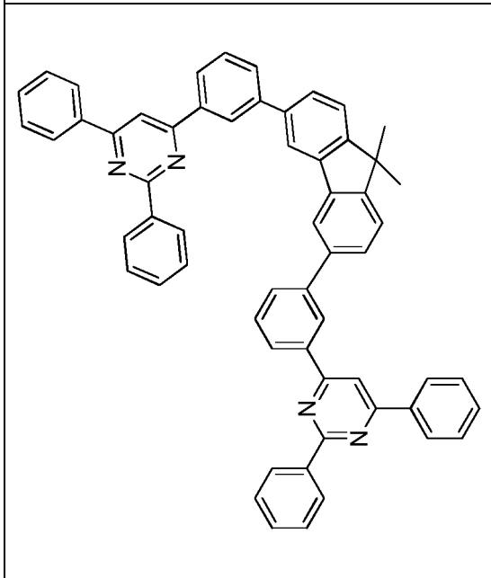
Compound 2-e-7
