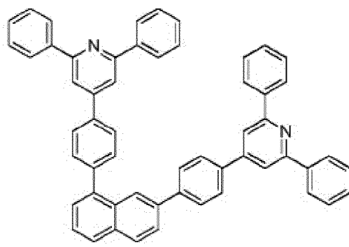
Composé 2-d-8
