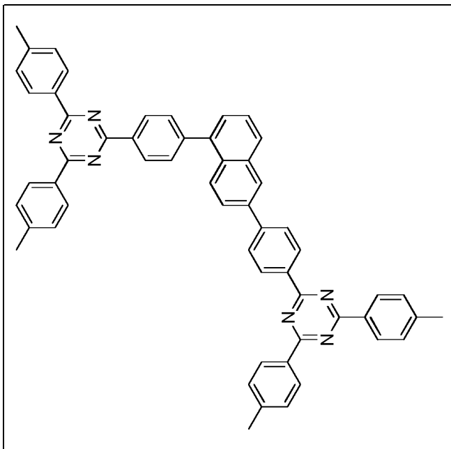
Compound 1-c-10
