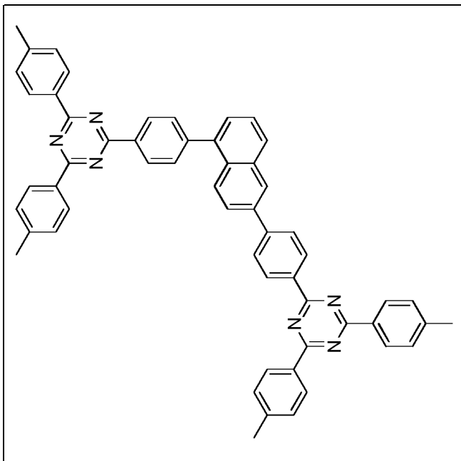
Compound 1-c-10
