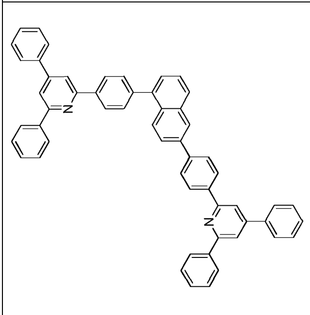
Compound 2-c-9
