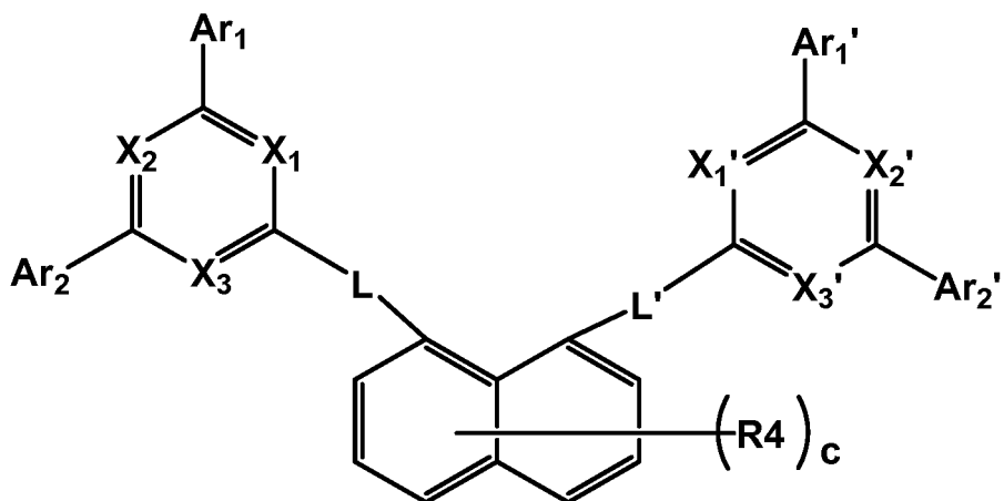
Formula 1-c
