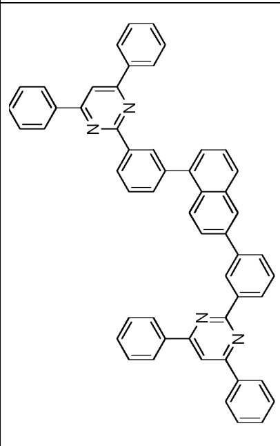
Compound 2-c-9
