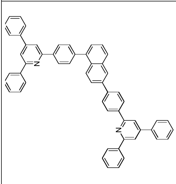
Compound 2-c-9
