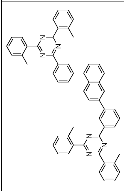
Compound 2-c-1
