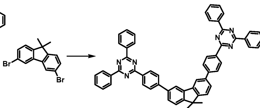
[Compound 1-e-1]
