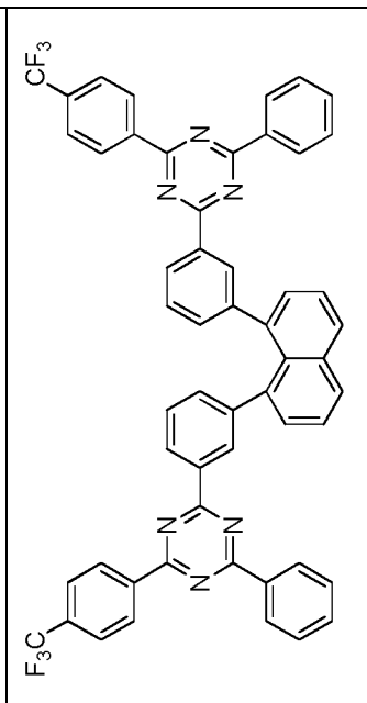
Compound 1-b-14
