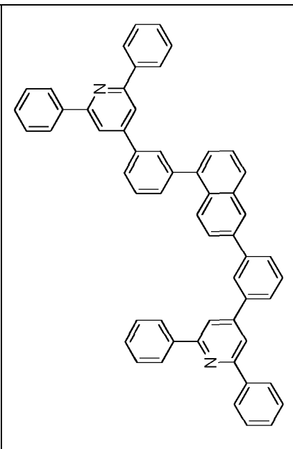
Compound 2-c-10
