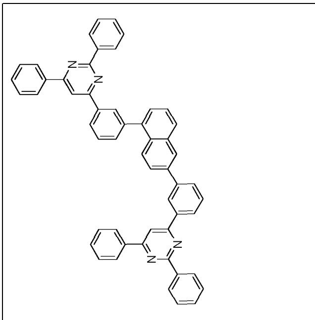
Compound 2-c-10
