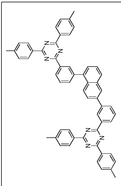
Compound 2-c-2
