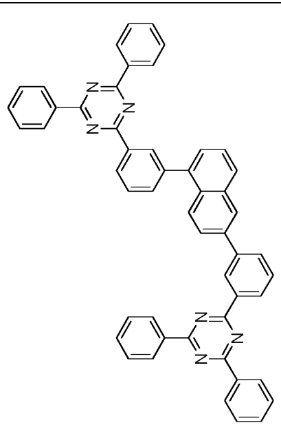
Compound 1-c-11
