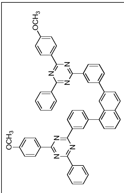
Compound 1-d-12
