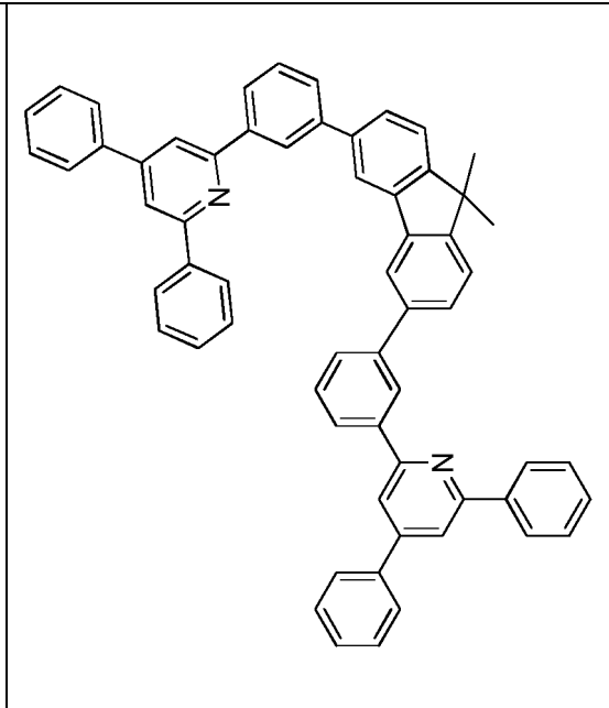
Compound 2-e-8
