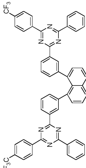
Compound 1-b-14
