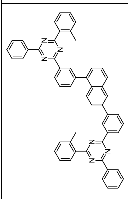
Compound 1-c-13
