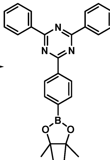
[Compound 1-C]
