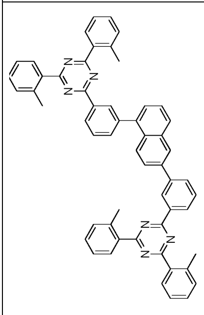
Compound 2-c-1
