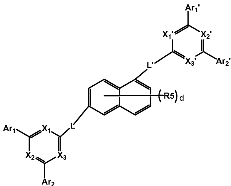
Formula 1-d
