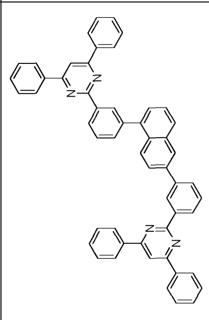
Compound 2-c-9
