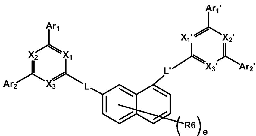
Formula 1-d
