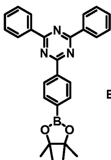
[Compound 1-C]
