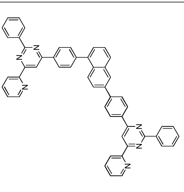
Compound 2-c-4
