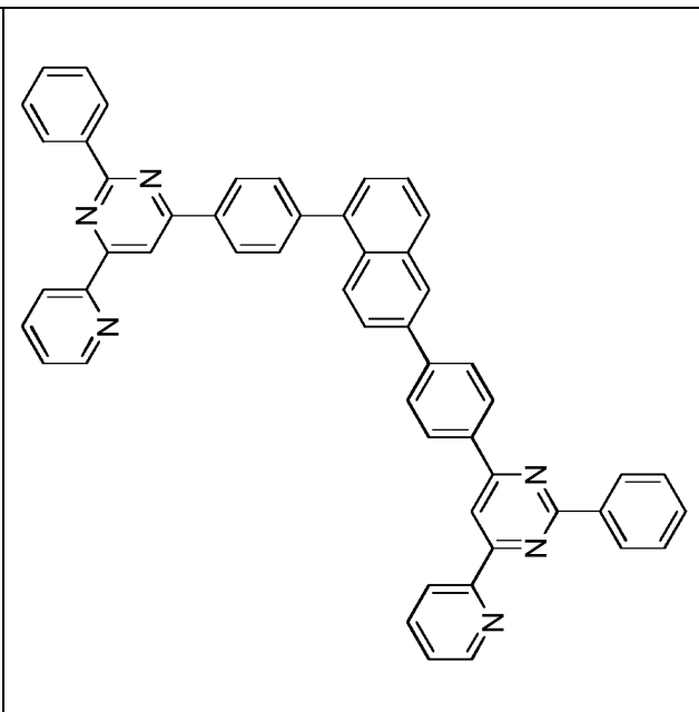
Compound 2-c-2
