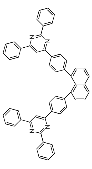
Compound 2-b-3
