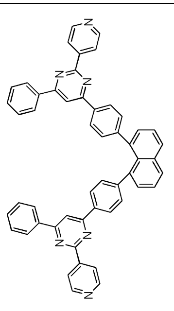
Compound 2-b-4
