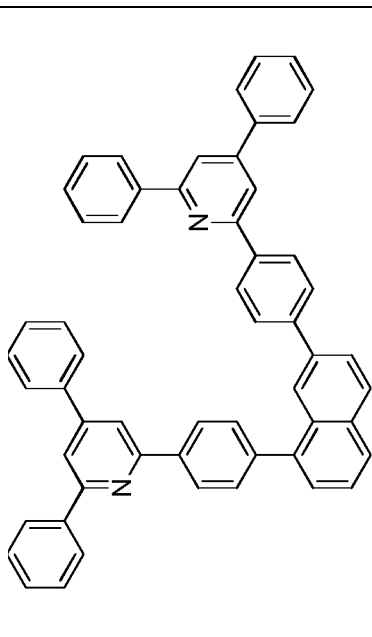
Compound 2-d-7
