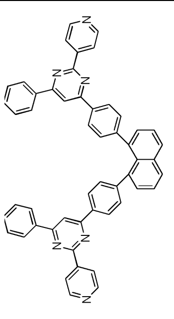
Compound 2-b-4
