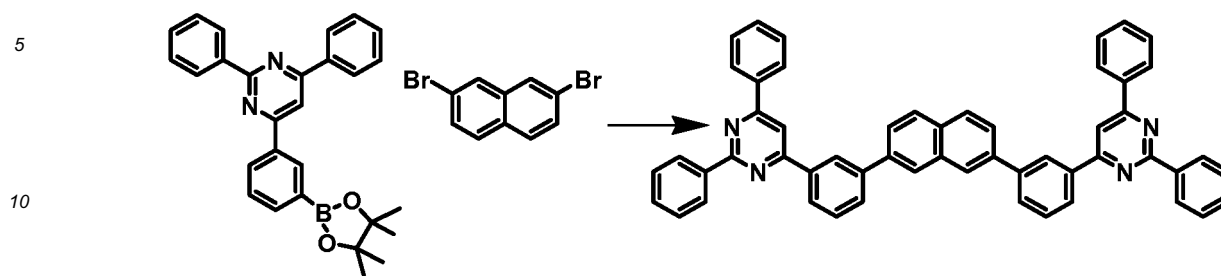
[Compound 4-B]
