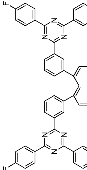
Compound 1-b-13
