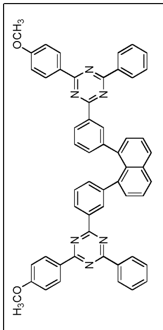
Compound 1-b-12
