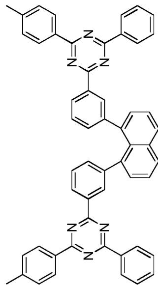
Compound 1-b-12
