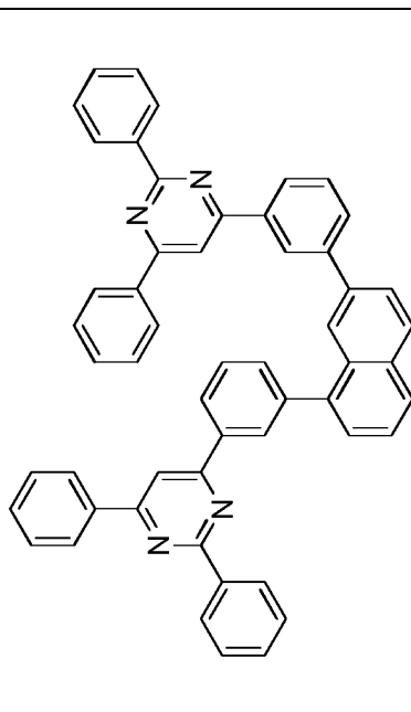
Compound 2-d-8
