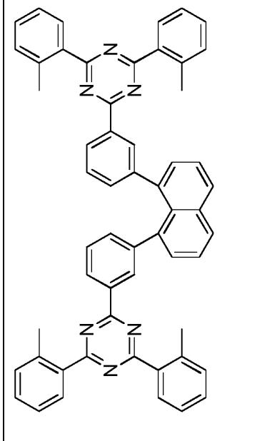
Compound 2-b-1
