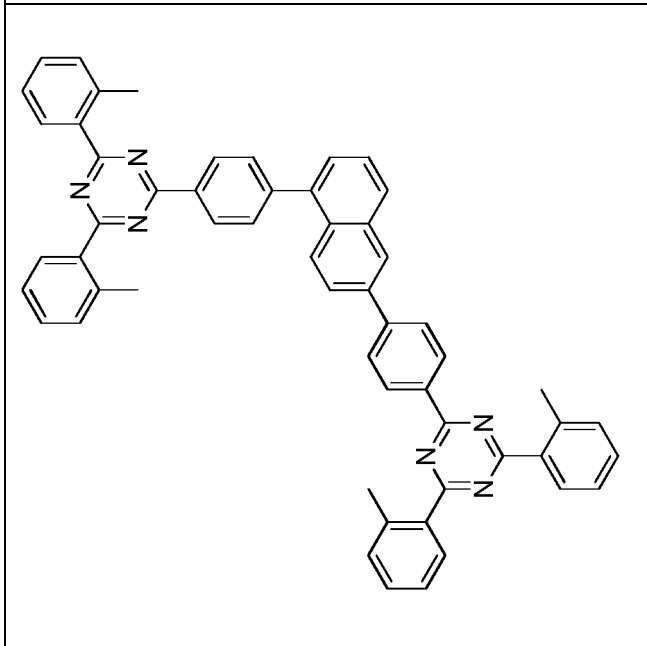
Compound 1-c-9
