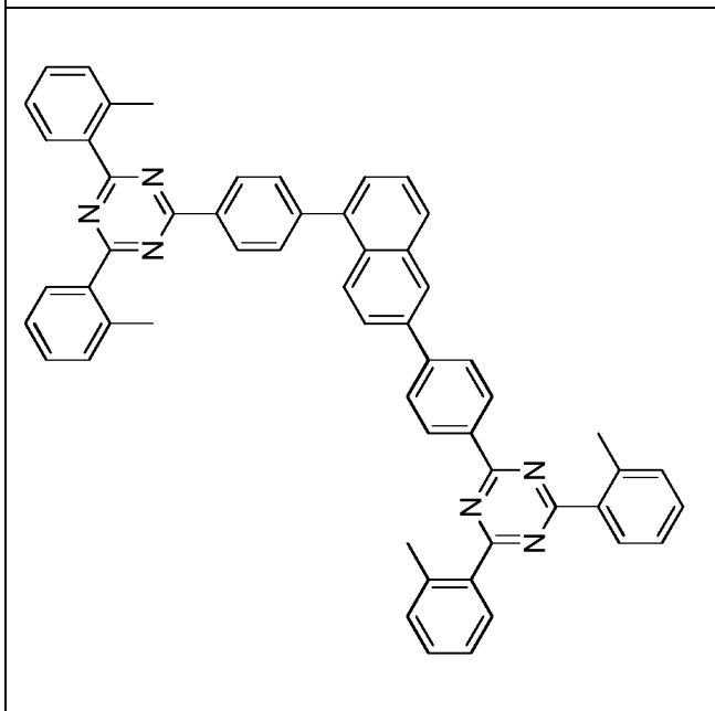
Compound 1-c-9
