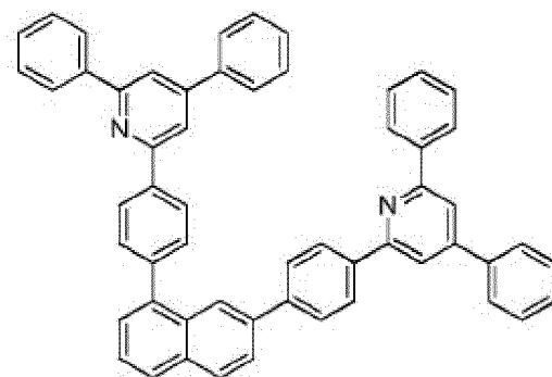
Composé 2-d-9
