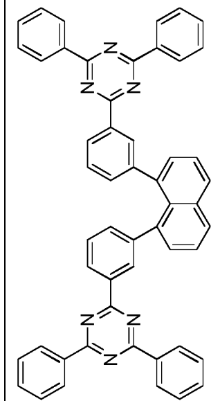
Compound 1-b-11
