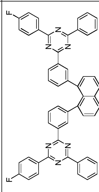
Compound 1-b-13
