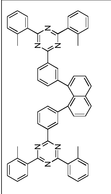
Compound 2-b-1
