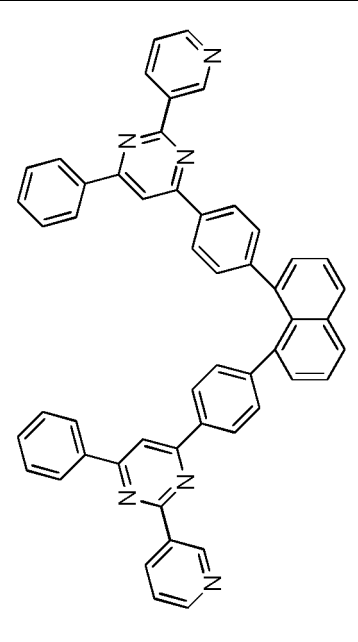
Compound 2-b-3
