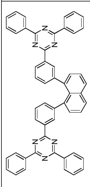
Compound 1-b-11
