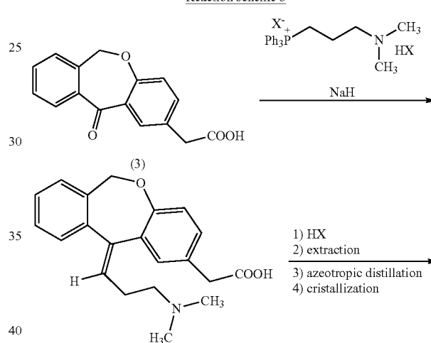
Reaction scheme 3
