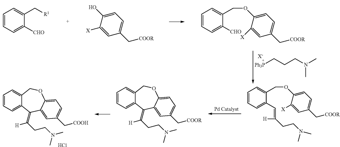
Reaction scheme 2
