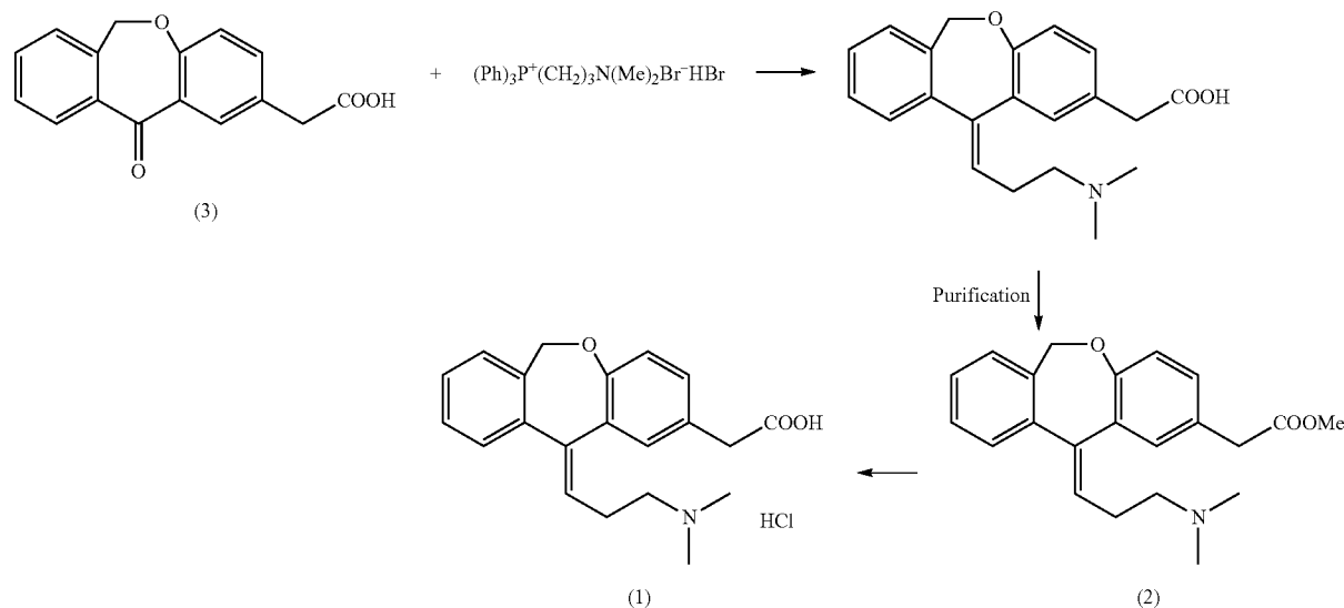
Reaction scheme 1
