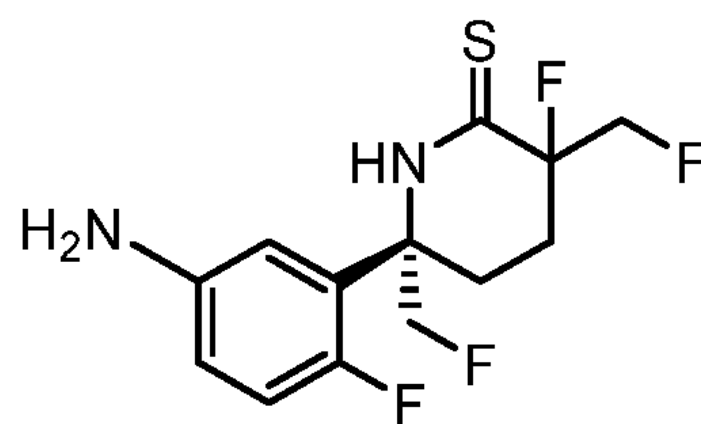
(6 S )-6-(5-amino-2-fluorophenyl)-3-fluoro-3,6-bis(fluoromethyl)piperidine-2-thione
