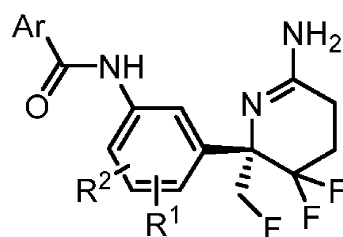
Formula I
