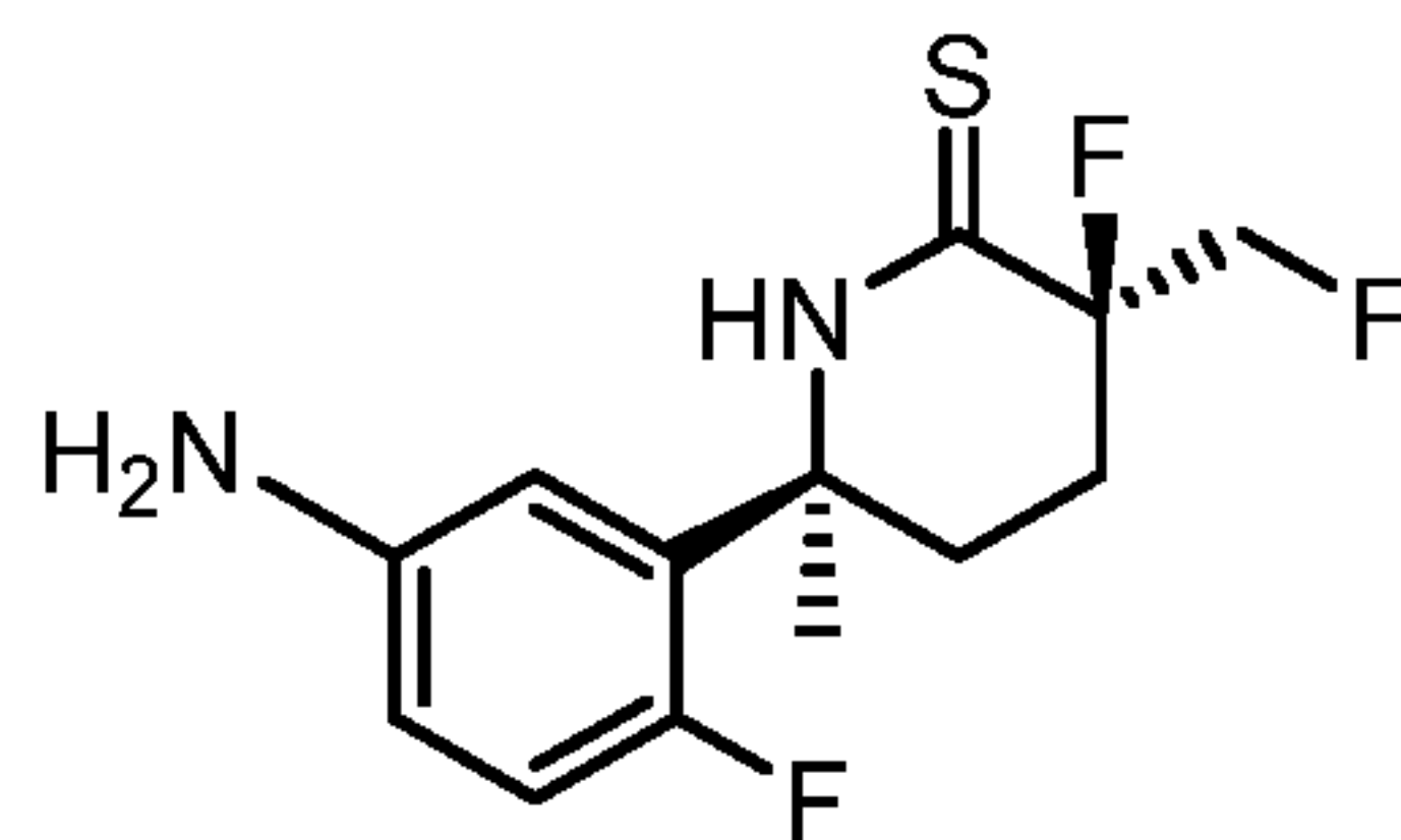
10 (3 R ,6 S )-6-(5-amino-2-fluorophenyl)-3-fluoro-3-(fluoromethyl)-6-methylpiperidine-2-thione
