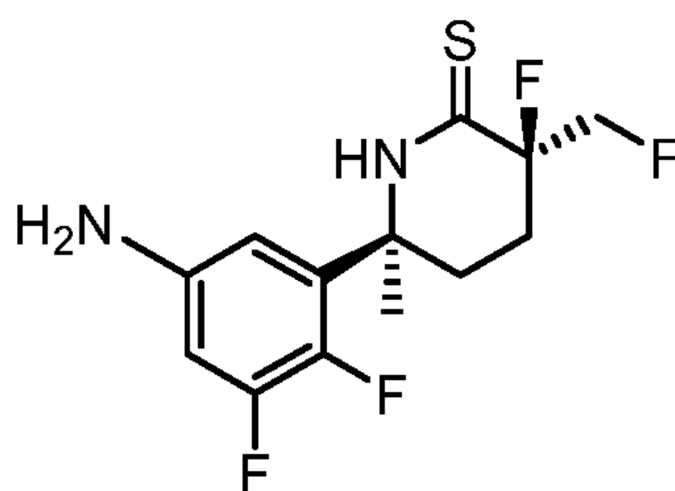
(3R,6S)-6-(5-amino-2,3-difluorophenyl)-3-fluoro-3-(fluoromethyl)-6-methylpiperidine-2-thione
