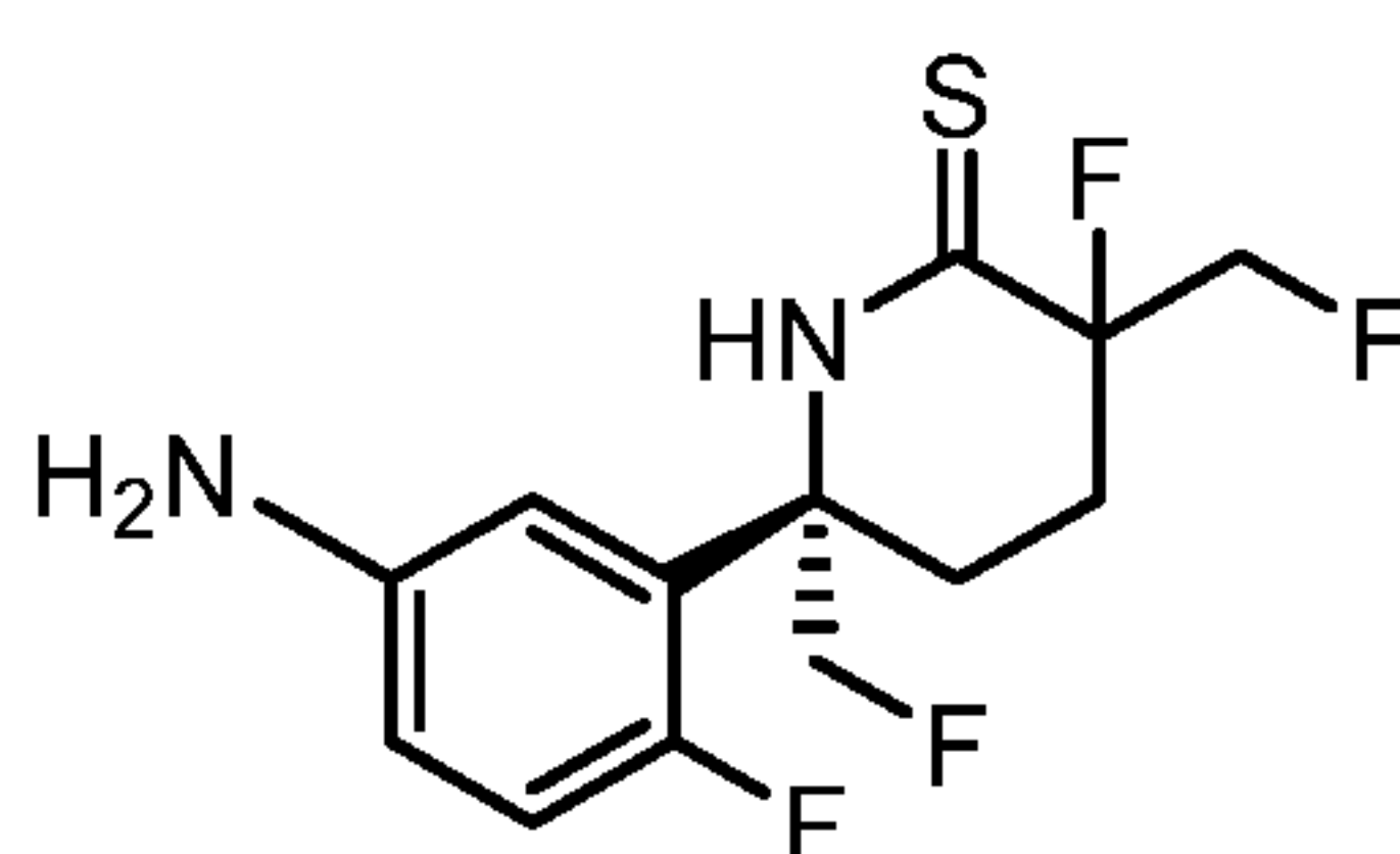
(6S)-6-(5-amino-2-fluorophenyl)-3-fluoro-3,6-bis(fluoromethyl)piperidine-2-thione
