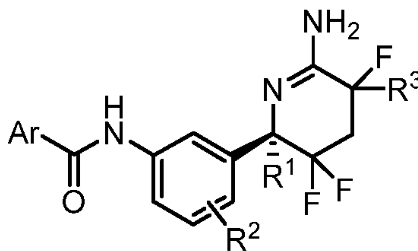
Formula II
