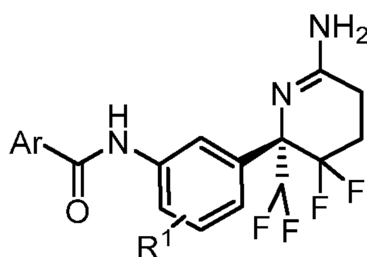
Formula I
