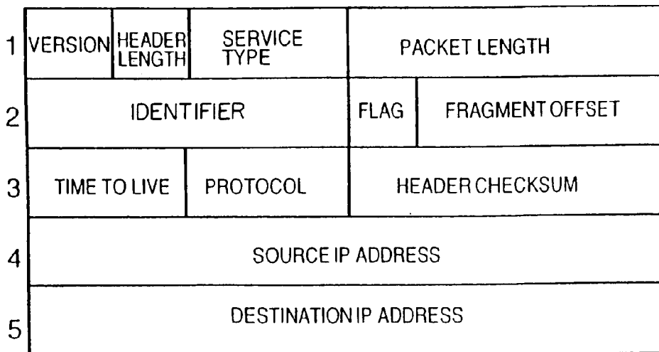
FIG. 11B IPv4 HEADER FORMAT
