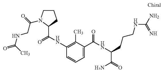
ST2864: Ac-Gly-Pro-SP30-Arg-NH 2
