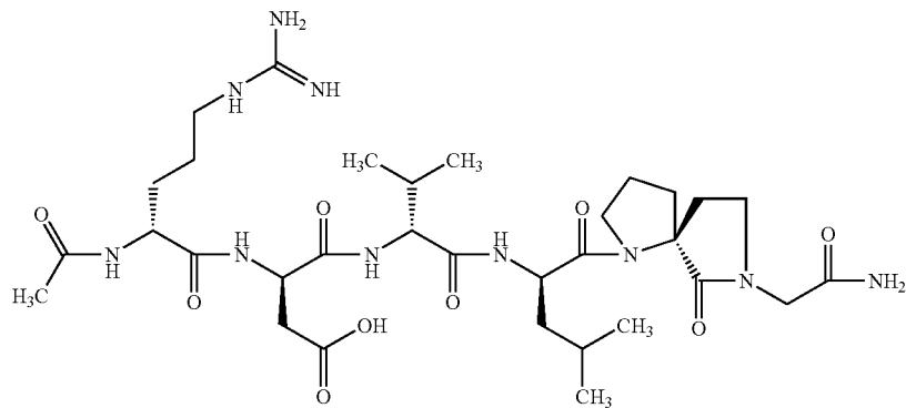
ST2799: Ac-arg-asp-val-leu-Beta1-NH 2
