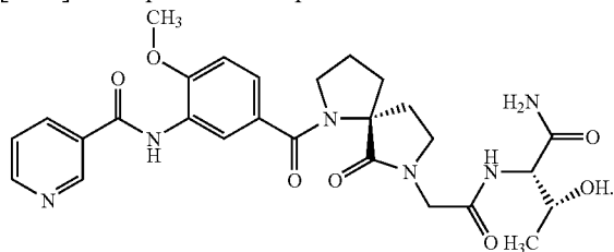
ST2792: PAM9-SP02-Beta2-Thr-NH 2
