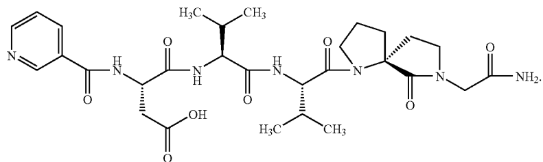
ST2794: PAM9-Asp-Val-Val-Beta2-NH 2
