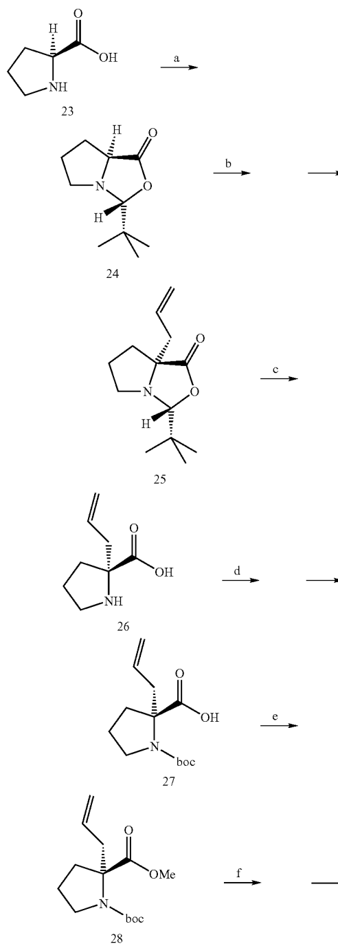
Scheme 3 Synthesis of ST2535
