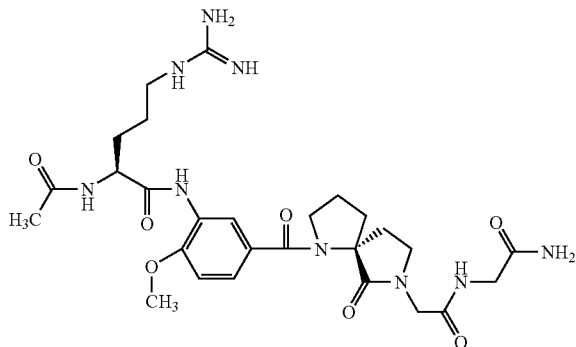
ST2801: Ac-Arg-SP12-Beta2-Thr-NH 2
