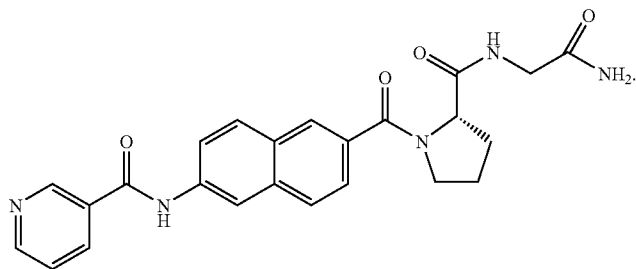
ST2798: PAM9-SP38-Pro-Gly-NH 2
