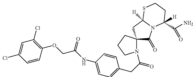
ST2825: PAM4-SP19-Beta8-NH 2
