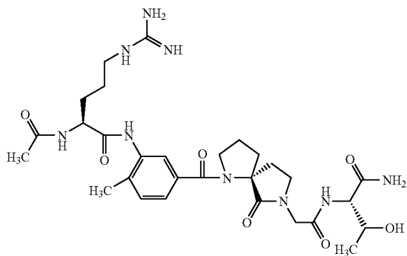
ST2801: Ac-Arg-SP12-Beta2-Thr-NH 2
