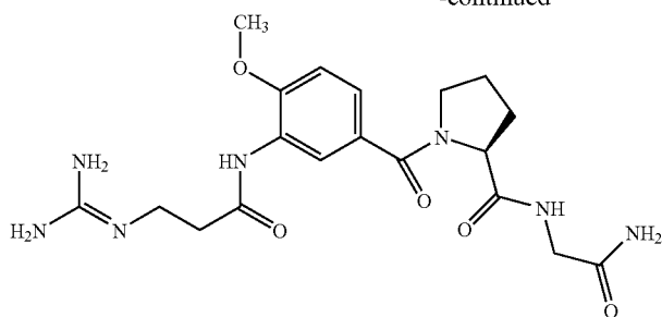
ST2796: AM9-SP02-Pro-Gly-NH 2
