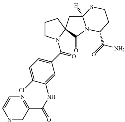
ST3374: PAM10-SP6-Beta8-NH 2
