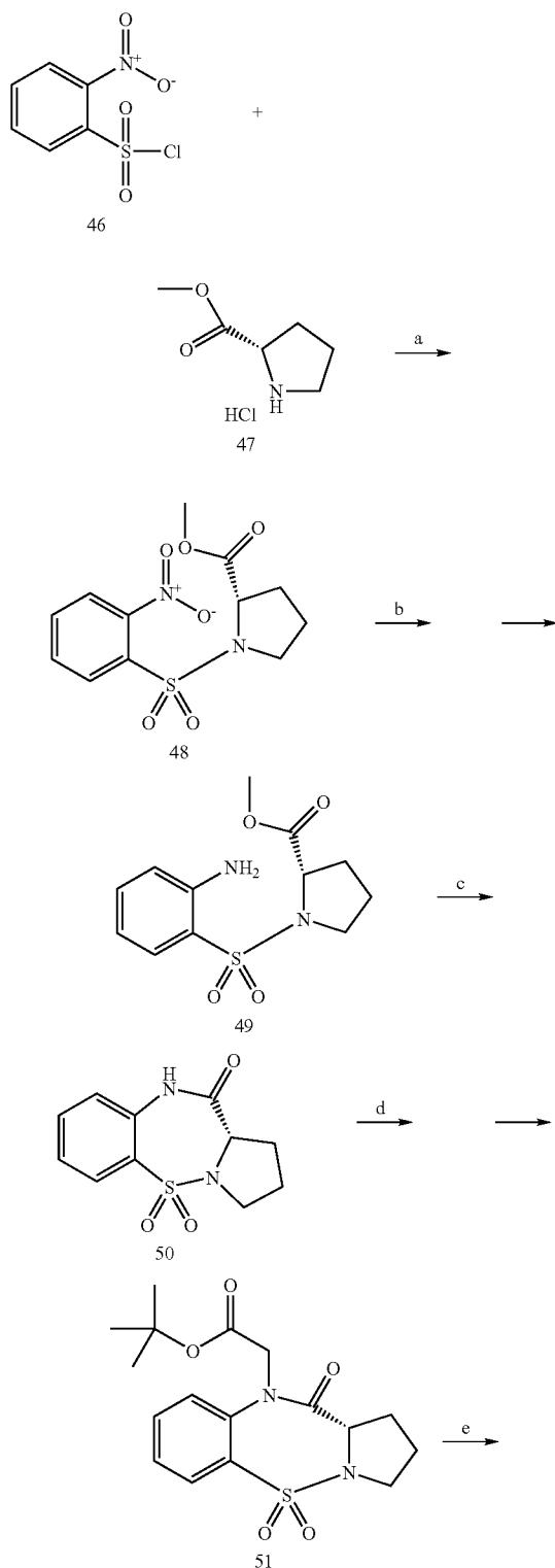
Scheme 6 Synthesis of ST2590
