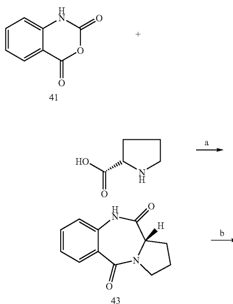
Scheme 5 Synthesis of ST2393
