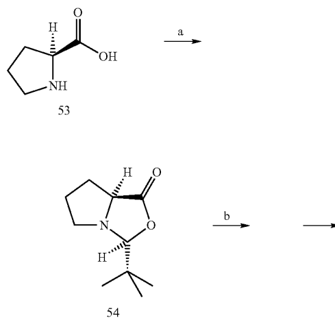
Scheme 7 Synthesis of ST2610
