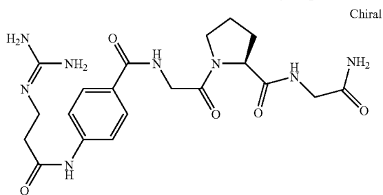
ST2863: AM9-SP17-Pro-Gly-NH 2
