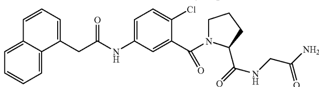
ST2797: PAM8-SP15-Pro-Gly-NH 2
