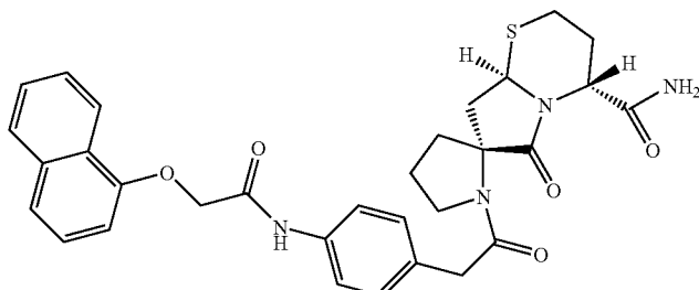
ST3324: PAM11-SP19-Beta8-NH 2
