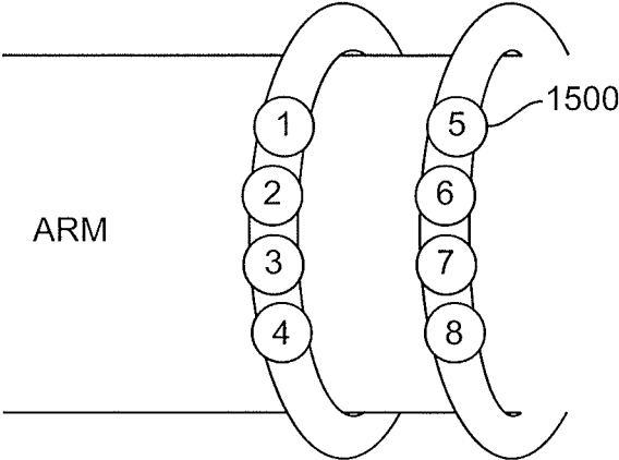
2 bands, each with a linear array of electrodes
