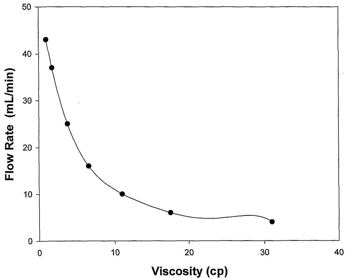
Figure 1. Flow rate of different viscosity irrigating solutions through an irrigation/aspiration tip, using Legacy 20000 at its default settings.
