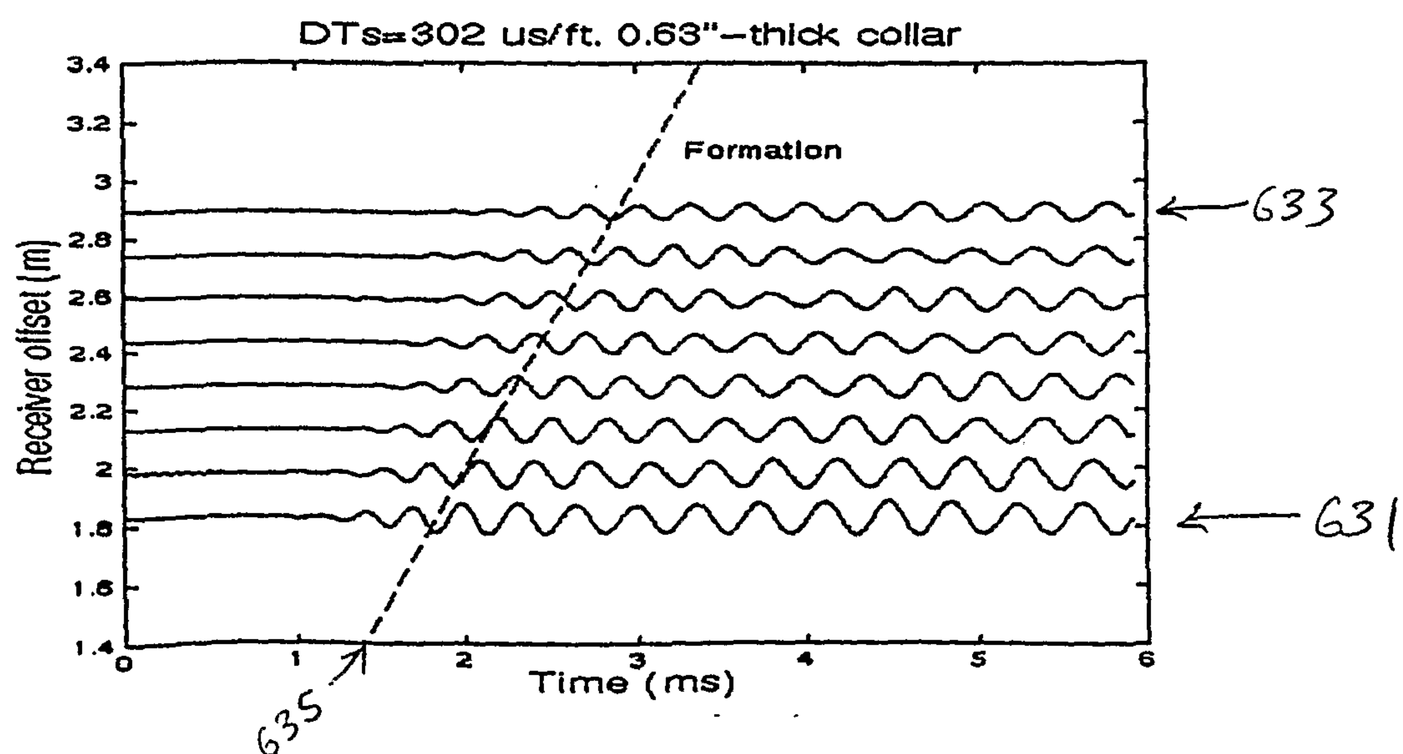
Figure 6B Quadrupole waveforms, thin collar pipe
