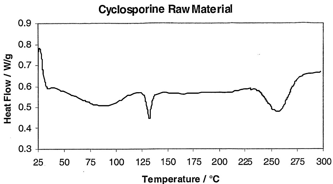
Figure 7: Normalized DSC thermogram of Cyclosporine active pharmaceutical ingredient
