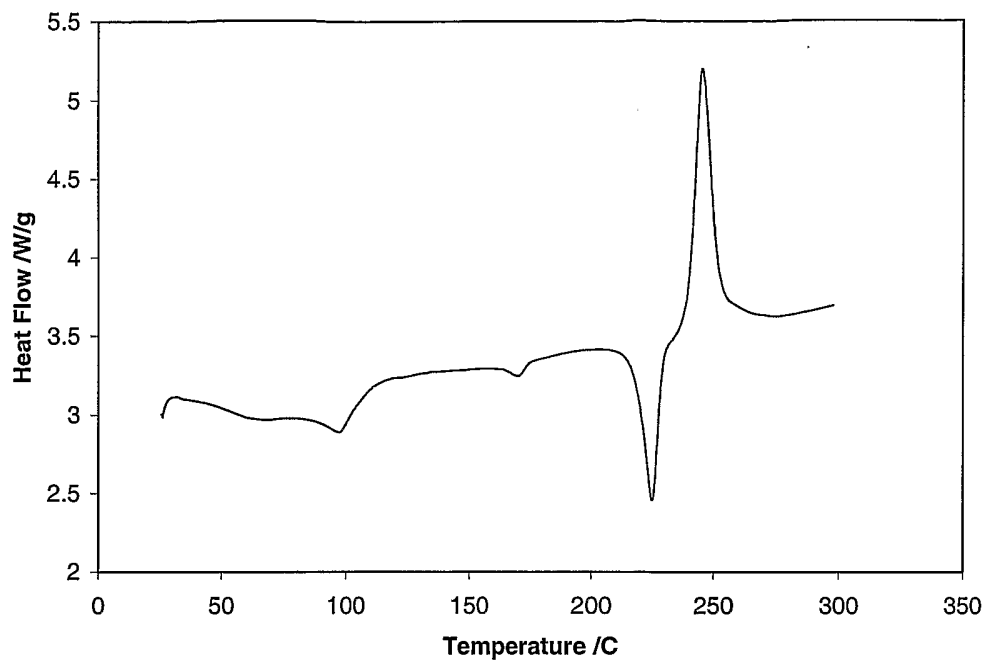
Figure 9: Normalized thermogram of Paclitaxel Active Pharmaceutical Ingredient
