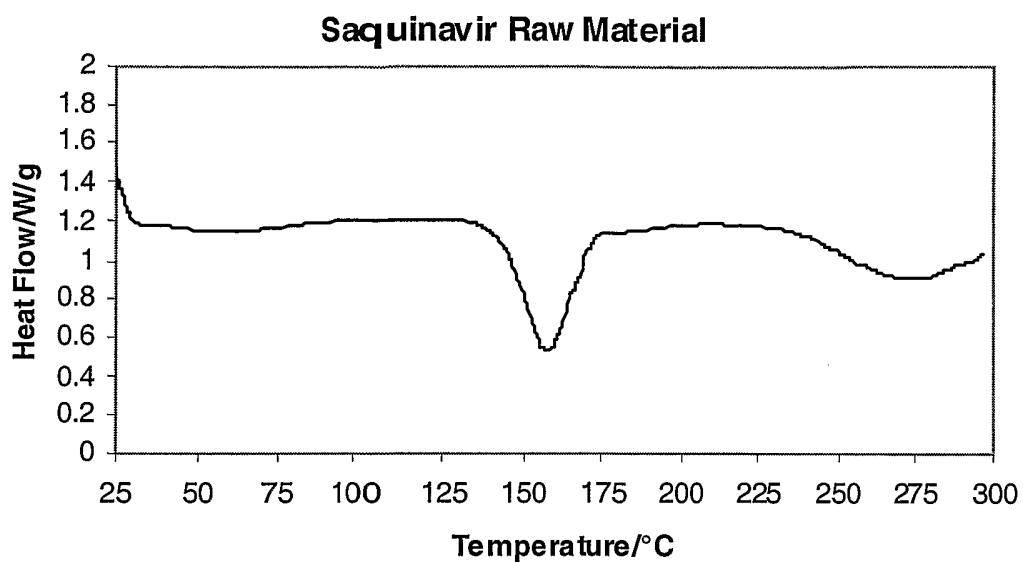
Figure 5: Normalized DSC thermogram of Saquinavir active pharmaceutical ingredient
