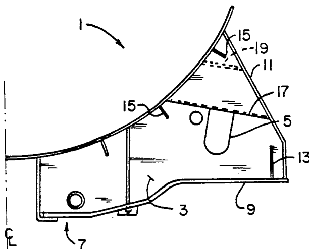
FIG. 5. PRIOR ART.
