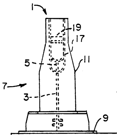
FIG. 6. PRIOR ART.
