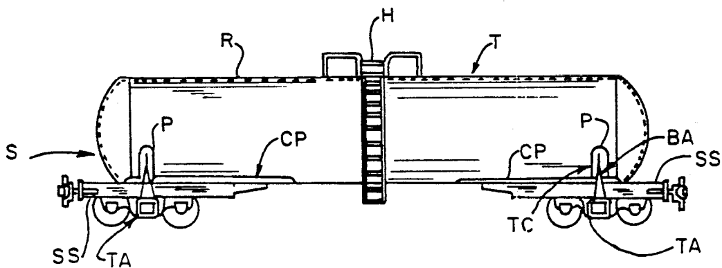
FIG. 6. PRIOR ART.
