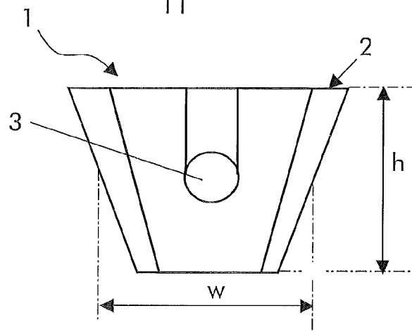
Fig. 3 Prior art
