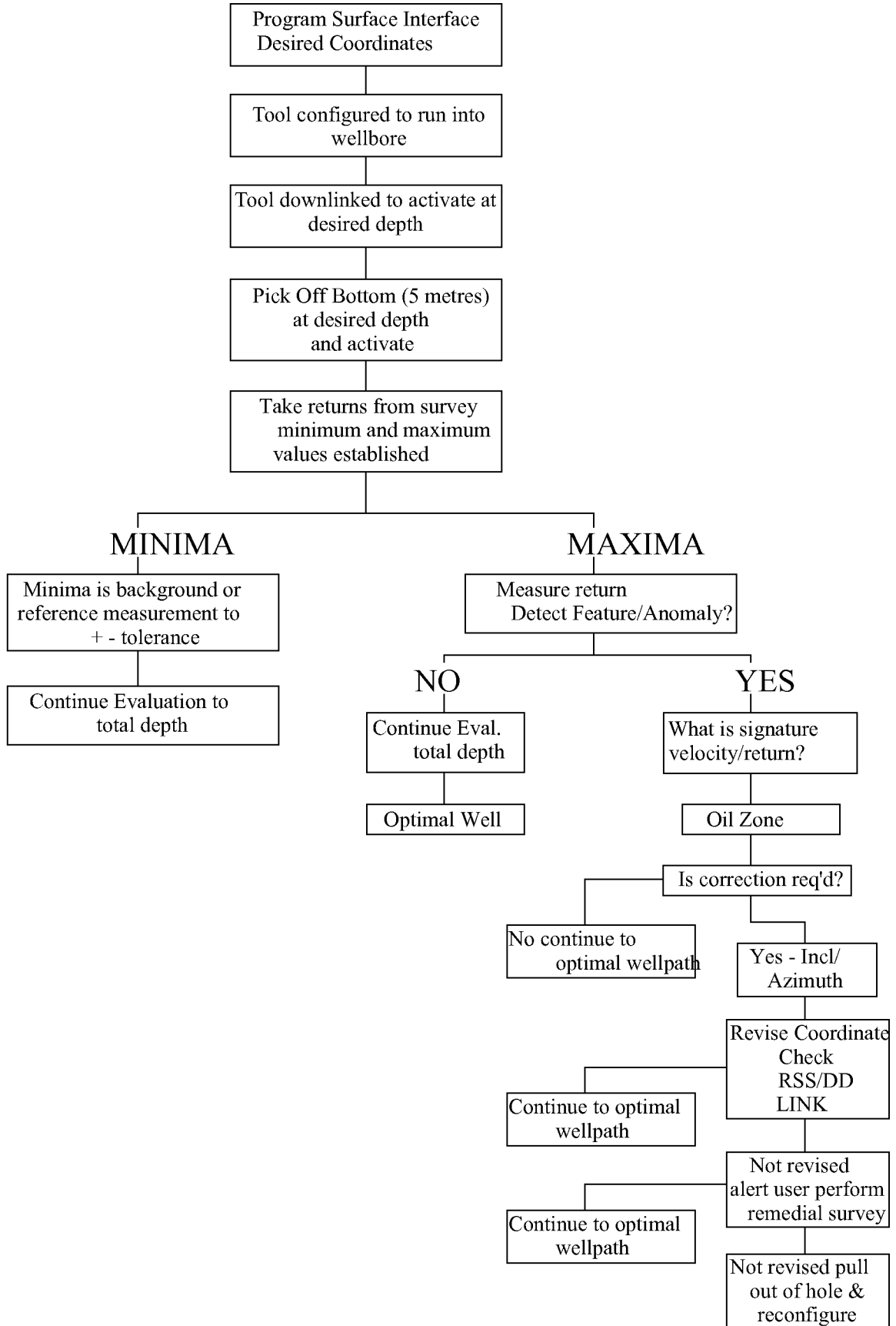
Figure 9 Logic Circuit for Lookahead Formation Evaluation Tool
