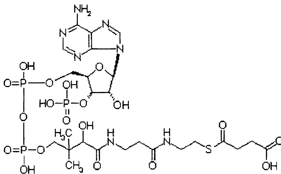
Succinyl-coenzyme A
