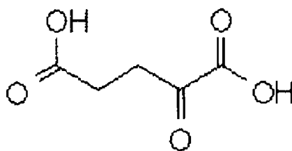
2-Oxoglutarate
