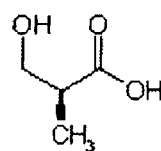
3-Hydroxyisobutyric acid
