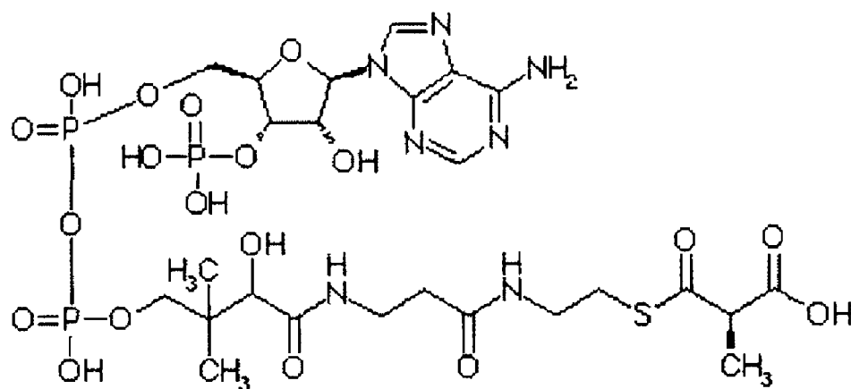
Methylmalonyl-coenzyme A
