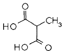
Methyl malonate
