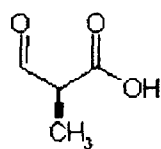
Methylmalonate semialdehyde
