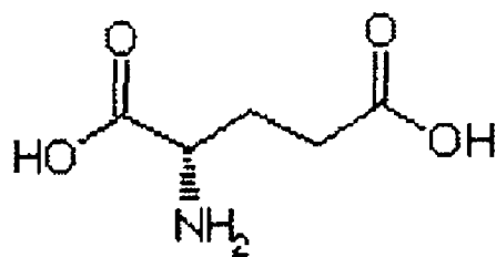
L-Glutamate
