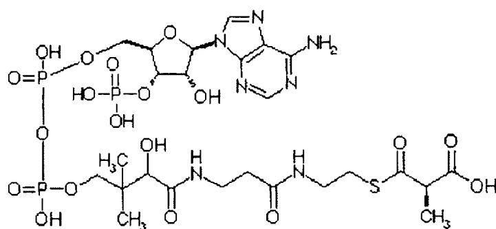
Methylmalonyl-coenzyme A
