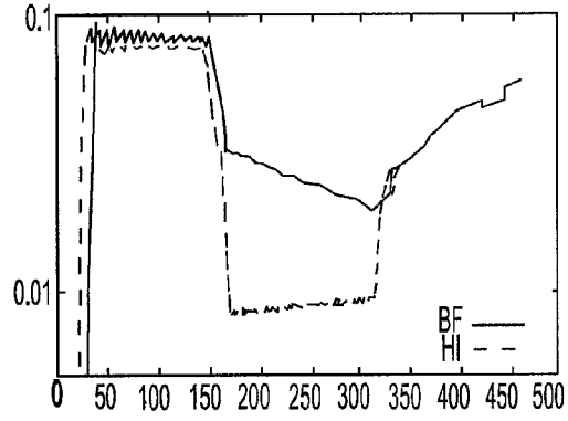
FIG. 4c REWARD, DECAY=1.0
