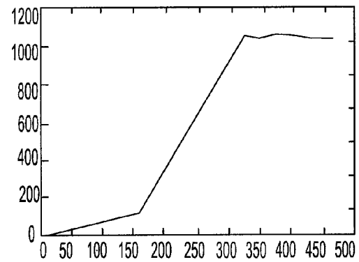
FIG. 4i CHOICE, DECAY=1.0
