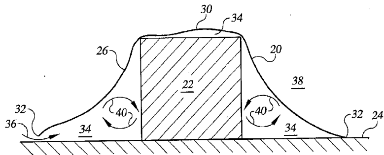
FIG. 1 PRIOR ART
