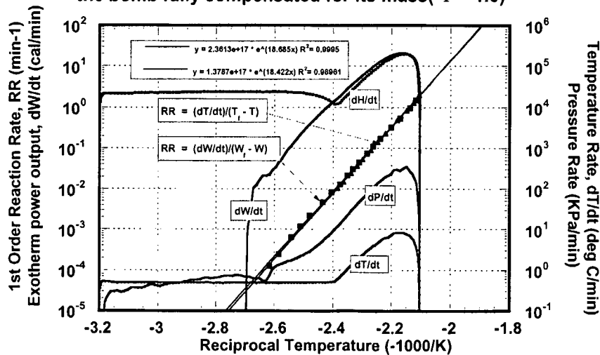
Figure 8. 5 g 10.0% dtbp in a 18 g SS bomb ramped at 0.5 deg C/min and the bomb fully compensated for its mass ( \Phi = 1.0 )
