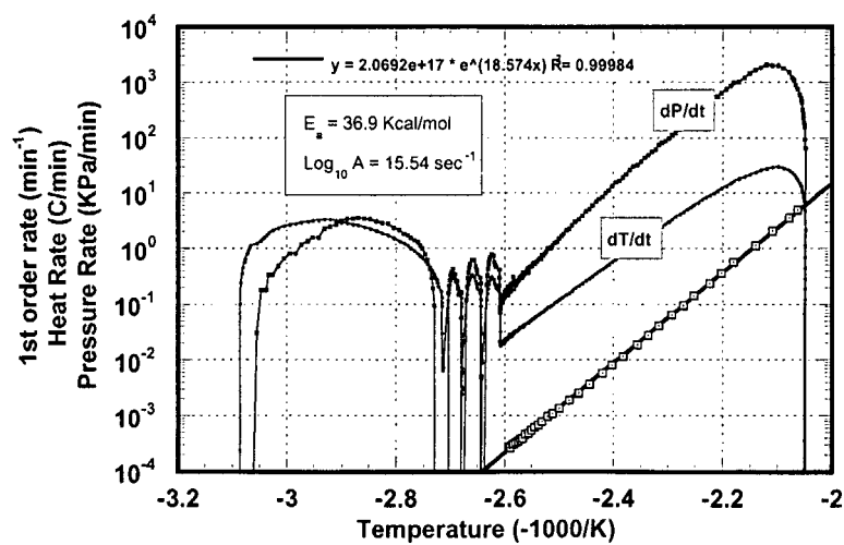
Figure 2. 6 g 20% DTBP in toluene in a 6 g titanium bomb
