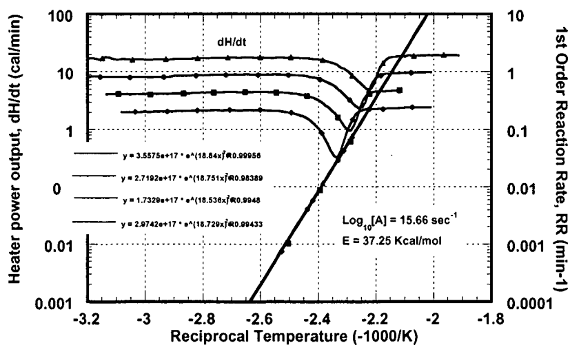
Figure 16. 3 g 16.7% solution DTBP in Toluene heated at 0.25, 0.5, 1.0 and 2.0 C/min in a 71 g Hasteloy C bomb and stirred at 200 rpm.
