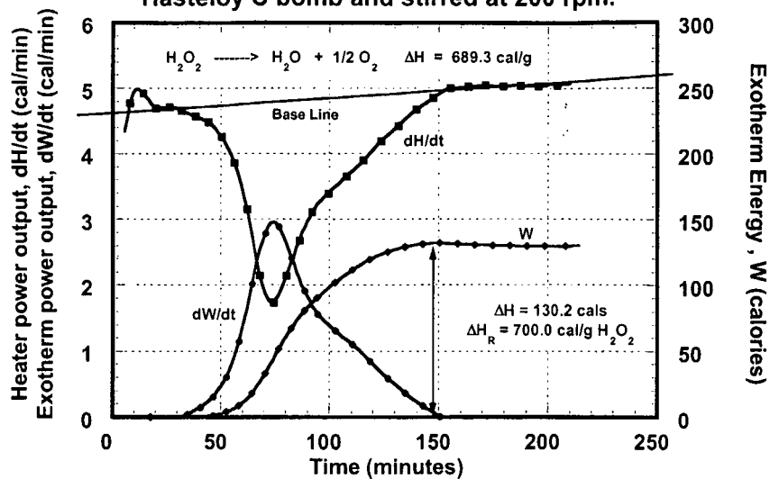
Figure 17. 3.0 g 6.2% \text{H}_2\text{O}_2 heated at 0.5 C/min in a 71 g Hasteloy C bomb and stirred at 200 rpm.
