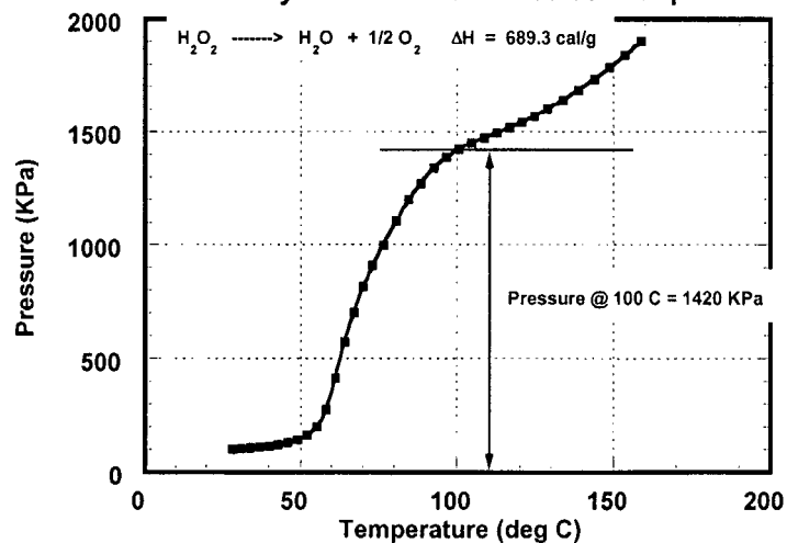
Figure 18. 3.0 g 6.2% \text{H}_2\text{O}_2 heated at 0.5 C/min in a 71 g Hasteloy C bomb and stirred at 200 rpm.
