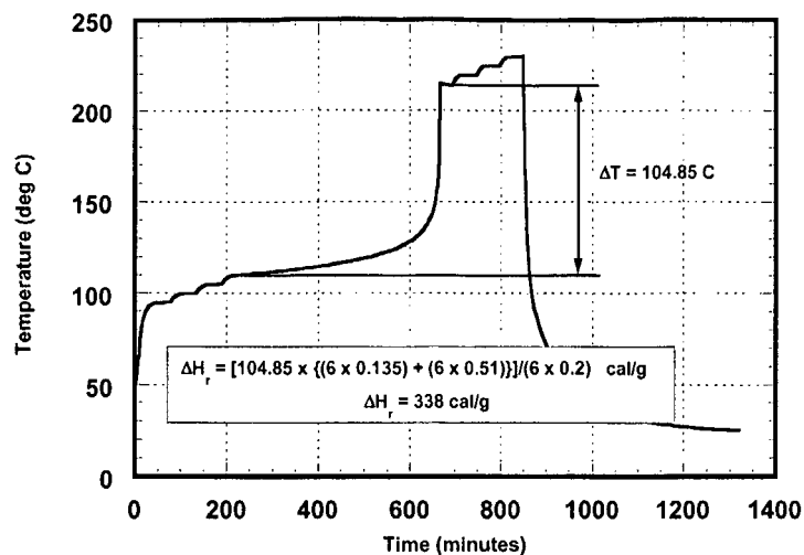
Figure 1. 6 g 20% DTBP in Toluene in a 6 g Ti Bomb
