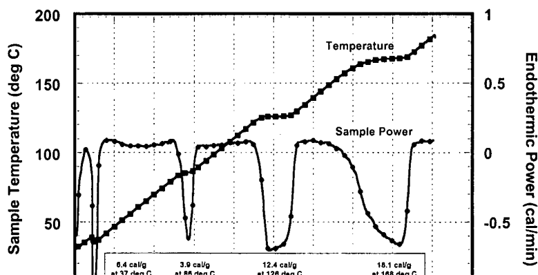
Figure 11. 4g NH 4 NO 3 in a 10.6 g SS bomb heated at constant power (0.05 Watts)
