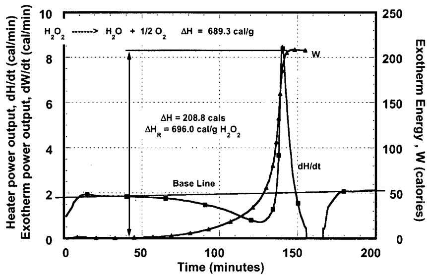
Figure 12. 3.0 g 10% \text{H}_2\text{O}_2 heated at 0.5 C/min in a 9.7 g 316 SS bomb and stirred at 200 rpm. Bomb thermally compensated to \Phi = 1.0
