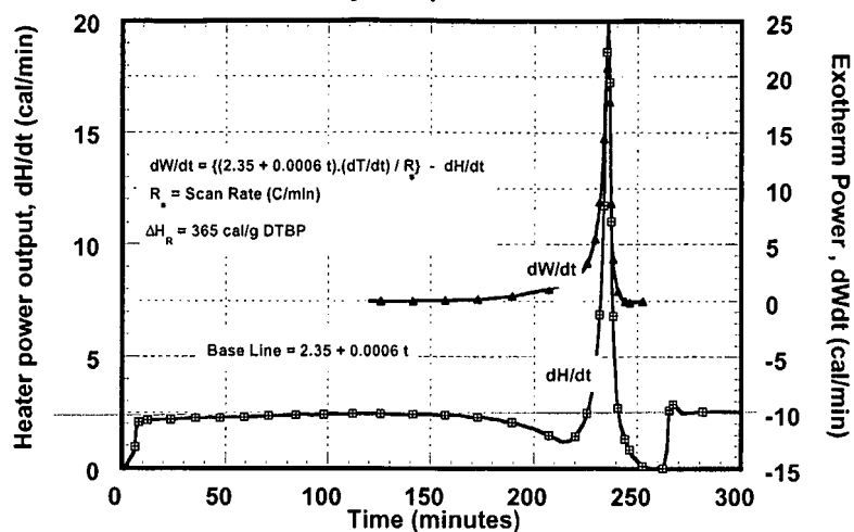
Figure 7. 5.0 g 10% DTBP heated at 0.5 C/min in a 18 g 316 SS bomb Bomb thermally compensated to \Phi = 1.0
