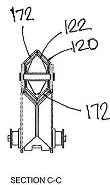
SECTION C-C
