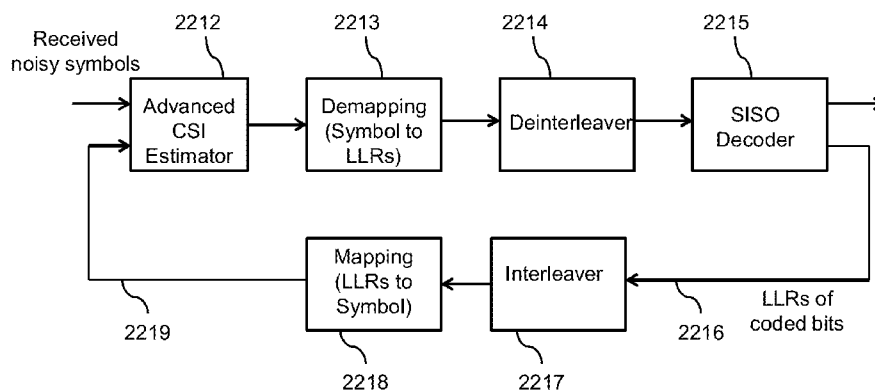
Joint, Iterative CSI Estimation and SISO Decoding
