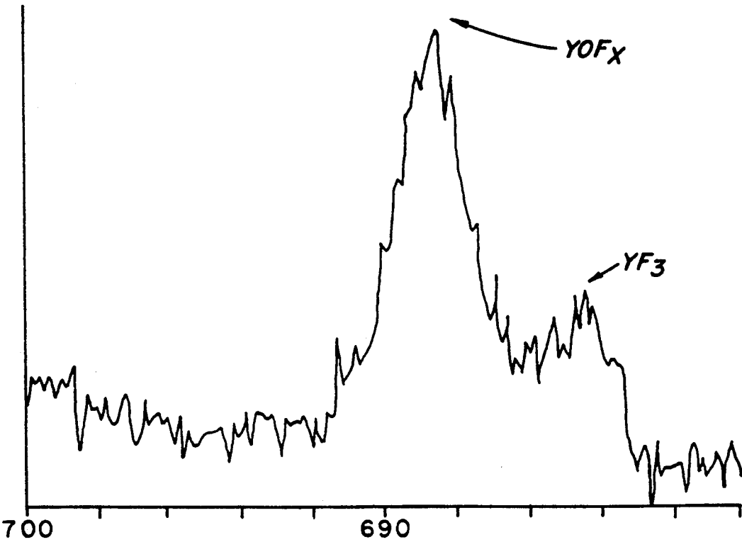
FLUORINE F 1s XPS SPECTRUM
