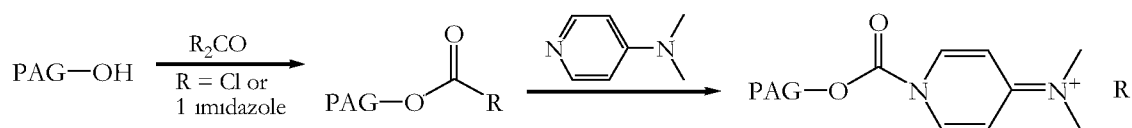
Scheme 1
