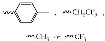
PAG sulfonates, wherein R =
