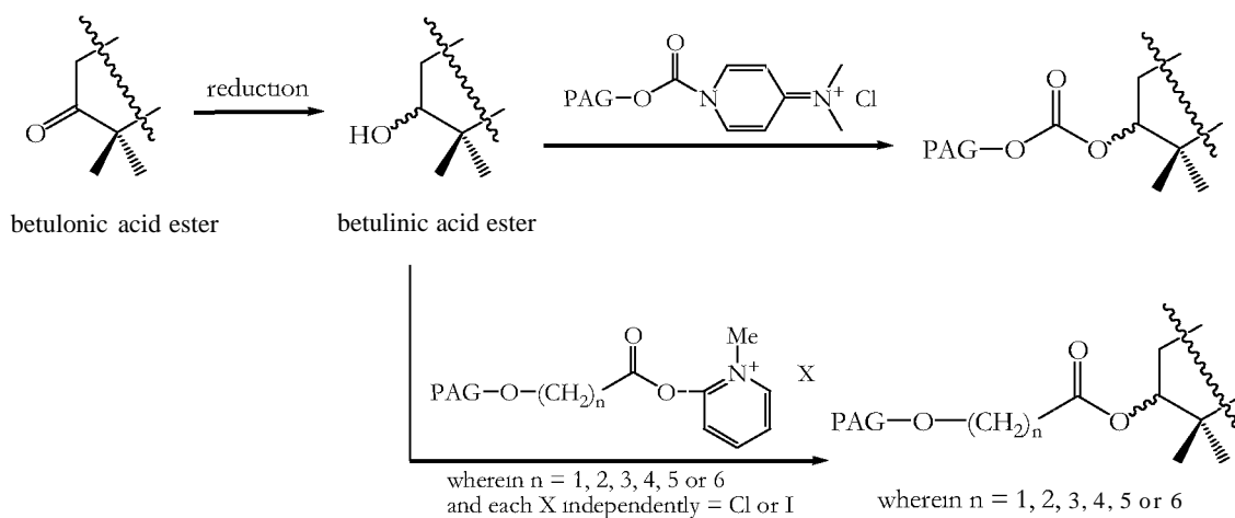
Scheme 3
