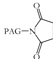
PAG maleimide derivative
