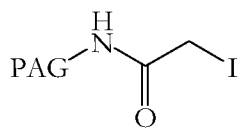
PAG iodoacetamide derivative
