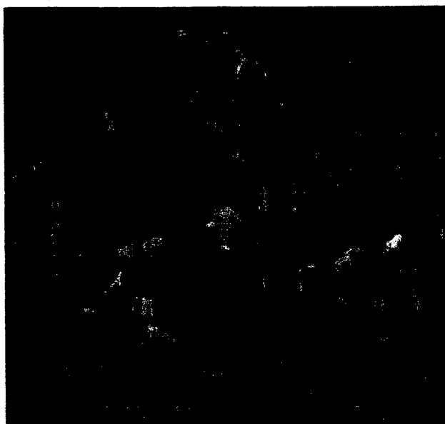
HR-TEM image
