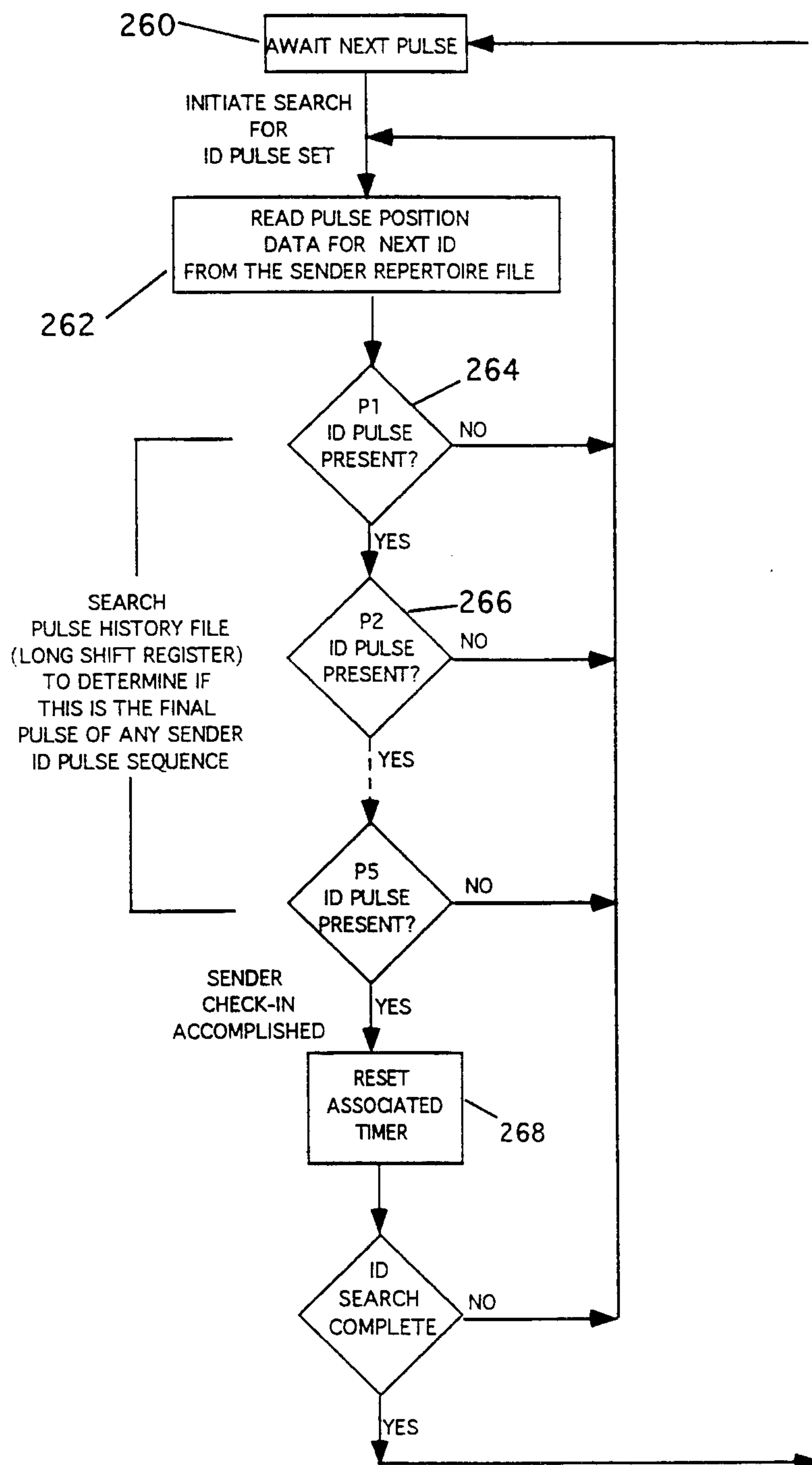
FIGURE 11 FLOW CHART, CHECK-IN SEQUENCE AT THE MONITOR FOR ONE SENDER, PULSE CODE EMBODIMENT
