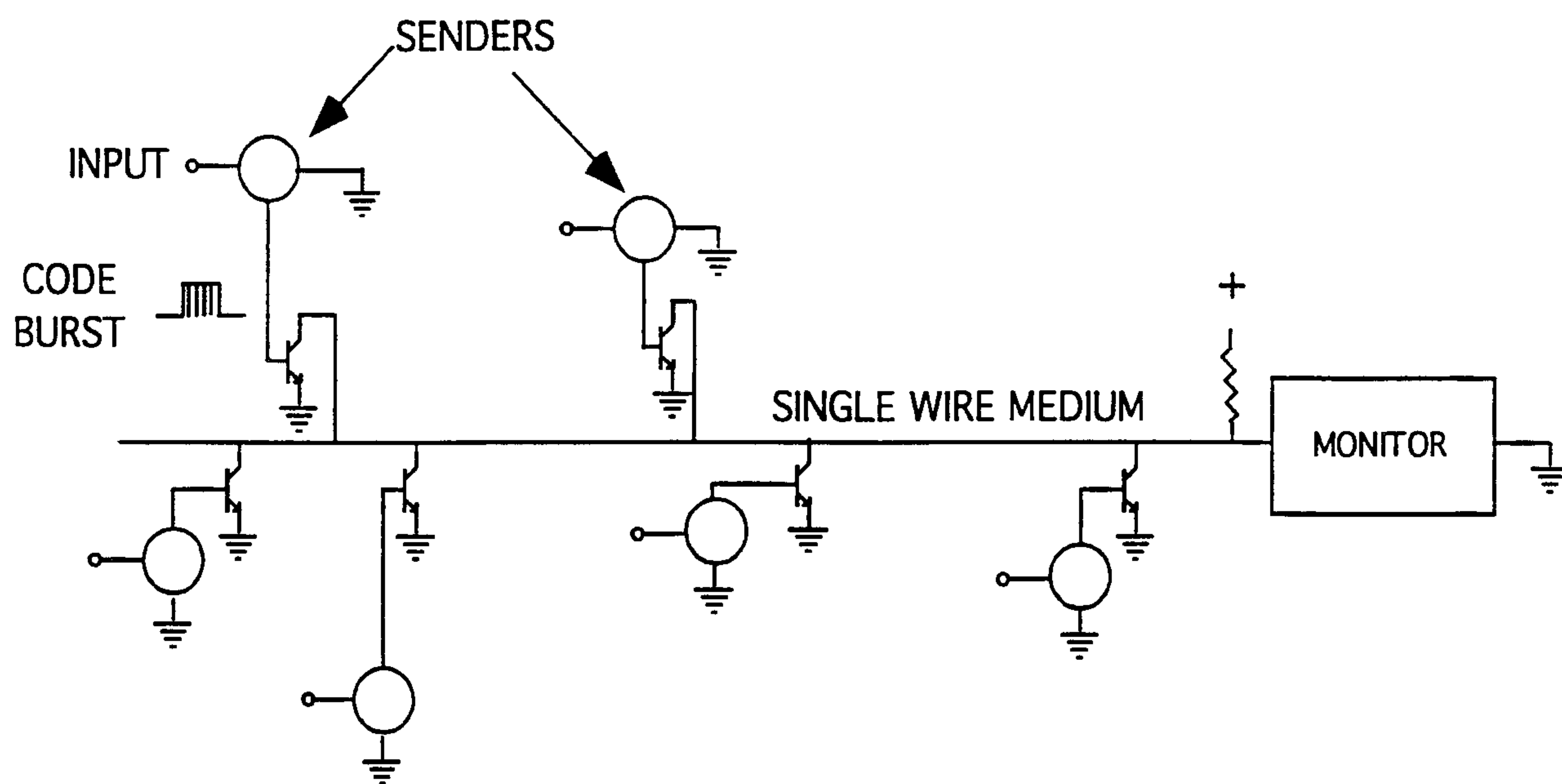
FIGURE 25 SENDERS AND MONITOR USING A SINGLE WIRE MEDIUM
