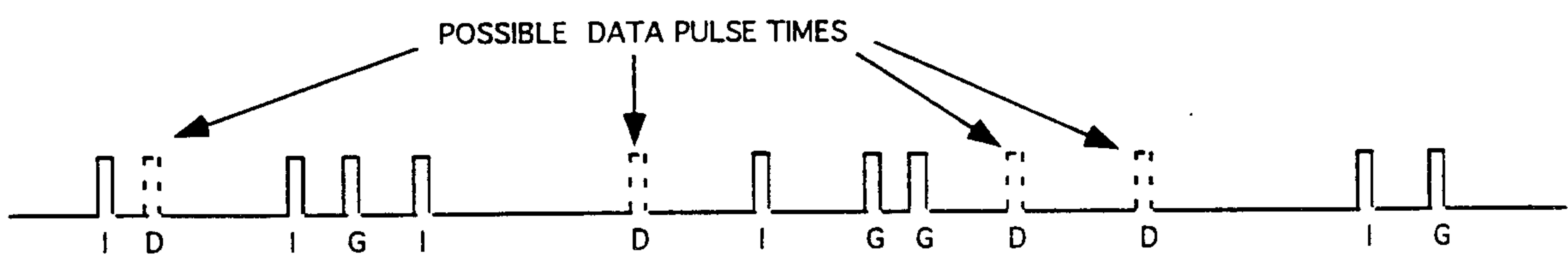
FIGURE 19 WAVEFORM WITH FOUR POSSIBLE POSITIONS FOR MULTIPLE DATA PULSES EACH INTEGRATED OVER TIME
