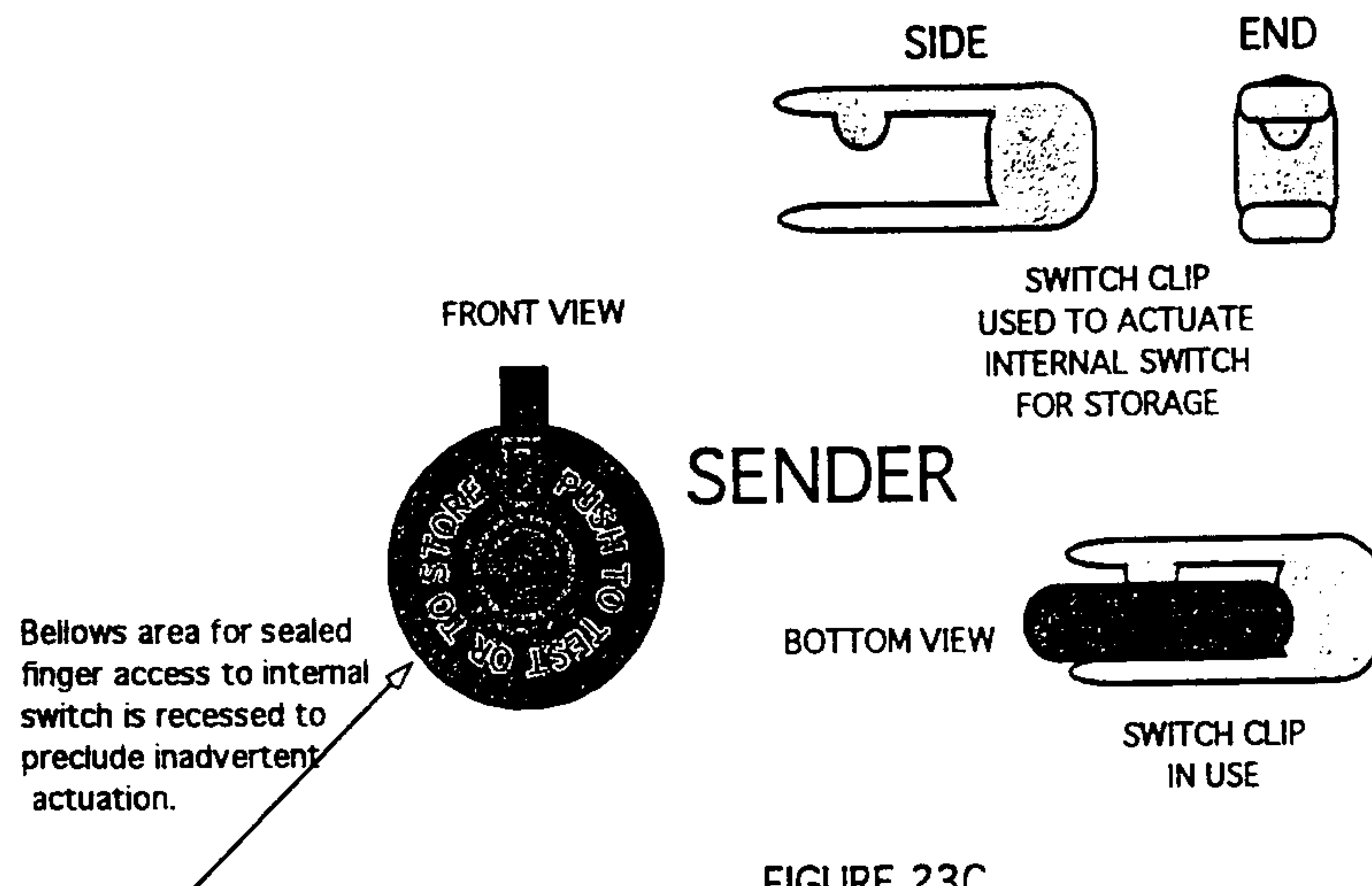
FIGURE 23C MOB SENDER WITH FINGER CONTROL OR SWITCH CLIP CONTROL OF OPERATION
