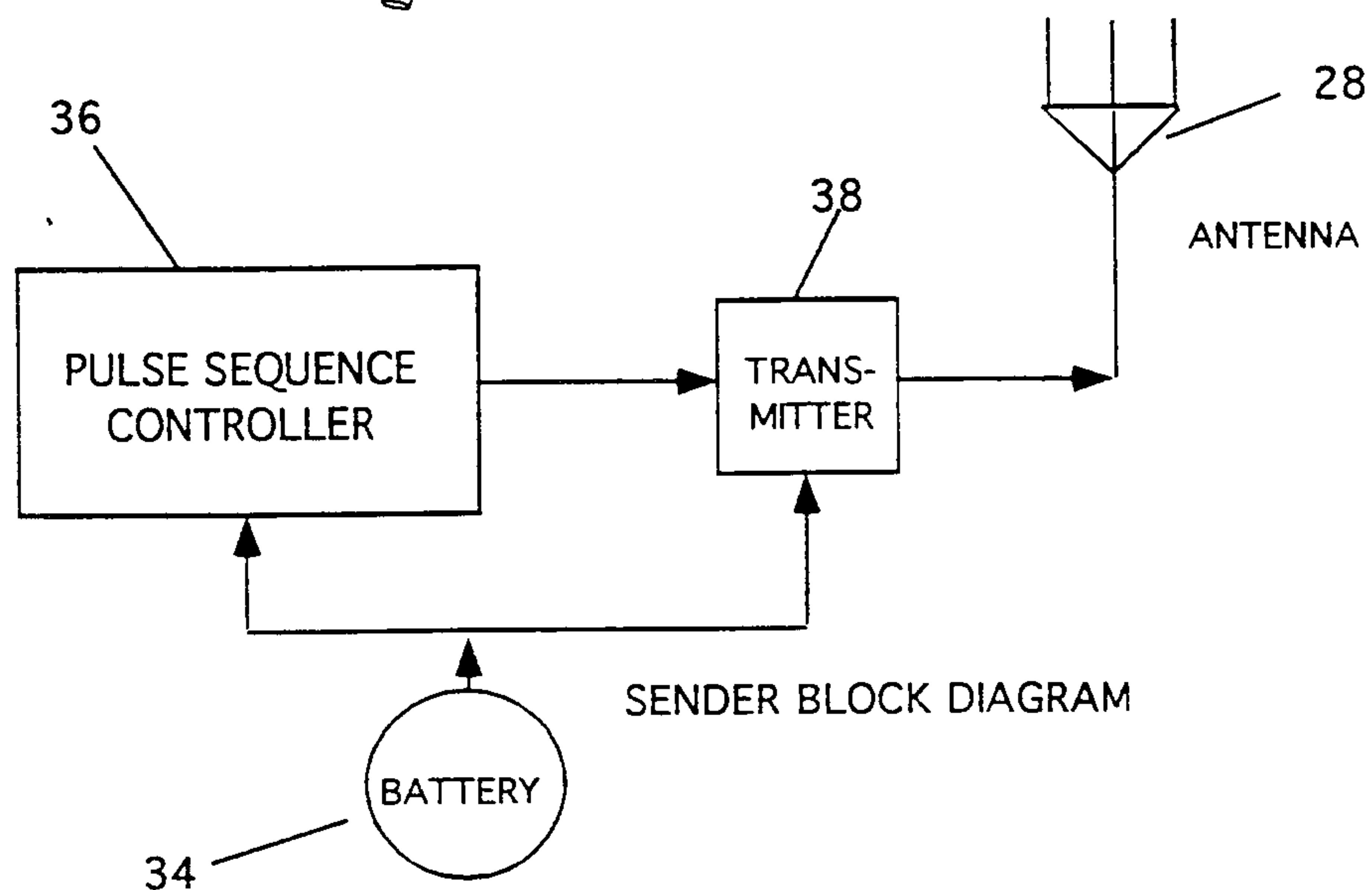
FIGURE 2B SENDER CONFIGURATION
