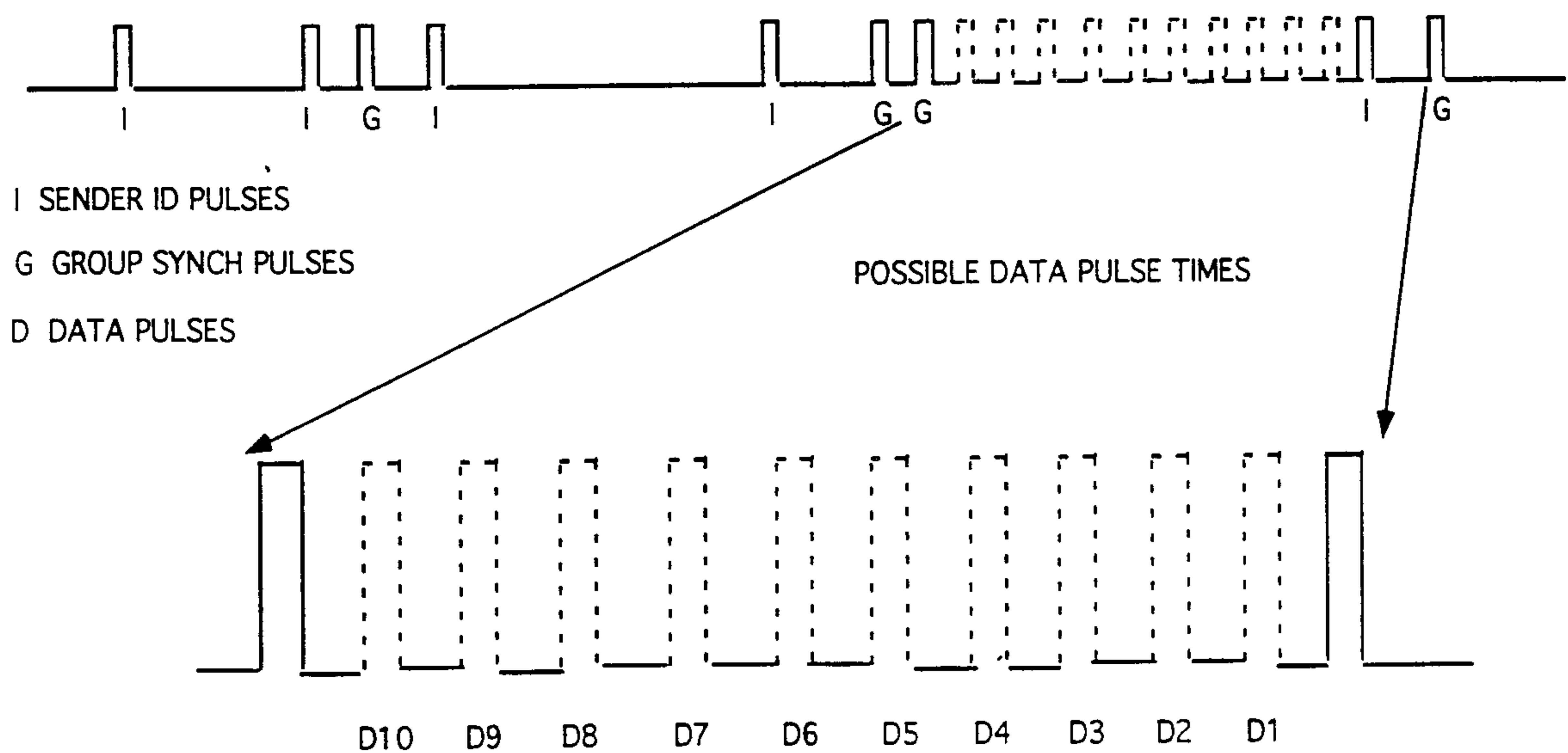
FIGURE 20 WAVEFORM WITH TEN POSSIBLE POSITIONS FOR A SINGLE DATA PULSE INTEGRATED OVER TIME
