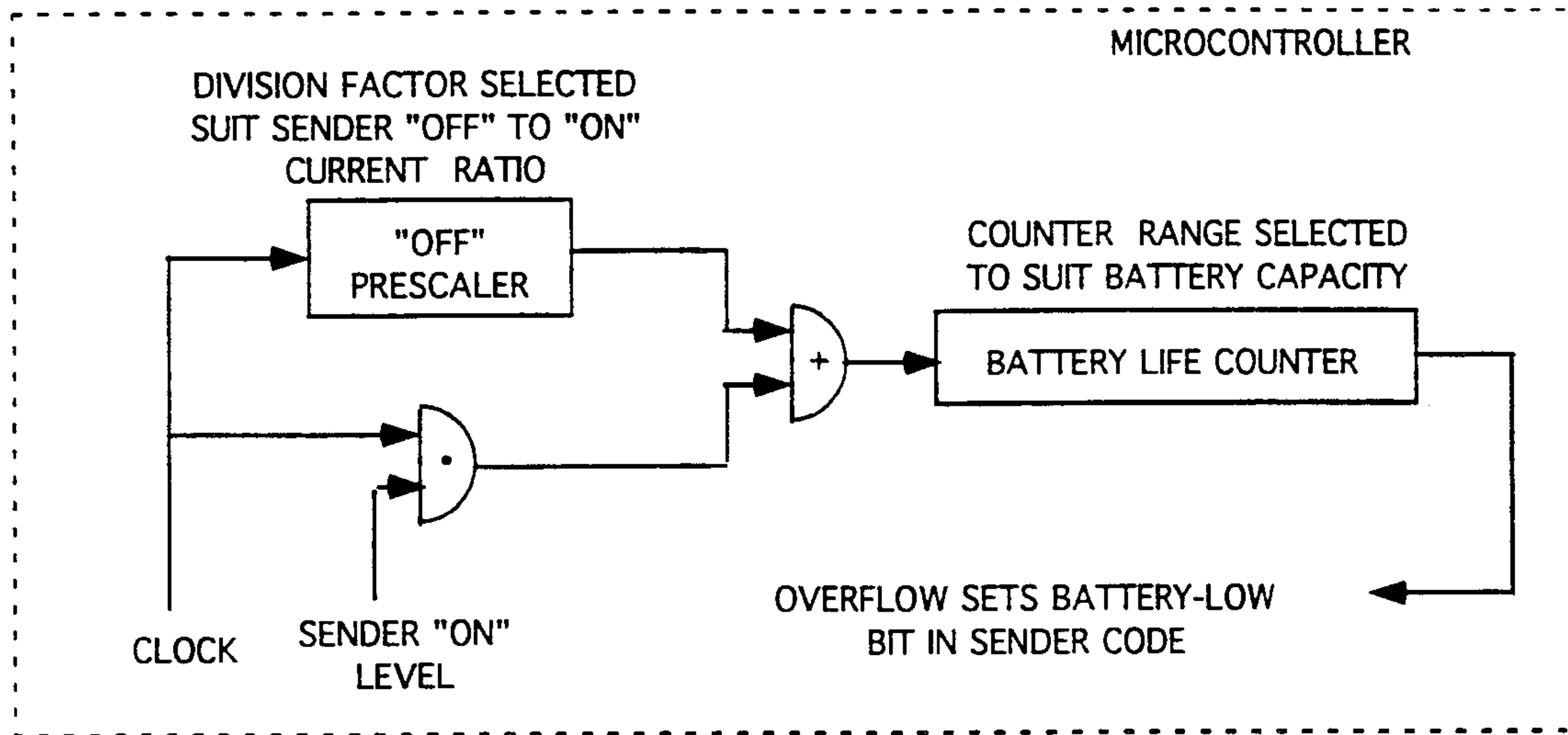
FIGURE 24A FUNCTIONAL BLOCK DIAGRAM, METHOD OF LOGGING SENDER'S BATTERY USE, PREDICTING IT'S END-OF-LIFE, AND REPORTING VIA THE BATTERY STATUS BIT
