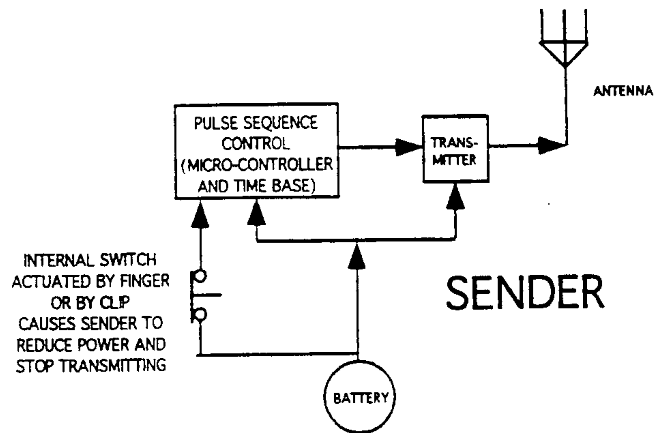
FIGURE 23B FUNCTIONAL BLOCK DIAGRAM, SENDER WITH SWITCH ACTUATED MODE CONTROL
