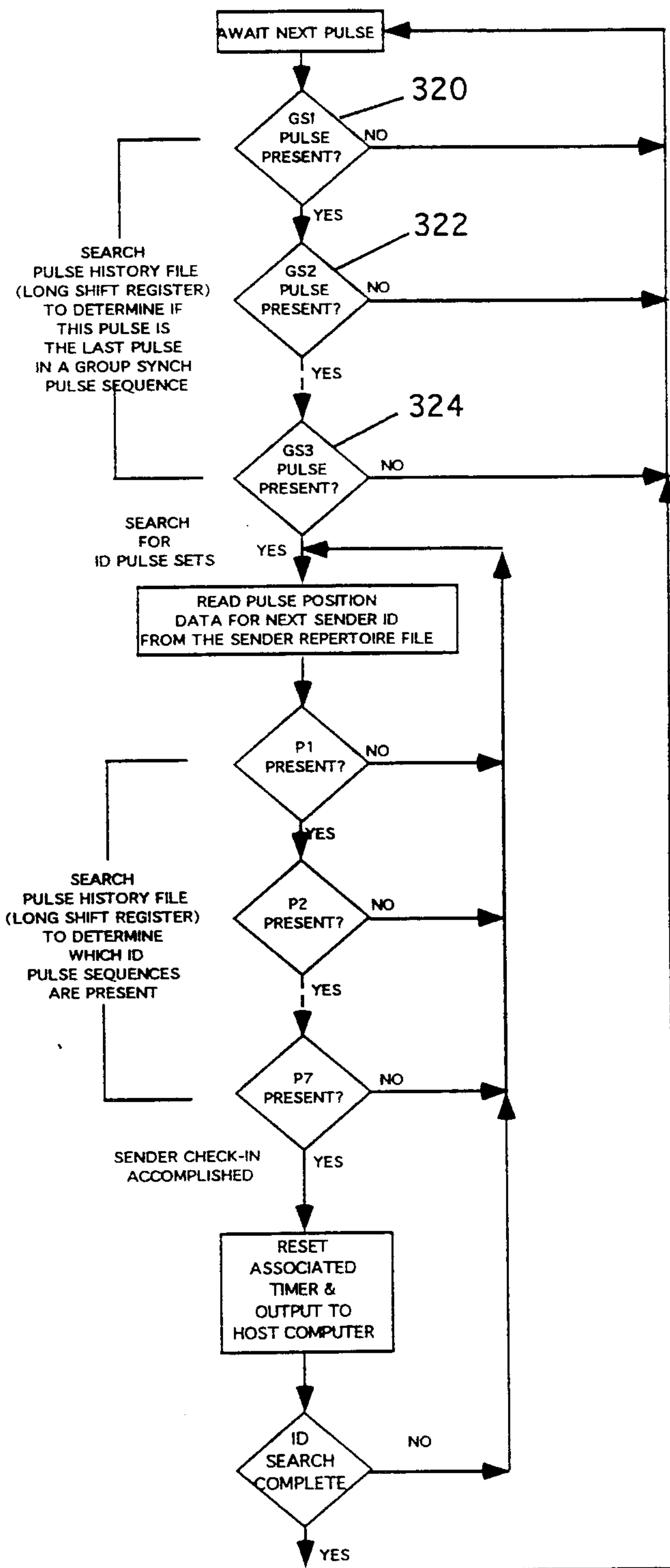
FIGURE 14 FLOW CHART, CHECK-IN SEQUENCE AT THE MONITOR FOR ONE SENDER, GROUP SYNCH EMBODIMENT
