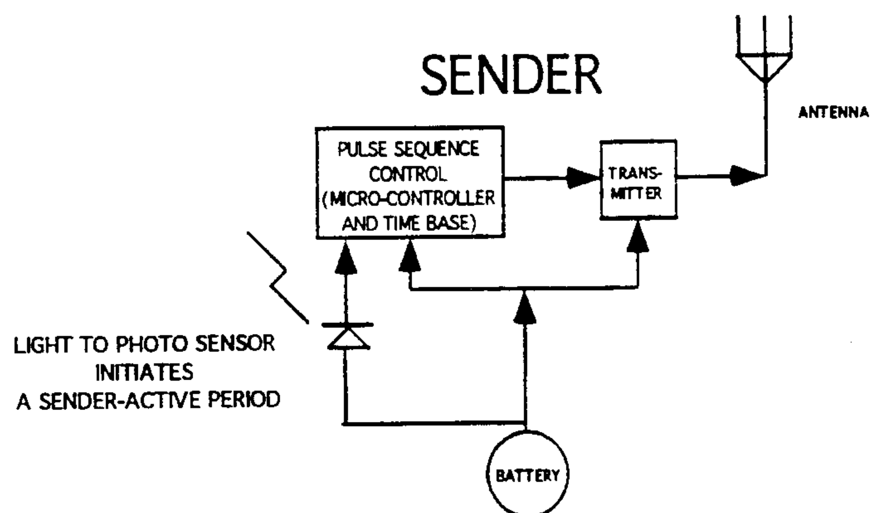
FIGURE 23D FUNCTIONAL BLOCK DIAGRAM, SENDER WITH PHOTO SENSOR TO CONTROL ON/OFF OPERATION
