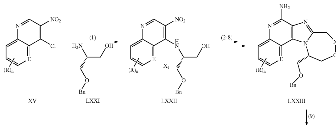
Reaction Scheme XI
