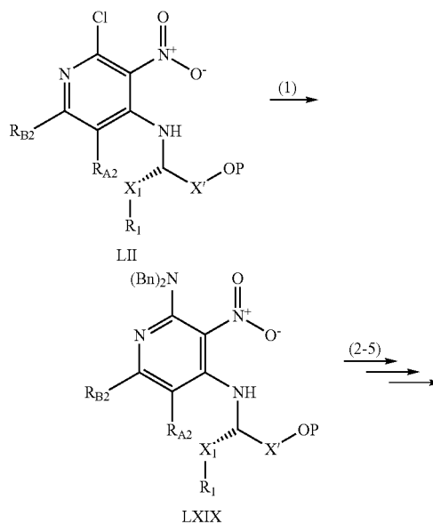
Reaction Scheme X
