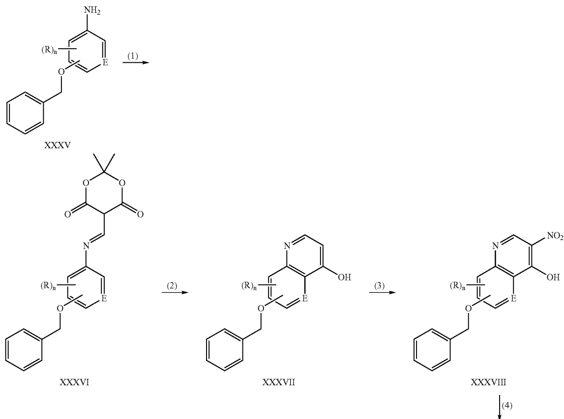
Reaction Scheme IV
