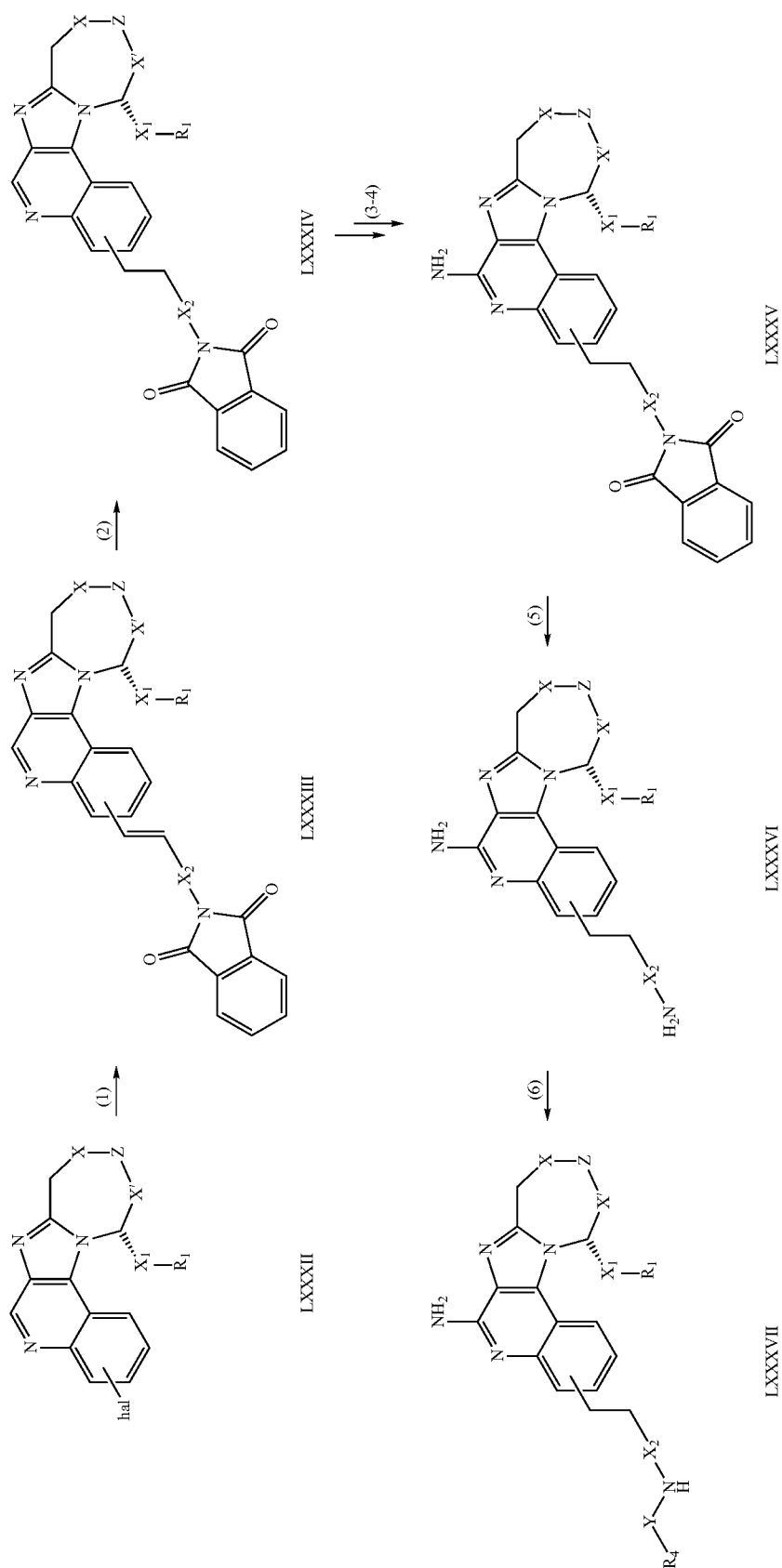
Reaction Scheme XIV
