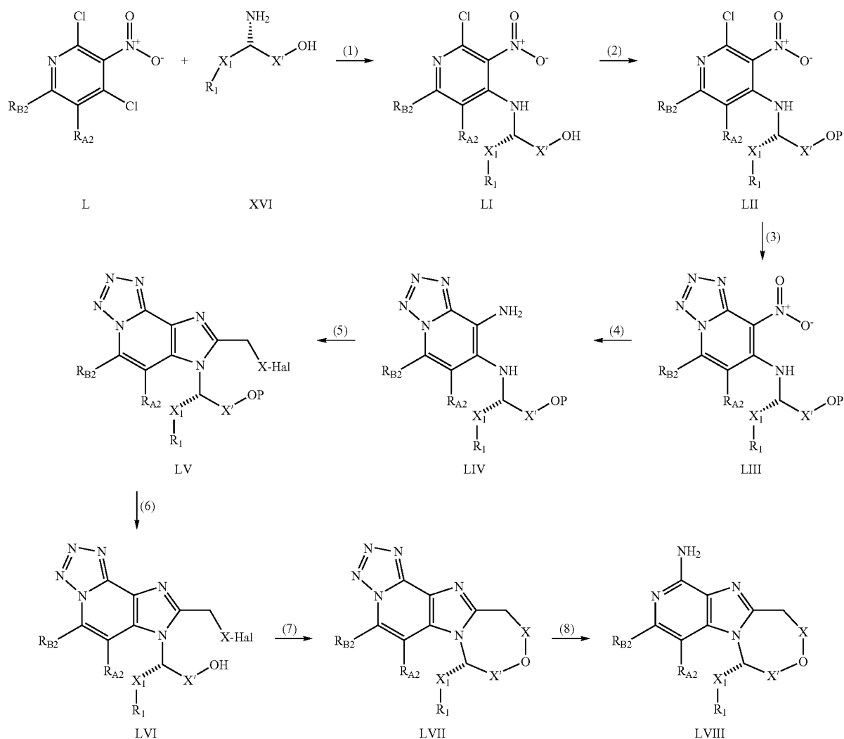
Reaction Scheme V
