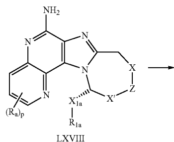
Reaction Scheme IX
