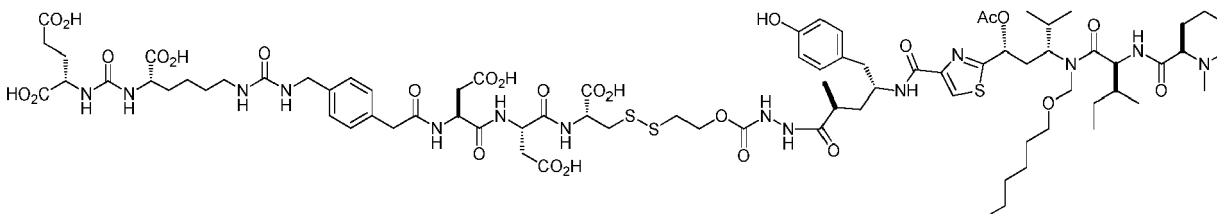
EC1720 (C80H118N14O27S3, Exact Mass: 1802.75, Mol. Wt.: 1804.07)
