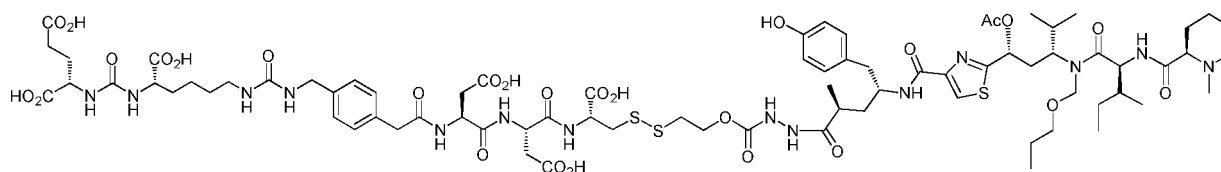
EC1718 ( C_{77}H_{112}N_{14}O_{27}S_3 , Exact Mass: 1760.70, Mol. Wt.: 1761.99)
