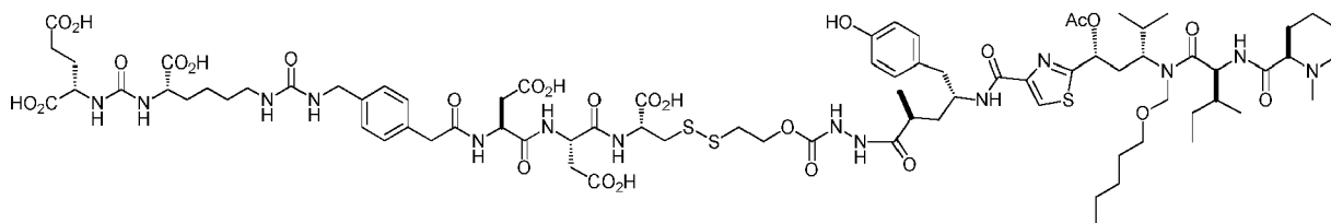
EC1719 (C79H116N14O27S3, Exact Mass: 1788.73, Mol. Wt.: 1790.04)
