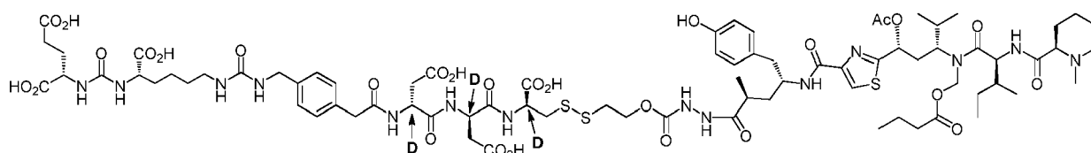
EC1584 ( C_{78}H_{112}N_{14}O_{28}S_3 , Exact Mass: 1788.69, Mol. Wt.: 1790.00)
