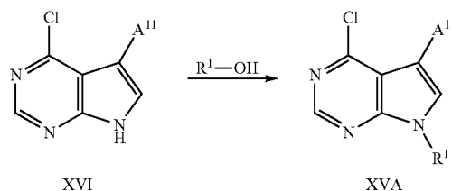
Scheme 32
