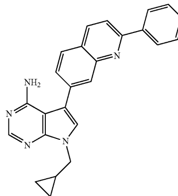
7-Cyclopropylmethyl-5-(2-phenylquinolin-7-yl)-7H-pyrrolo[2,3-d]pyrimidin-4-ylamine
