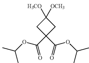
3,3-Dimethoxy-cyclobutane-1,1-dicarboxylic acid diisopropyl ester
