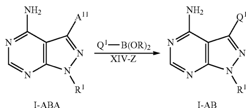
Scheme 28
