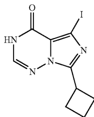
7-Cyclobutyl-5-iodo-3H-imidazo[5,1-f][1,2,4]triazin-4-one
