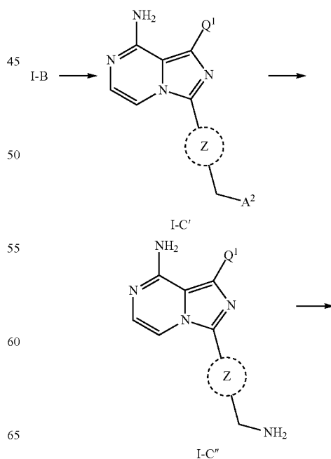
Scheme 21
