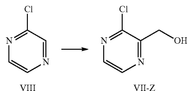
Scheme 13
