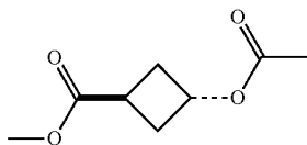
trans-3-Acetoxycyclobutanecarboxylic acid methyl ester
