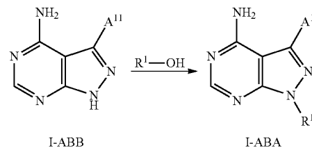
Scheme 29
