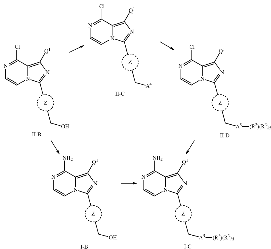
Scheme 20
