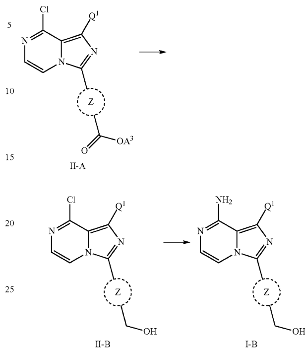
Scheme 19
