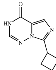
7-Cyclobutyl-3H-imidazo[5,1-f][1,2,4]triazin-4-one
