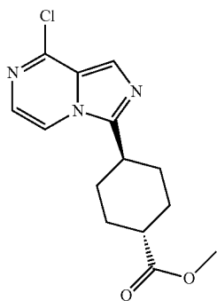
trans-Methyl 4-(8-chloroimidazo[1,5-a]pyrazin-3-yl)cyclohexanecarboxylate
