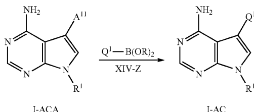
Scheme 30
