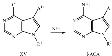
Scheme 31
