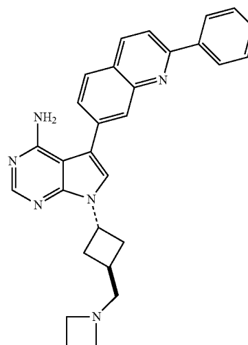
7-(trans-3-Azetidin-1-ylmethylcyclobutyl)-5-(2-phenylquinolin-7-yl)-7H-pyrrolo[2,3-d]pyrimidin-4-ylamine
