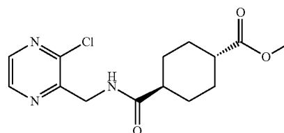
trans-Methyl 4-({[(3-chloropyrazin-2-yl)methyl]amino}carbonyl)cyclohexanecarboxylate
