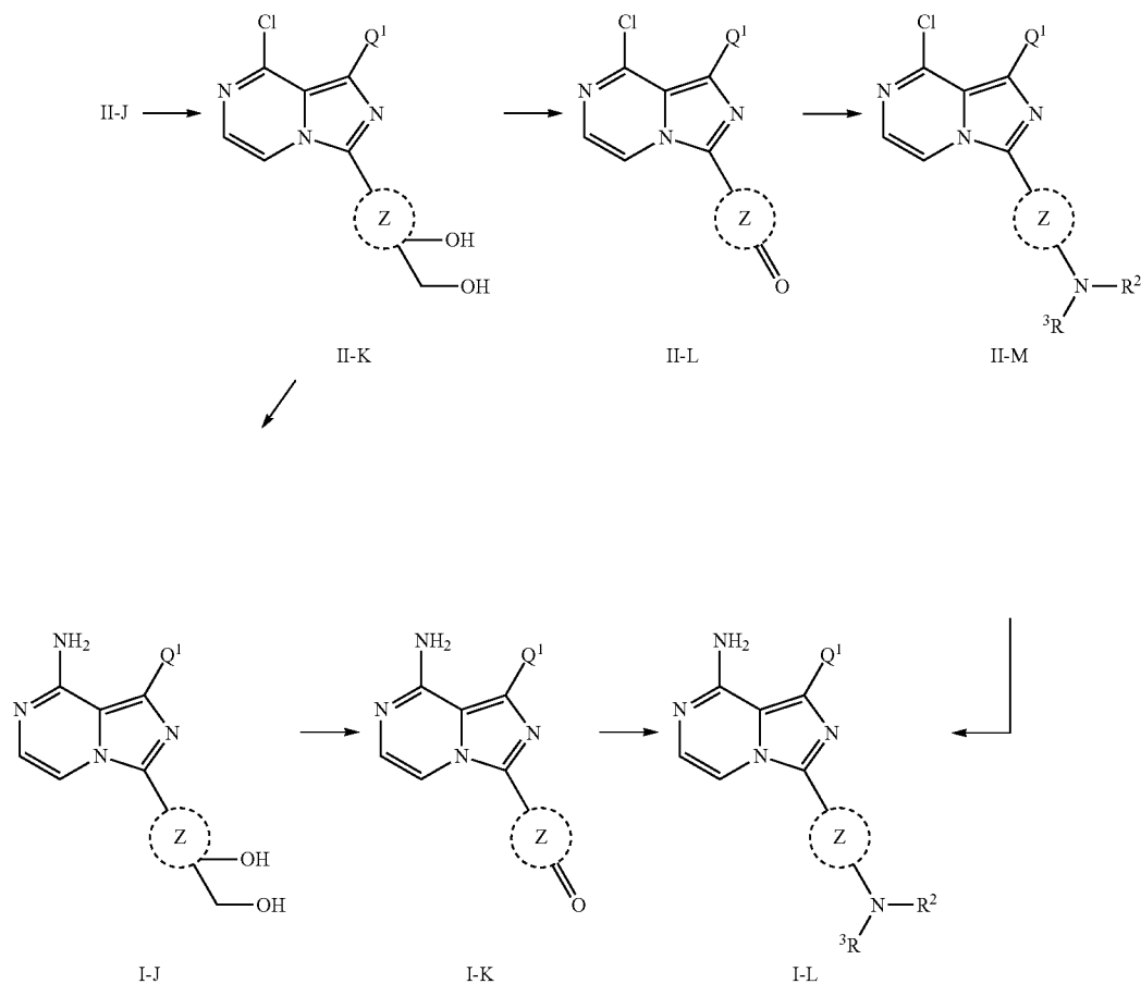
Scheme 25
