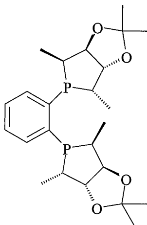
(S,S,S,S)-"Me-KetalPhos",
