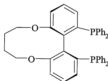
(S)-"C4-TunePhos",
