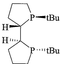
( R,R,S,S )-"TangPhos",
