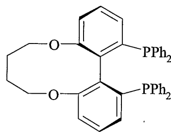
( S )-"C4-TunePhos",
