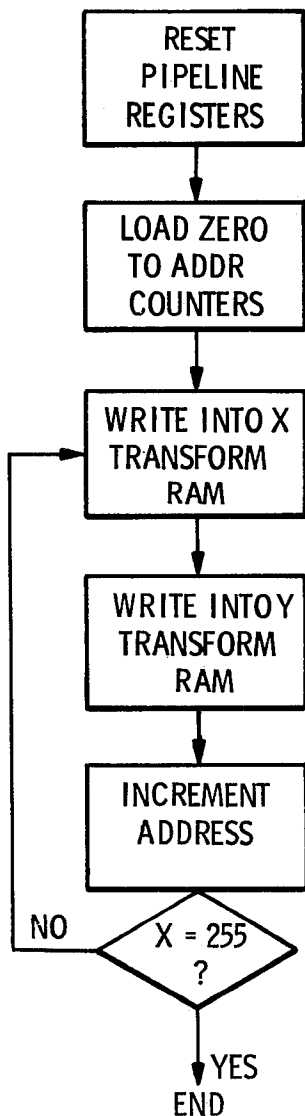
LOADING TRANSFORM RAM-FLOW CHART
