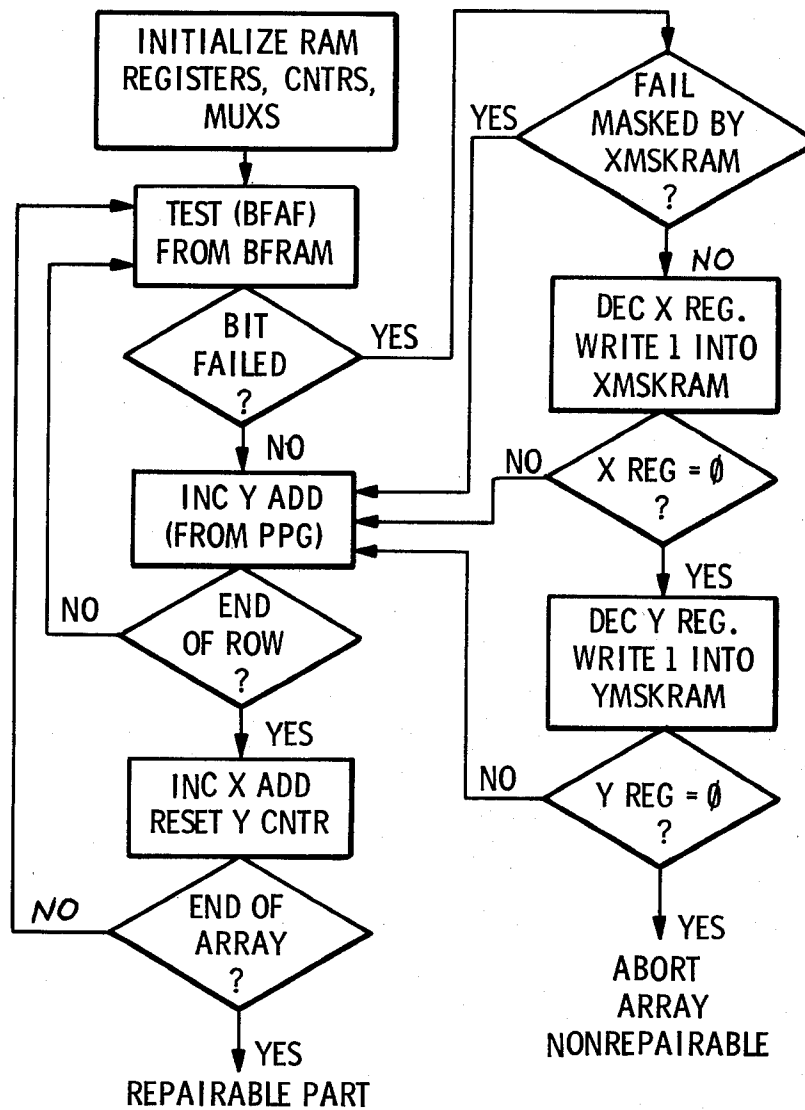
FLOW CHART OF 3rd PASS ALGORITHM
