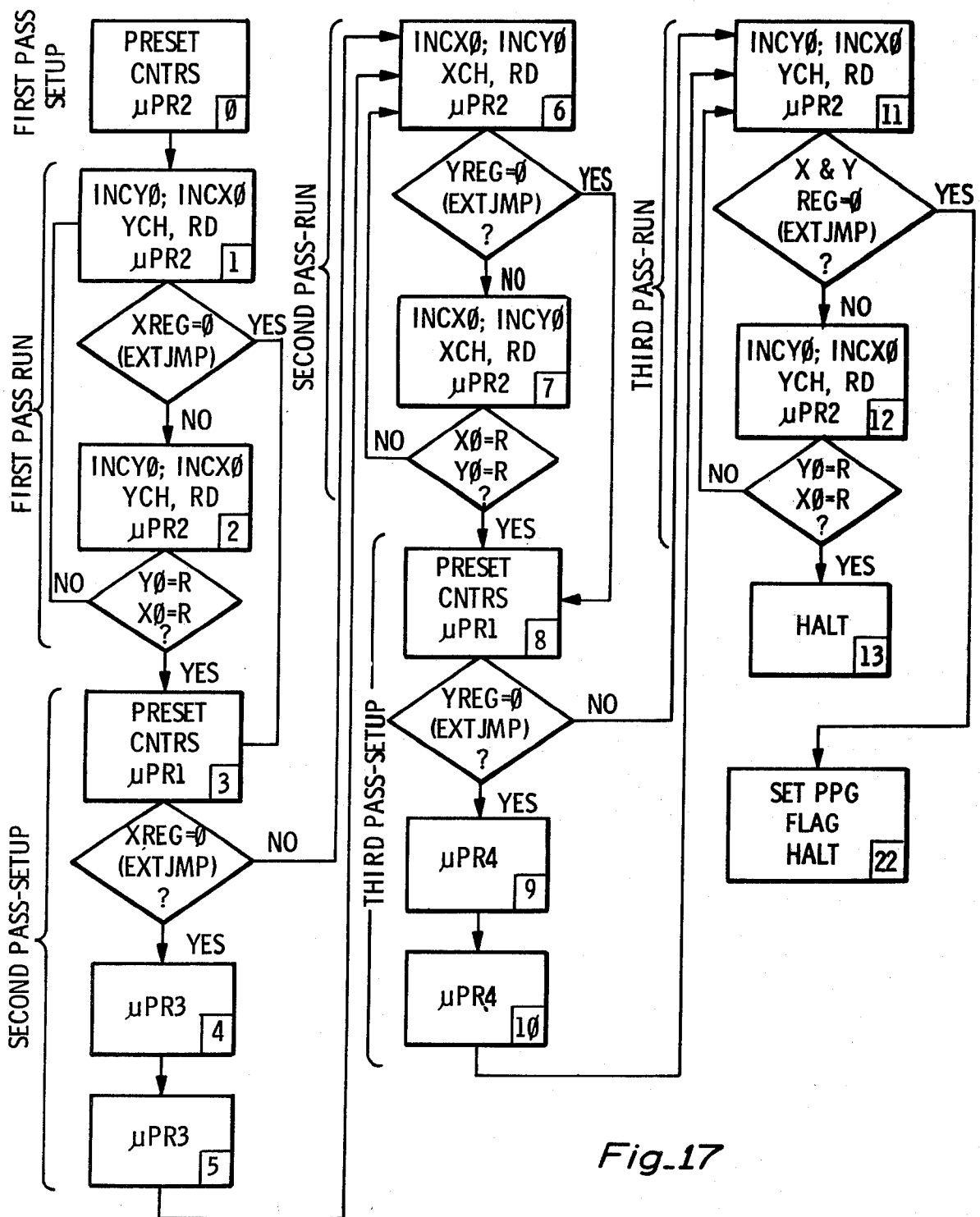
PATTERN GENERATOR LOGIC FLOW CHART
