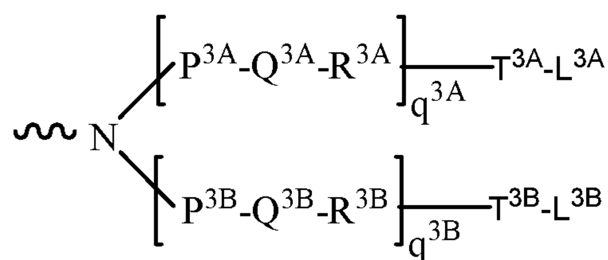
Formula (III)
