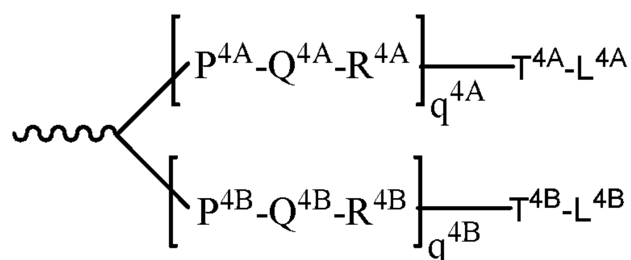
Formula (IV)
