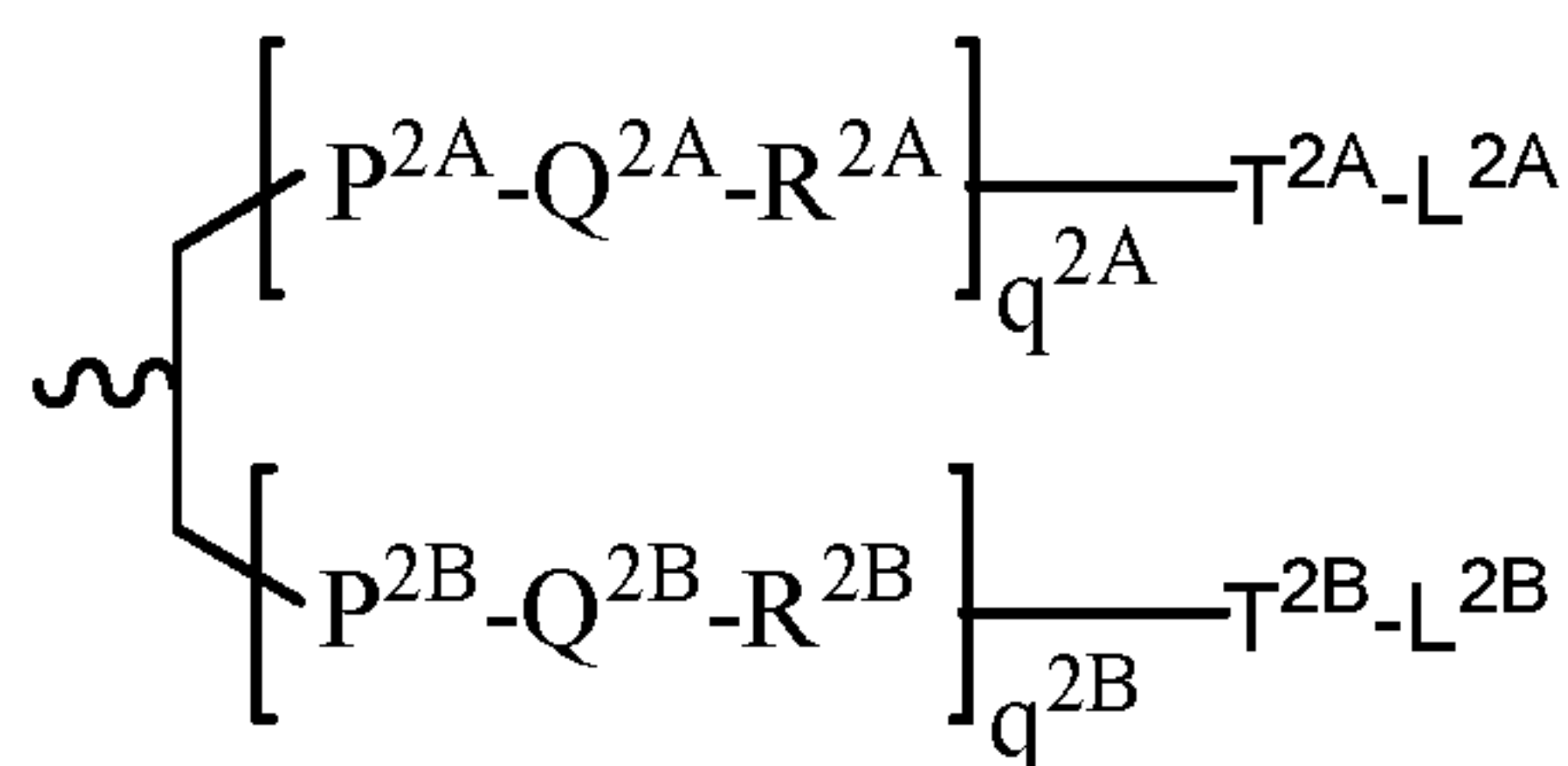
Formula (II)
