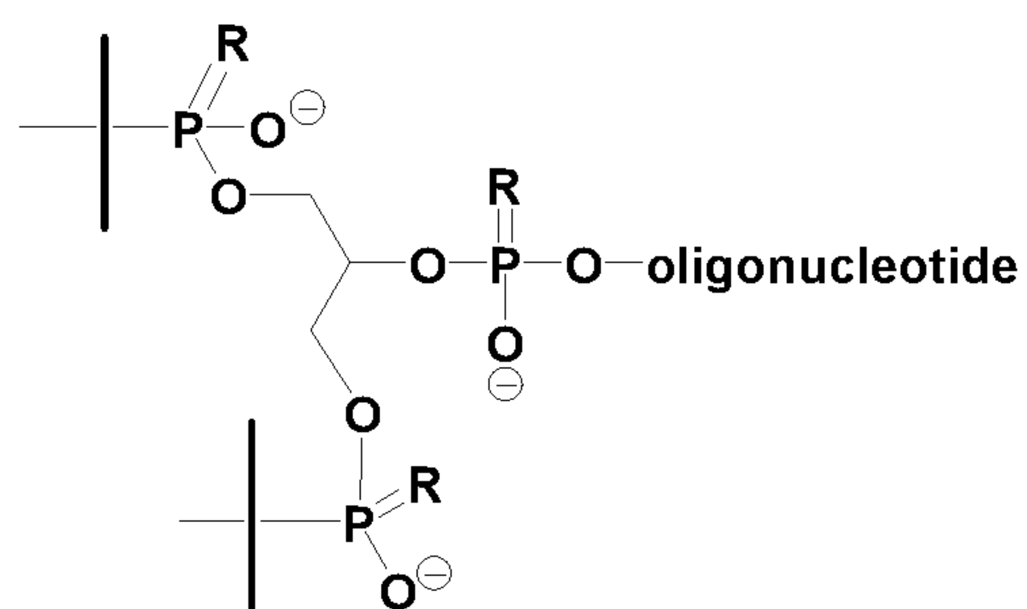
Formula (VII)
