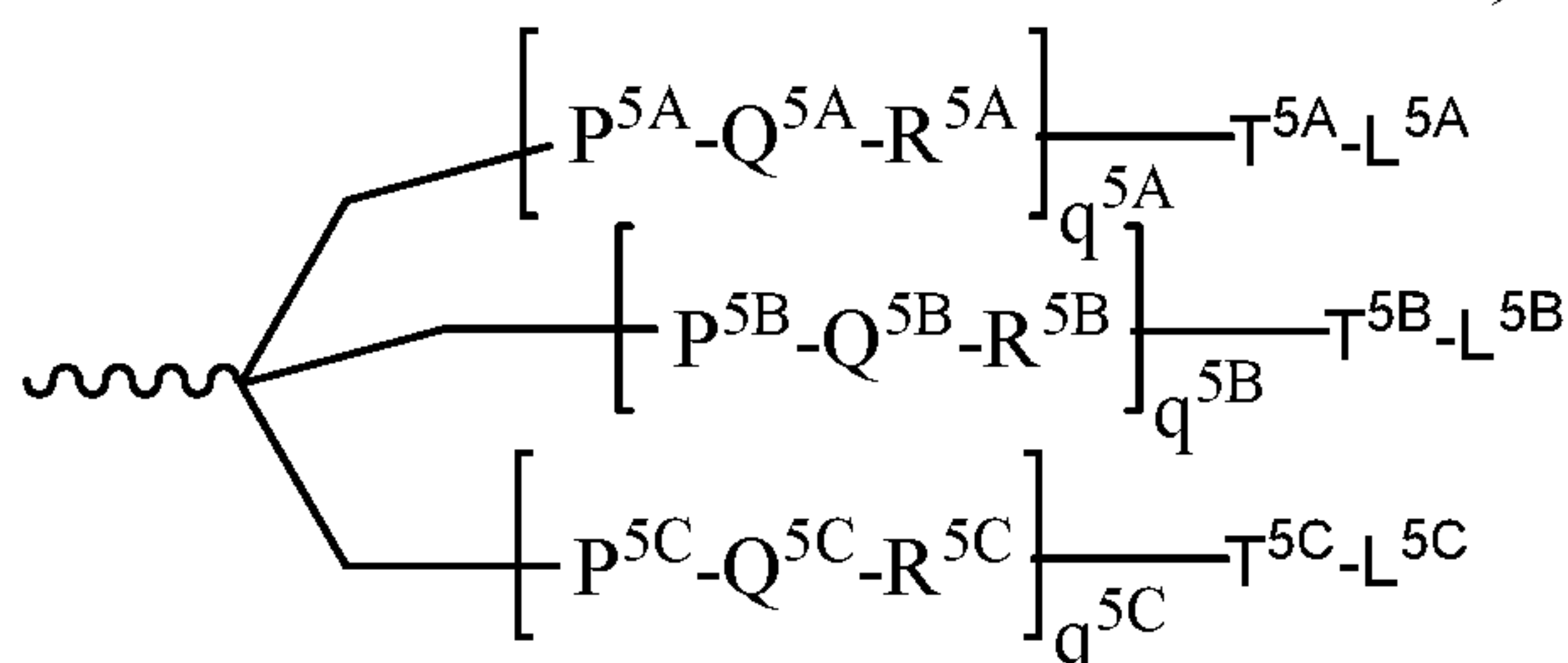
Formula (V)
