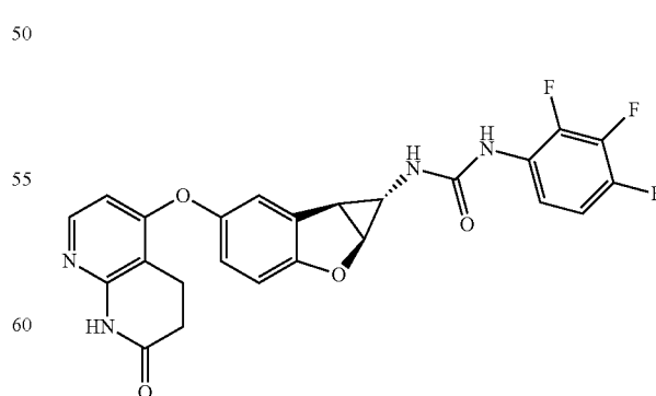
Compound 1.46
