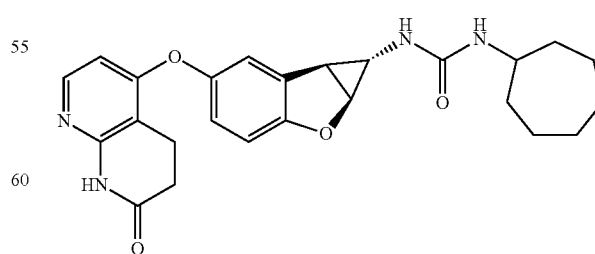
Compound 1.52
