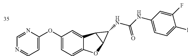
Compound 2.3
