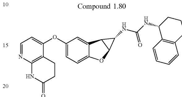
Compound 1.80
