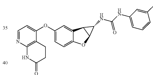
Compound 1.22
