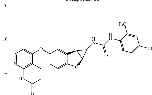
Compound 1.9
