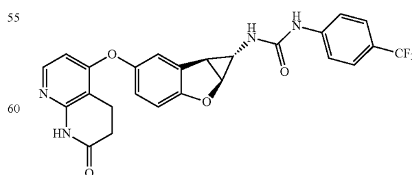
Compound 1.29
