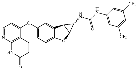
Compound 1.65
