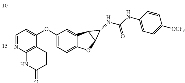
Compound 1.61
