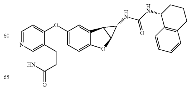
Compound 1.80
