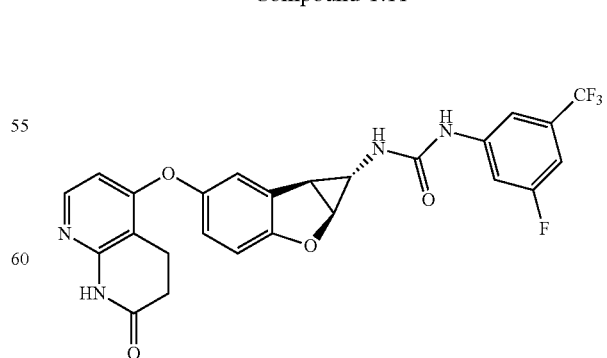
Compound 1.11
