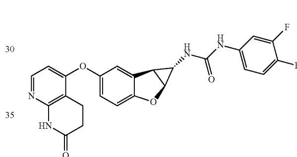
Compound 1.45
