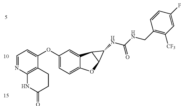
Compound 1.77
