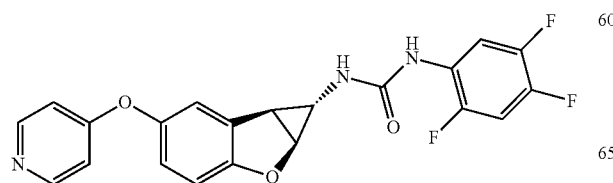
Compound 2.10
