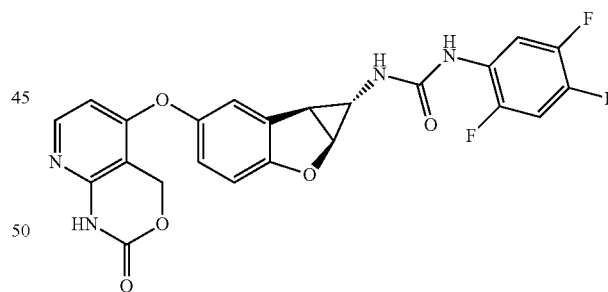
Compound 2.3
