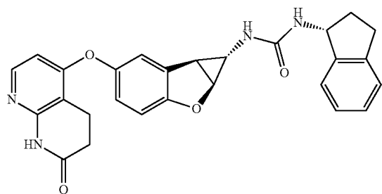
Compound 1.82
