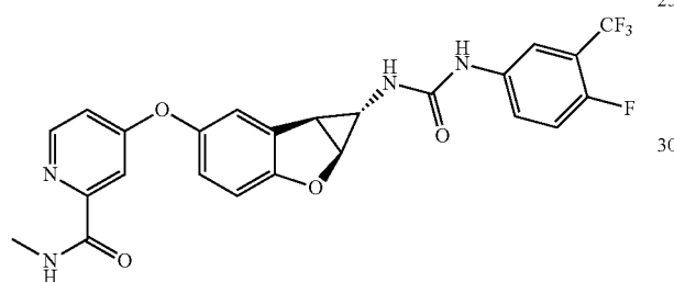
Compound 2.7
