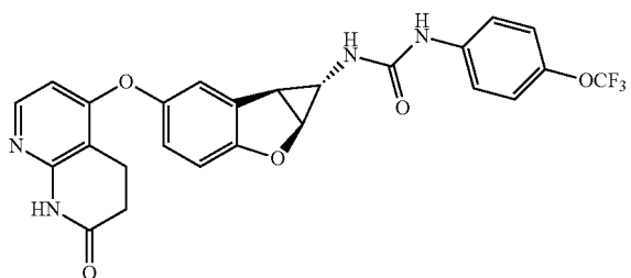
Compound 1.62
