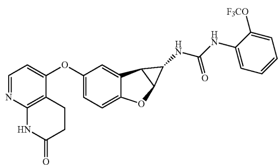
Compound 1.63
