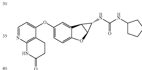
Compound 1.51
