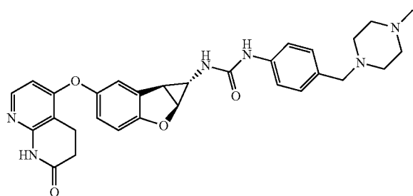
Compound 1.63
