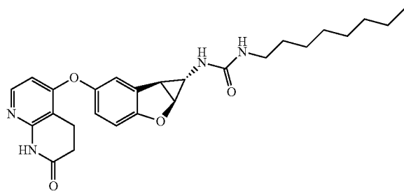
Compound 1.84
