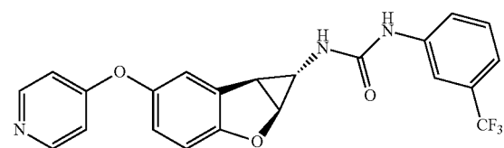
Compound 2.12
