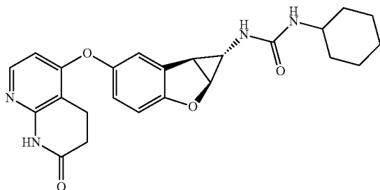
Compound 1.66
