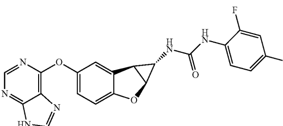
Compound 2.14
