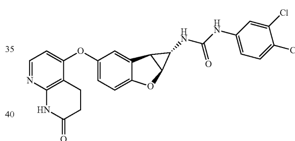
Compound 1.28
