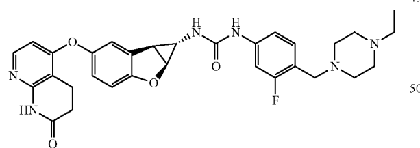
Compound 1.74
