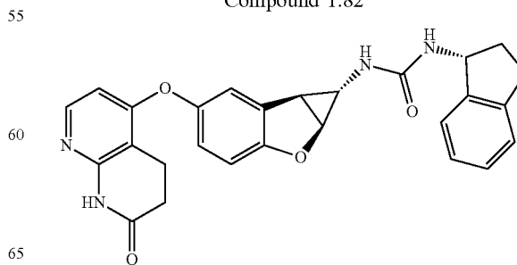
Compound 1.82
