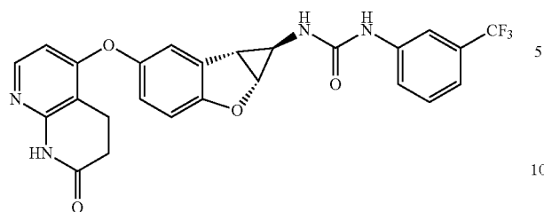
Compound 1.71
