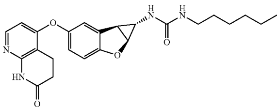
Compound 1.78
