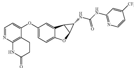
Compound 1.2
