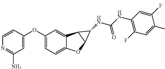
Compound 2.16
