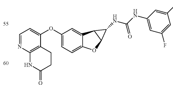
Compound 1.23
