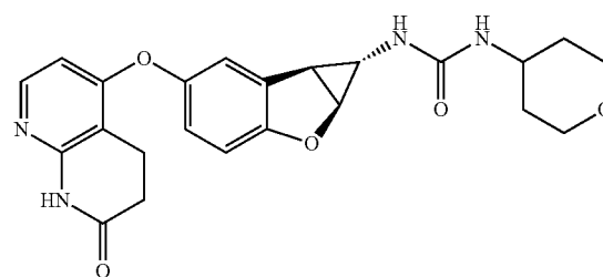
Compound 1.67
