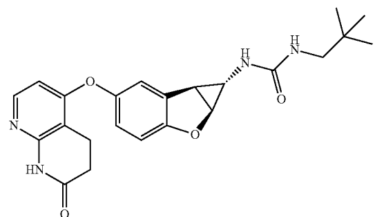
Compound 1.83
