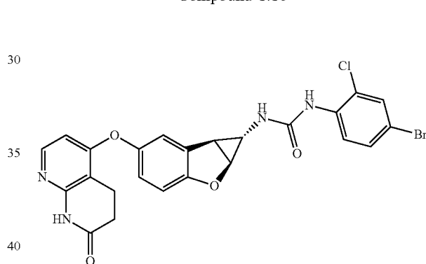
Compound 1.10
