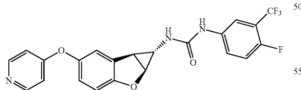
Compound 2.9
