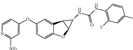
Compound 2.15
