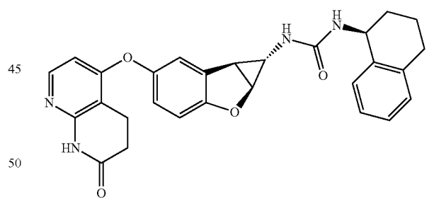
Compound 1.79
