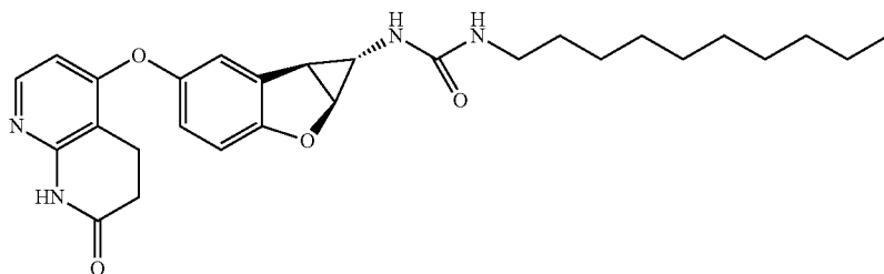
Compound 1.85
