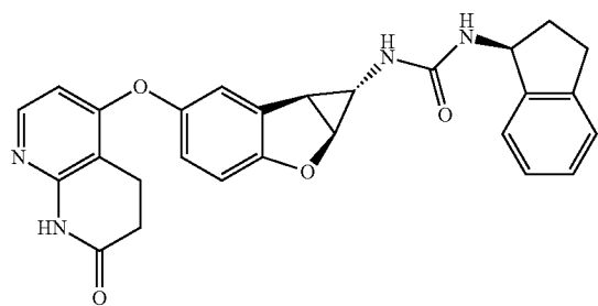
Compound 1.82
