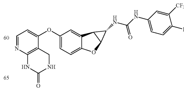
Compound 2.4
