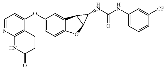
Compound 1.2
