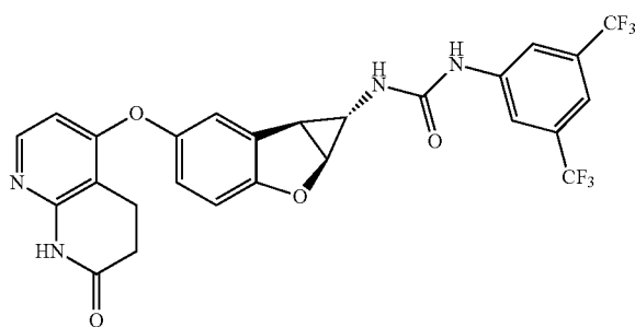
Compound 1.65
