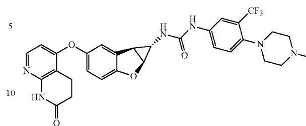
Compound 1.87
