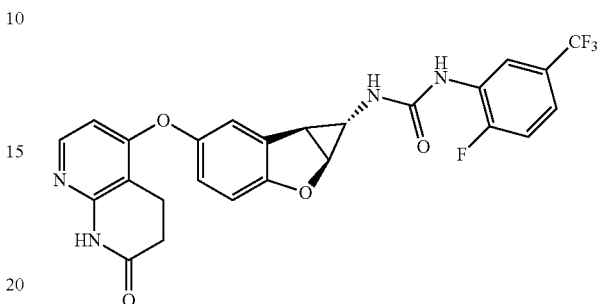
Compound 1.33
