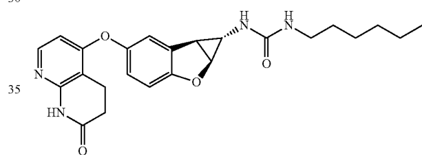
Compound 1.78
