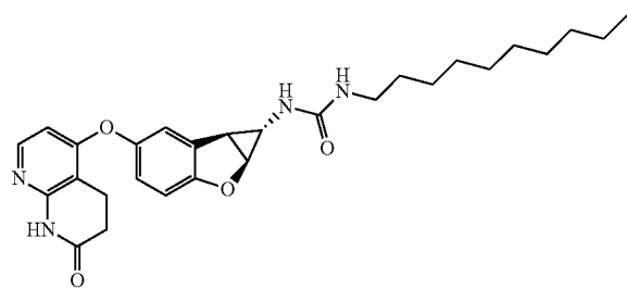
Compound 1.85
