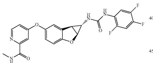
Compound 2.8
