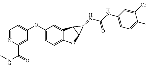
Compound 2.16
