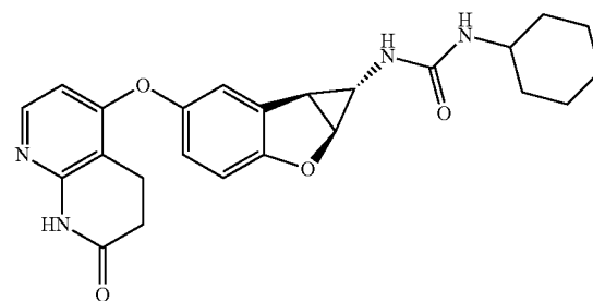
Compound 1.67
