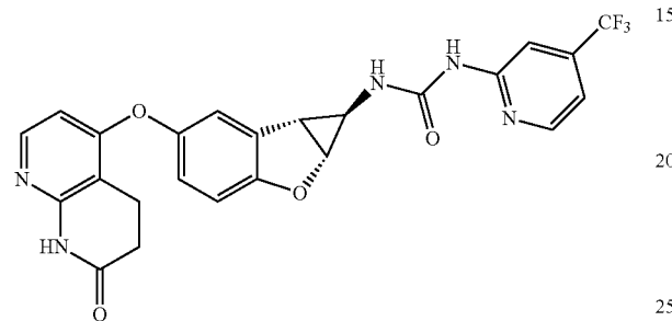
Compound 1.72
