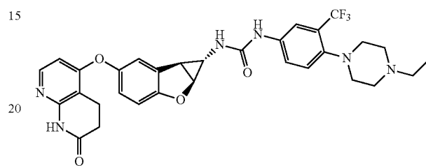
Compound 2.1
