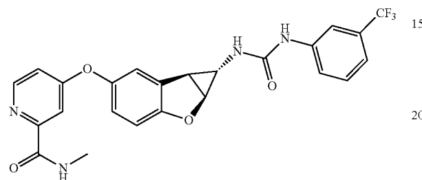
Compound 2.7
