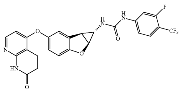
Compound 1.64
