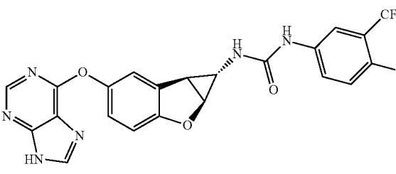
Compound 2.13
