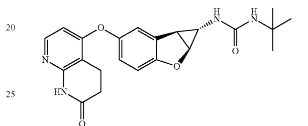
Compound 1.77
