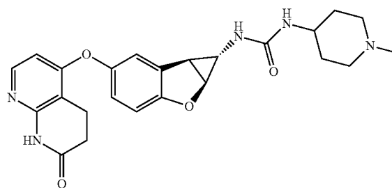
Compound 1.68
