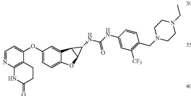
Compound 1.73
