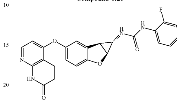
Compound 1.21
