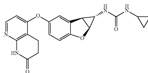
Compound 1.69
