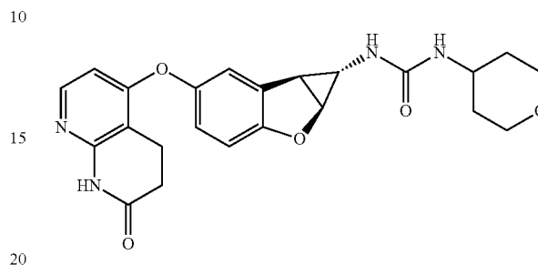
Compound 1.67
