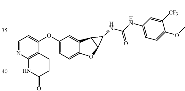
Compound 1.34
