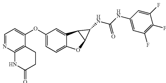
Compound 1.47
