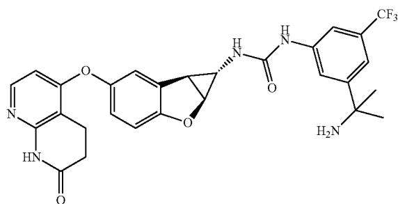
Compound 1.70
