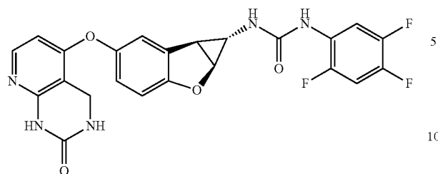
Compound 2.6
