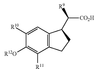
Figure 2. anti diastereomers of Formula V
