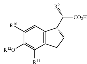
Figure 1. syn diastereomers of Formula V
