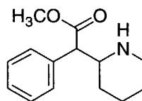
Methylphenidate
