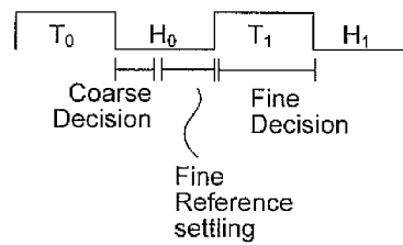
Fig. 2 (Prior Art)
