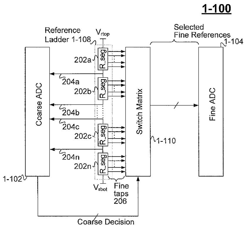
Fig. 3 (Prior Art)
