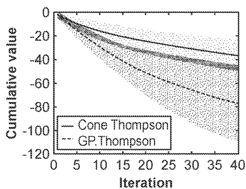
Results of optimization of f_1 .
