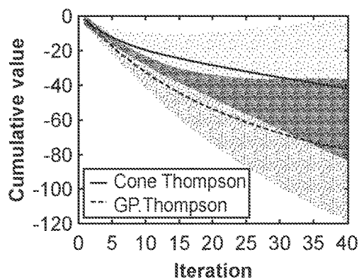
Results of optimization of f_2 .
