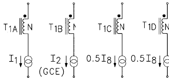
SEPIC FED BUCK (MC)
