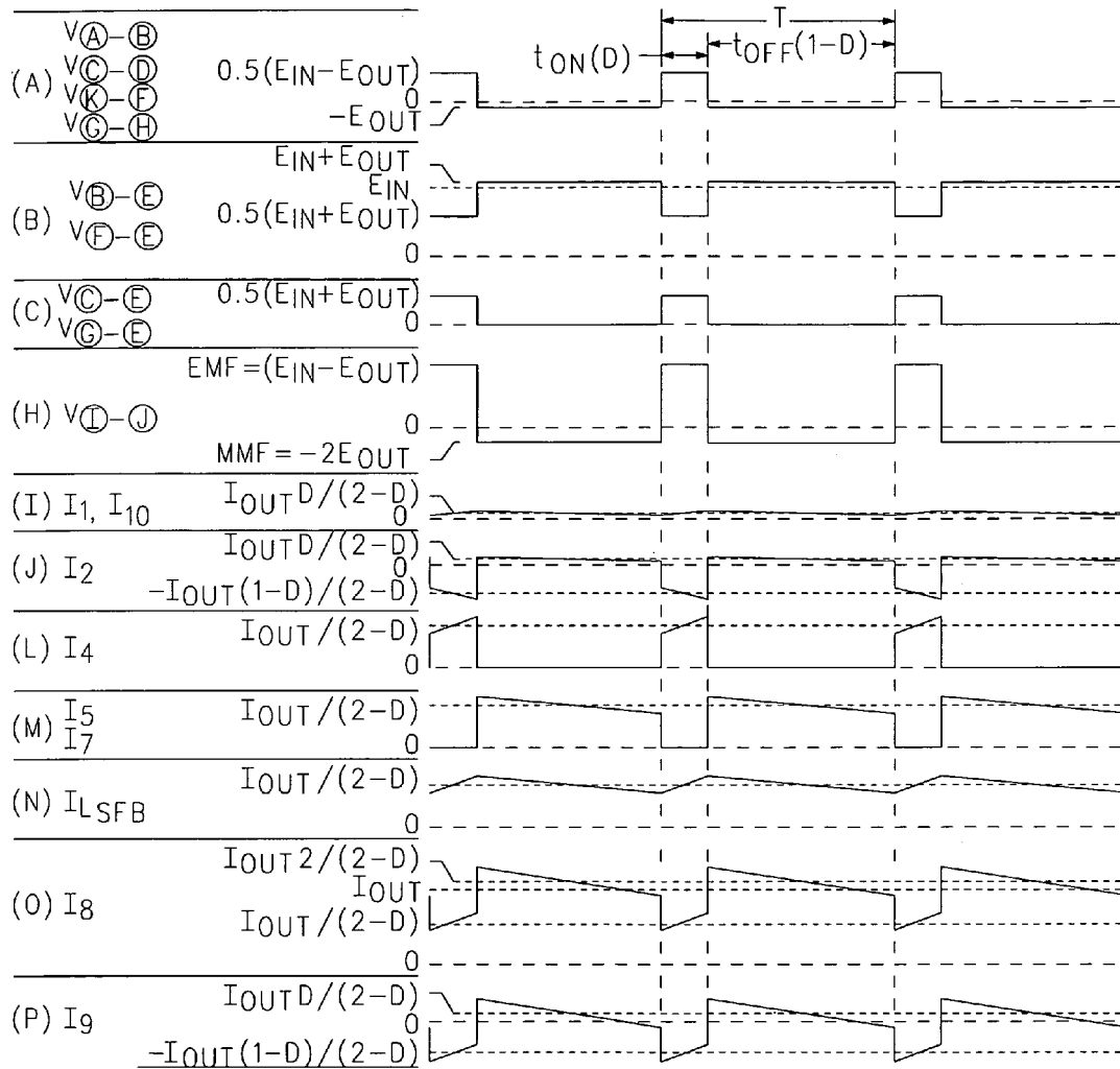
SEPIC FED BUCK (MC)
