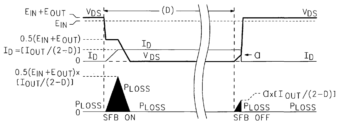
SEPIC FED BUCK
