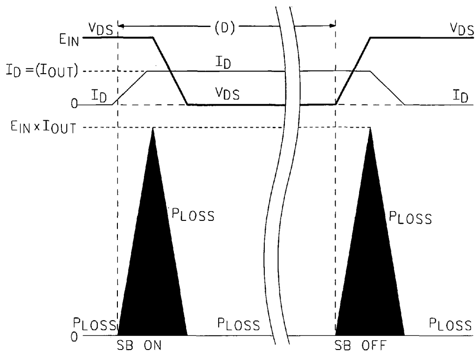
SYNCHRONOUS BUCK
