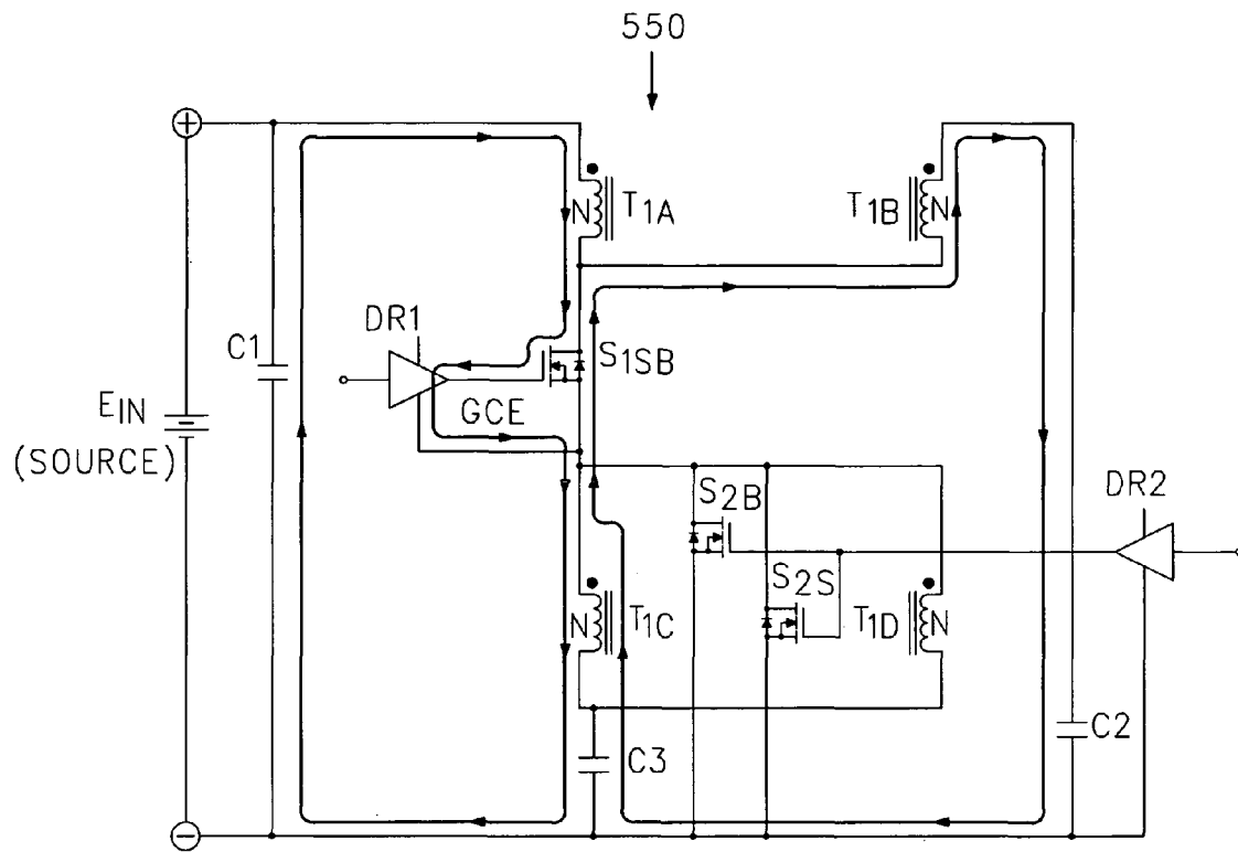
SEPIC FED BUCK (MC)
