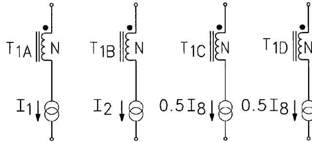
SEPIC FED BUCK (MC)
