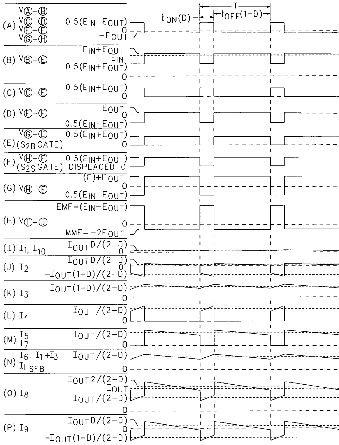
SEPIC FED BUCK (GC)
