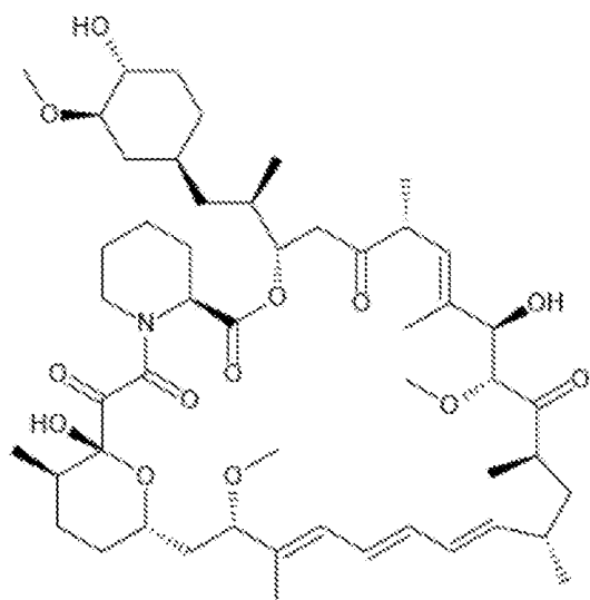
Sirolimus / Rapamycin
