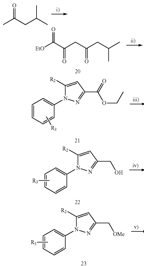
[Reaction Scheme 4]
