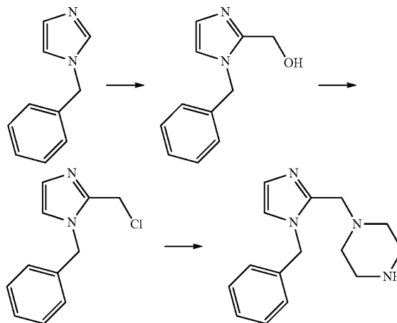
[Reaction Scheme 1]
