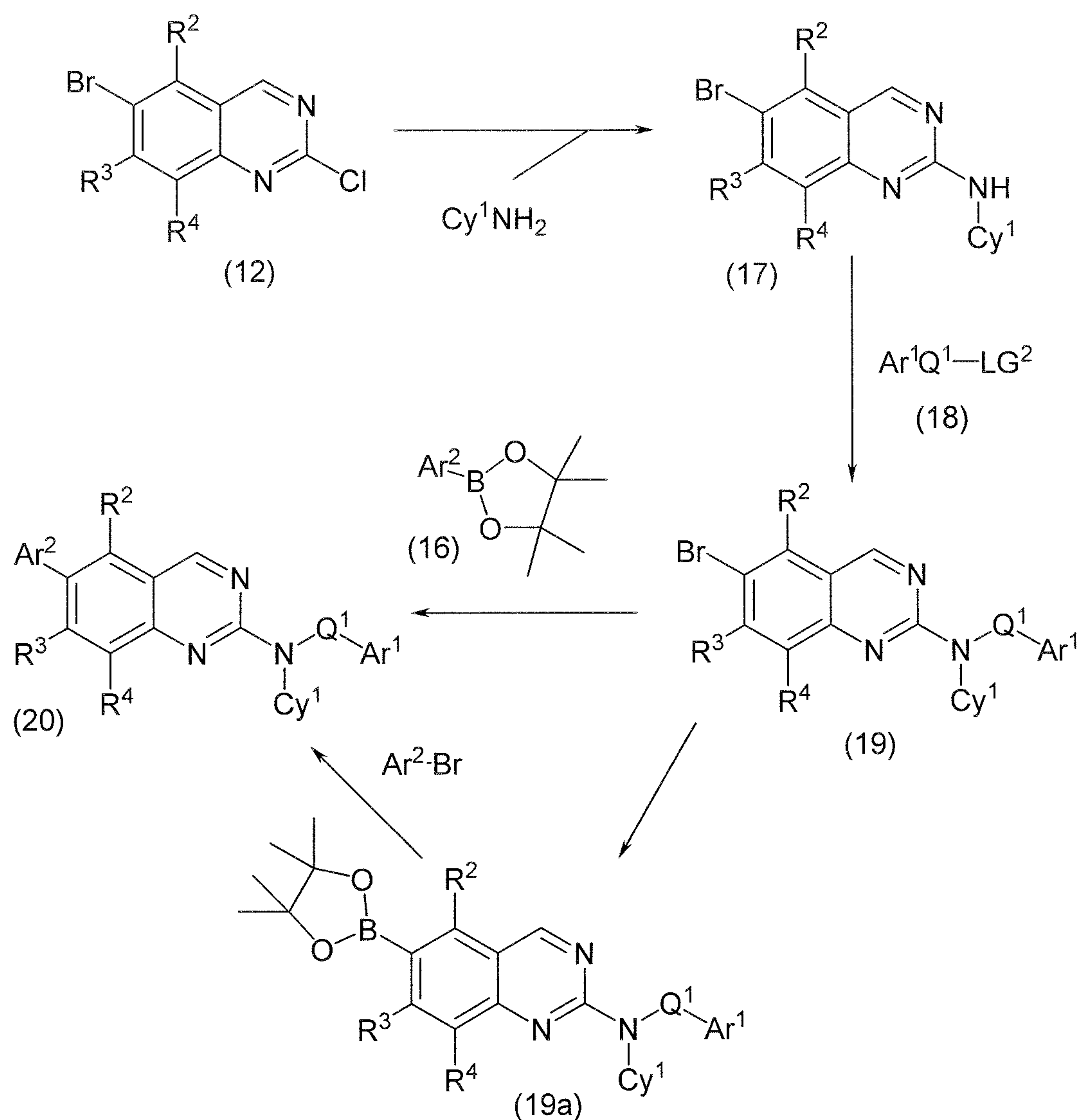
Scheme 2
