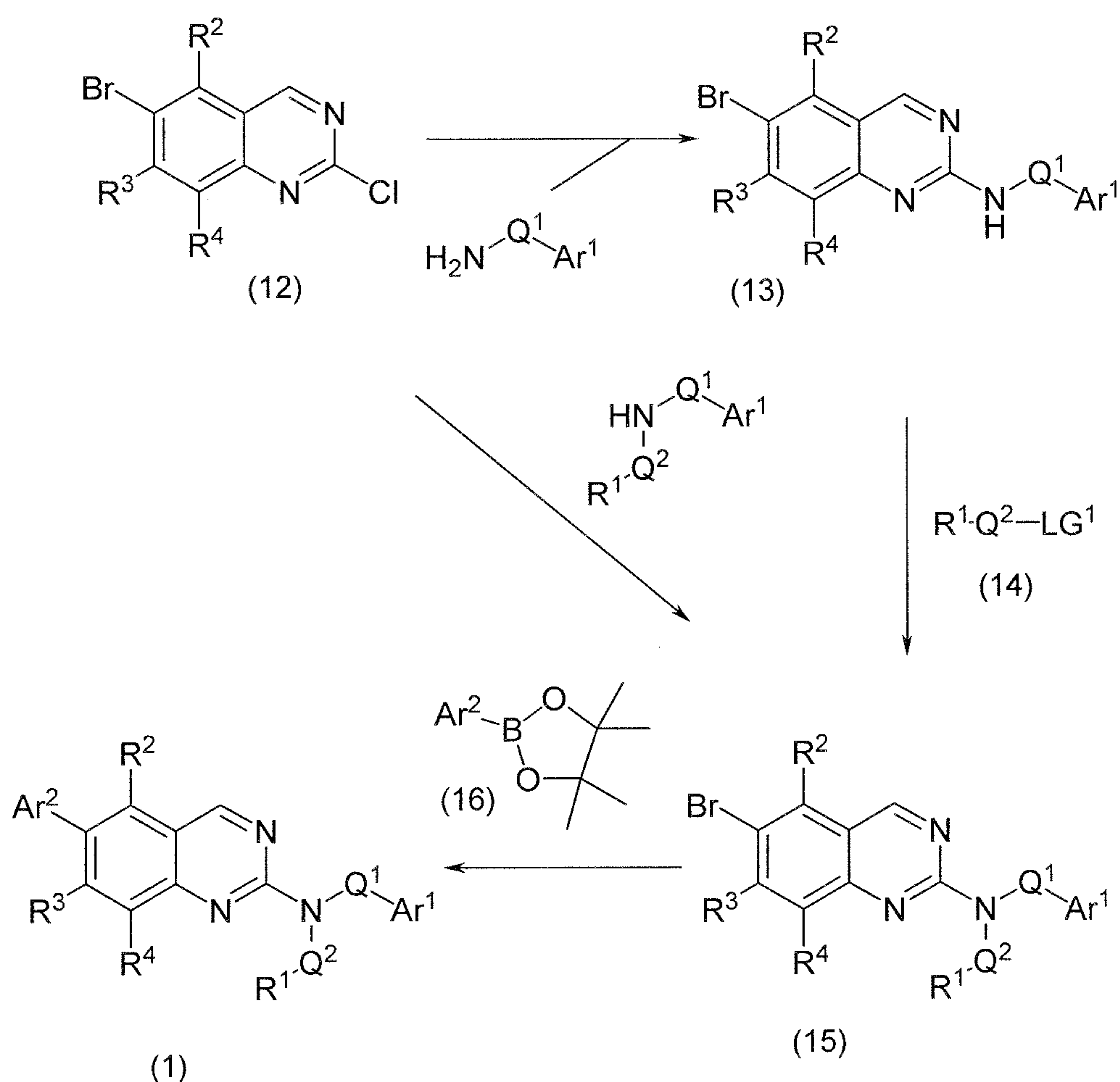
Scheme 1
