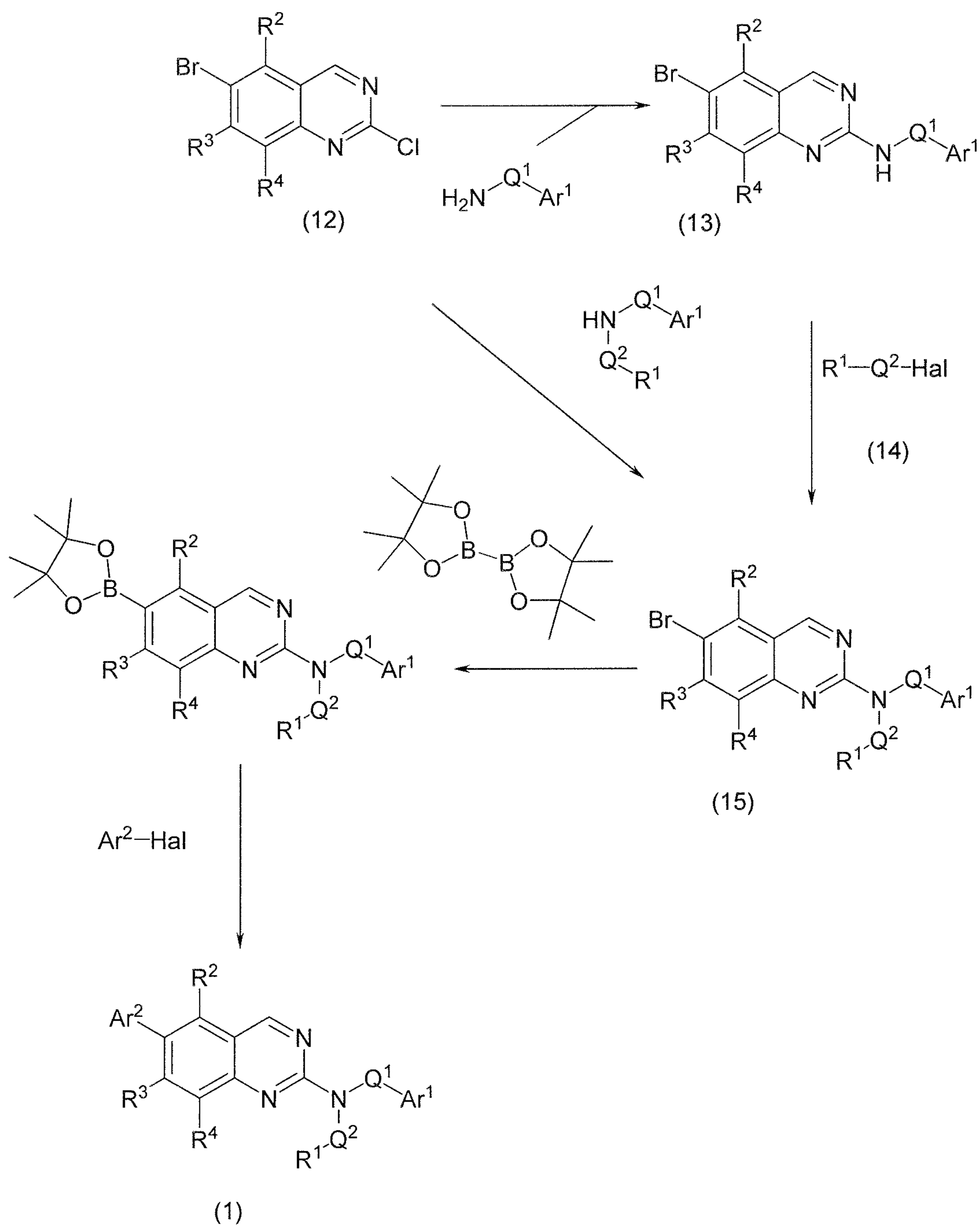
Scheme 3
