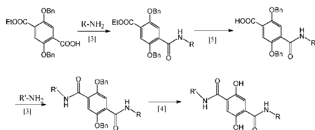
Scheme 7. Synthesis of Amides of type Ic with R ≠ R'
