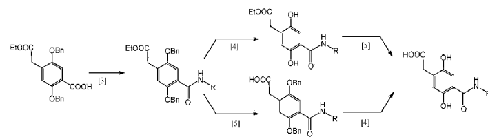
Scheme 14. Synthesis of Monoamides IIIa
