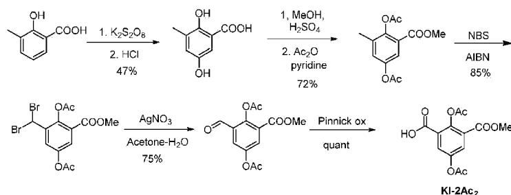
Scheme 9c: Synthesis of KI-2Ac 2
