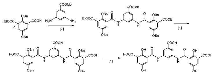
Scheme 11. Synthesis of Diamides of type IIb
