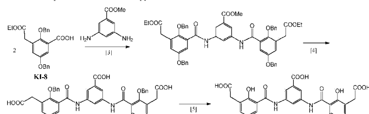
Scheme 15. Synthesis of Diamides of type IIIb
