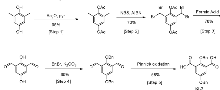
Scheme 9b: Alternative Synthesis of KI-7
