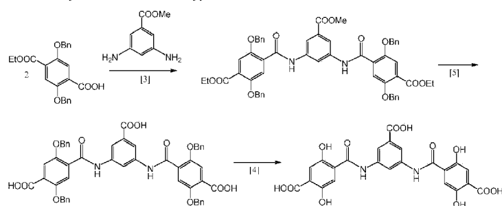
Scheme 5. Synthesis of Diamides of type Ib
