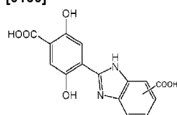
Scheme 8. Synthesis of compounds of type Id
