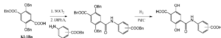
Scheme 4a. Synthesis of Monoamides Ia from KI-1Bn
