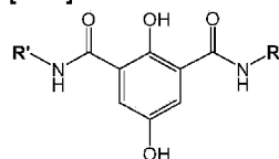
Scheme 12. Synthesis of Amides of type IIc with R = R'
