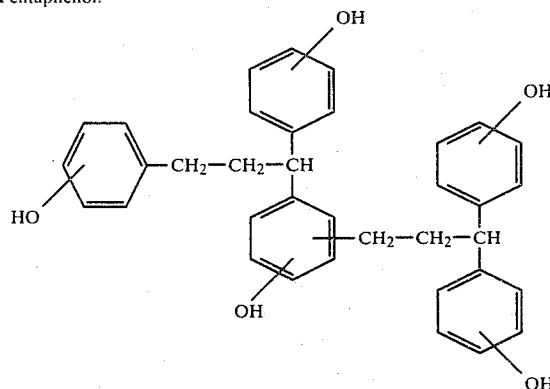
Pentaphenol:
