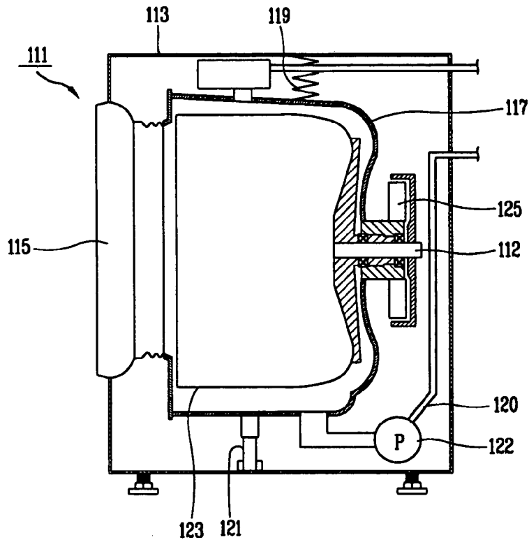
FIG. 3 CONVENTIONAL ART
