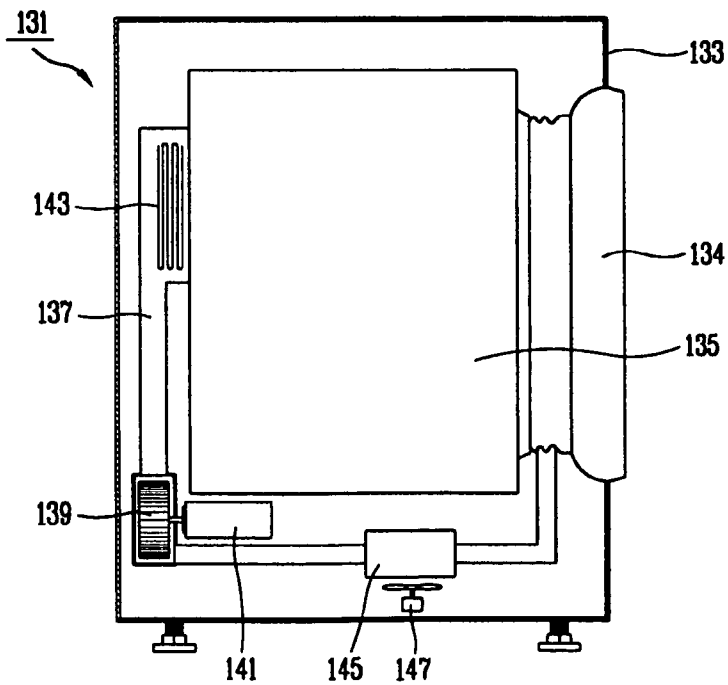
FIG. 3 CONVENTIONAL ART
