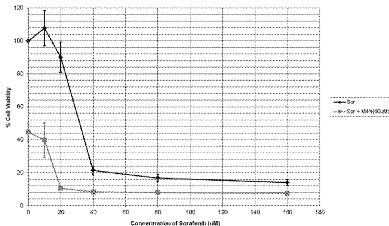
HepG2 Cells: 24 Hour Treatment with Sorafenib (Sor) and Sorafenib in Combination with a Constant Concentration of M4N (60 \mu M)
