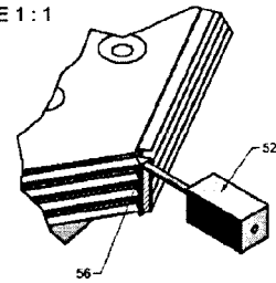
FIG. 7C HOT MELT DETAIL D SCALE 1 : 1
