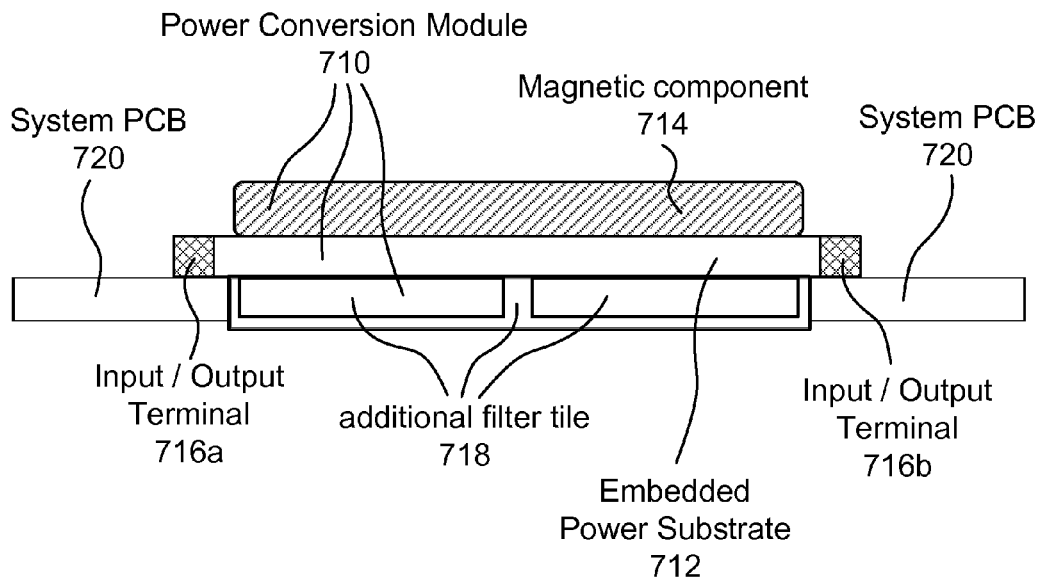
Cross Sectional View (System PCB with cavity)
