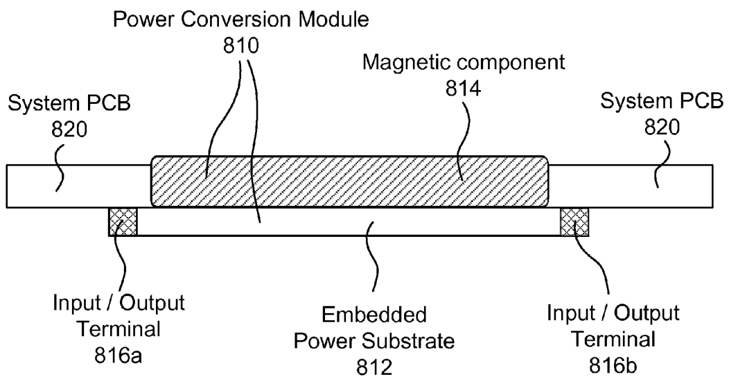
Cross Sectional View (System PCB with cavity)
