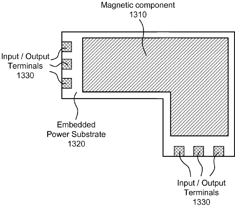
Top View
