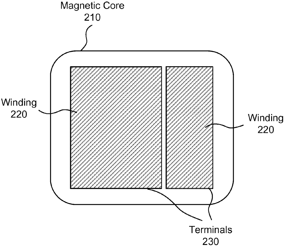
Bottom View (Magnetic Component)
