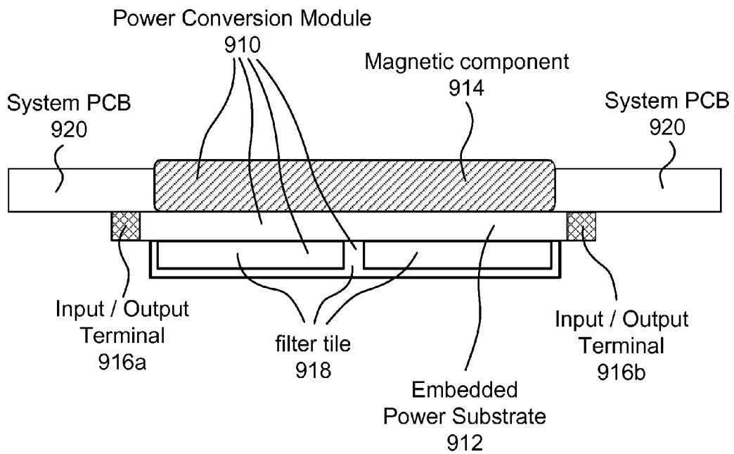
Cross Sectional View (System PCB with cavity)
