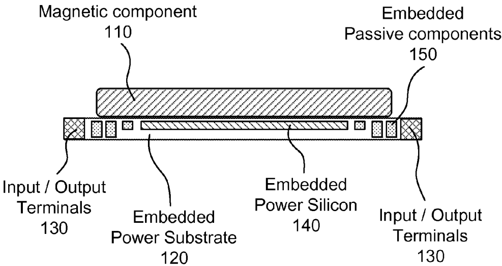
Cross Sectional View
