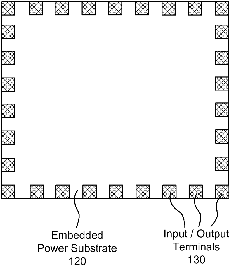
Bottom View
