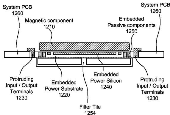
Cross Sectional View (Module with filter tile and protruding input/output terminals connected to system PCB)
