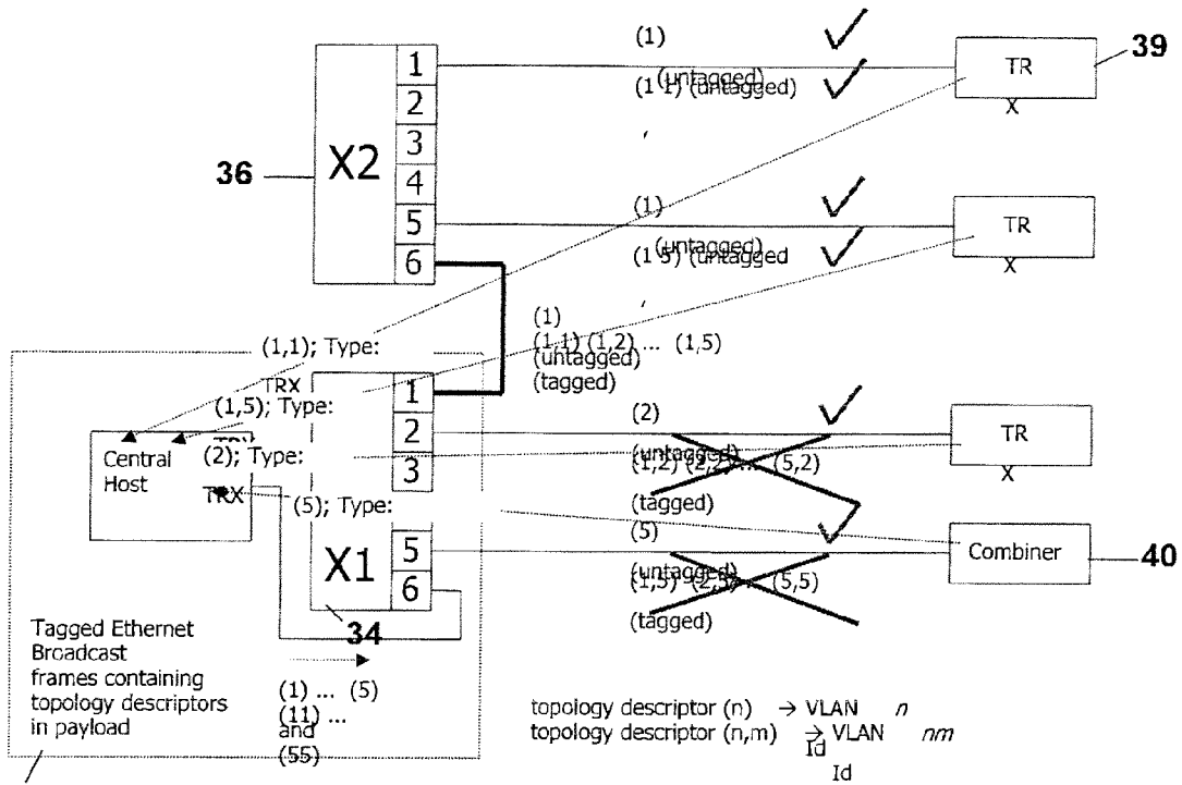
Fig. 9 VLAN-based implementation
