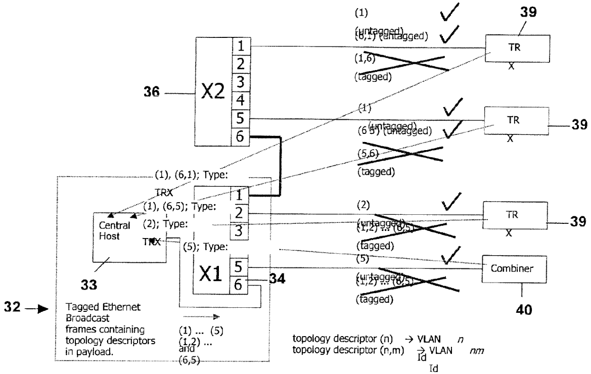
Fig. 5 VLAN-based implementation
