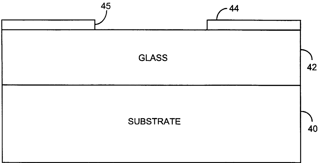
SPIN ON GLASS AND METALIZATION
