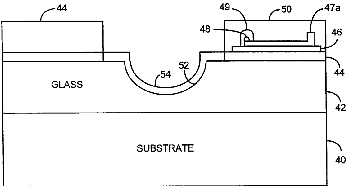
REFLECTOR METALIZATION FIG. 2d
