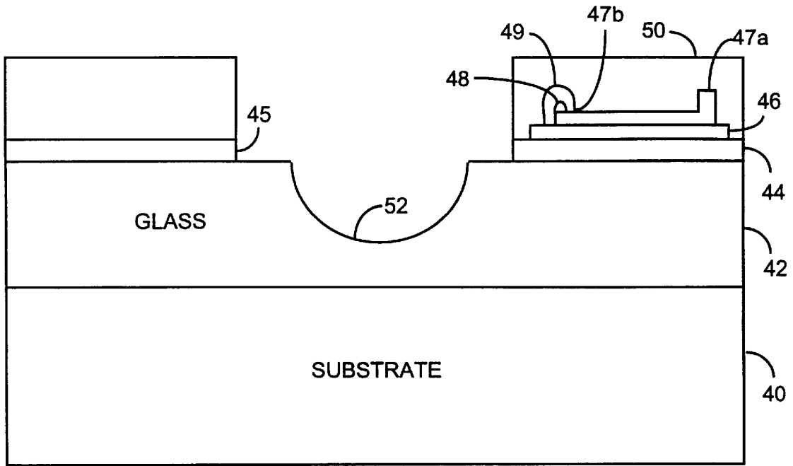
RECEIVER APERTURE FORMATION FIG. 2c
