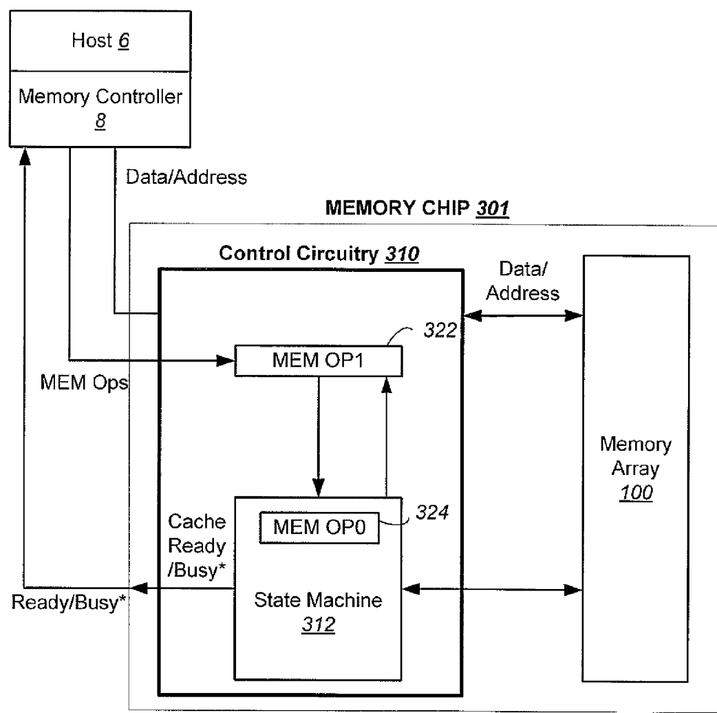
CONVENTIONAL CACHED MEMORY OPERATION
