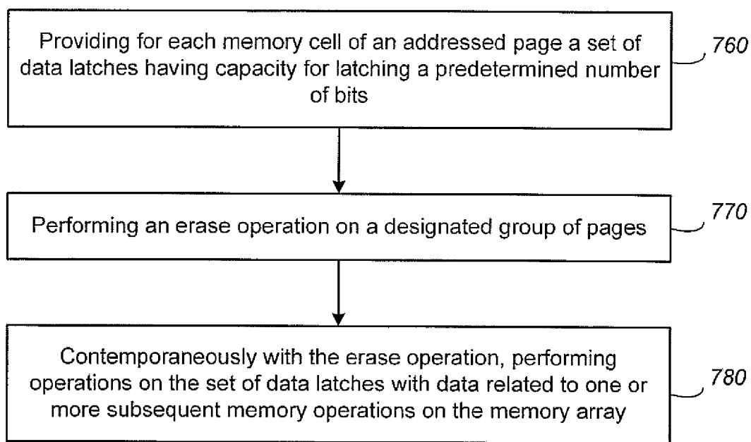
Cache Operation During Erase Operation
