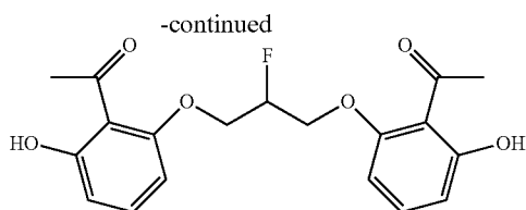
1,3-Bis(2-acetyl-3-hydroxyphenoxy)-2-fluoropropane
