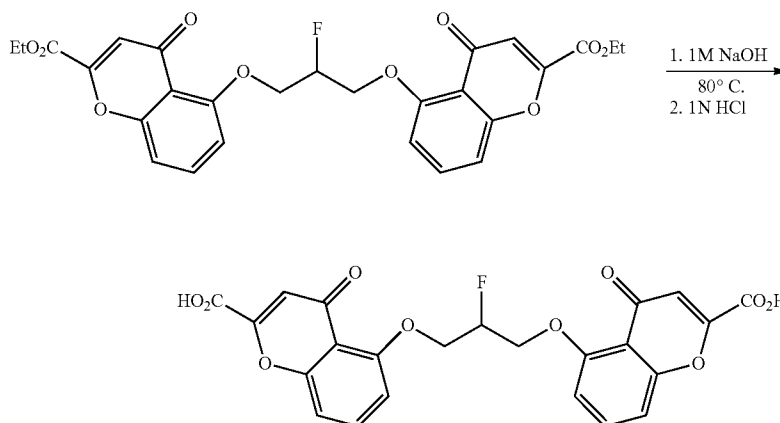
5,5'-(2-fluoropropane-1,3-diyl)bis(oxy)bis(4-oxo-4H-chromene-2-carboxylic acid)
