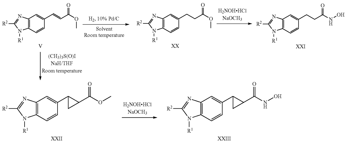
Scheme IV
