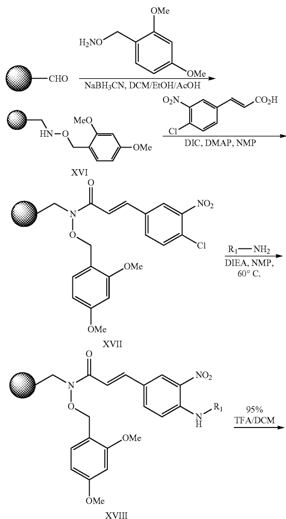
Scheme III
