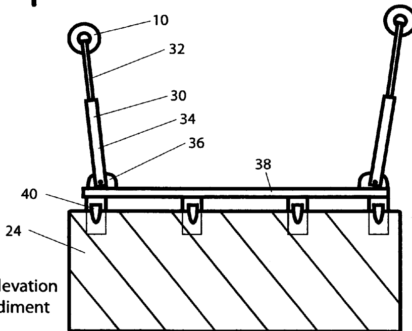
Figure 4: Front Elevation of Third Embodiment
